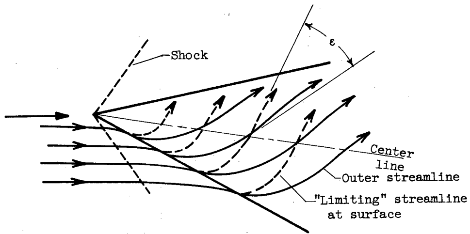
Figure 2. - Streamline patterns illustrating "secondary flow."
