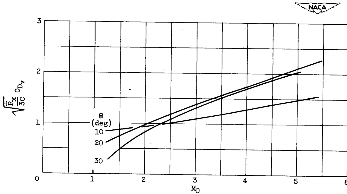
Figure 13. - Coefficient of viscous drag.
