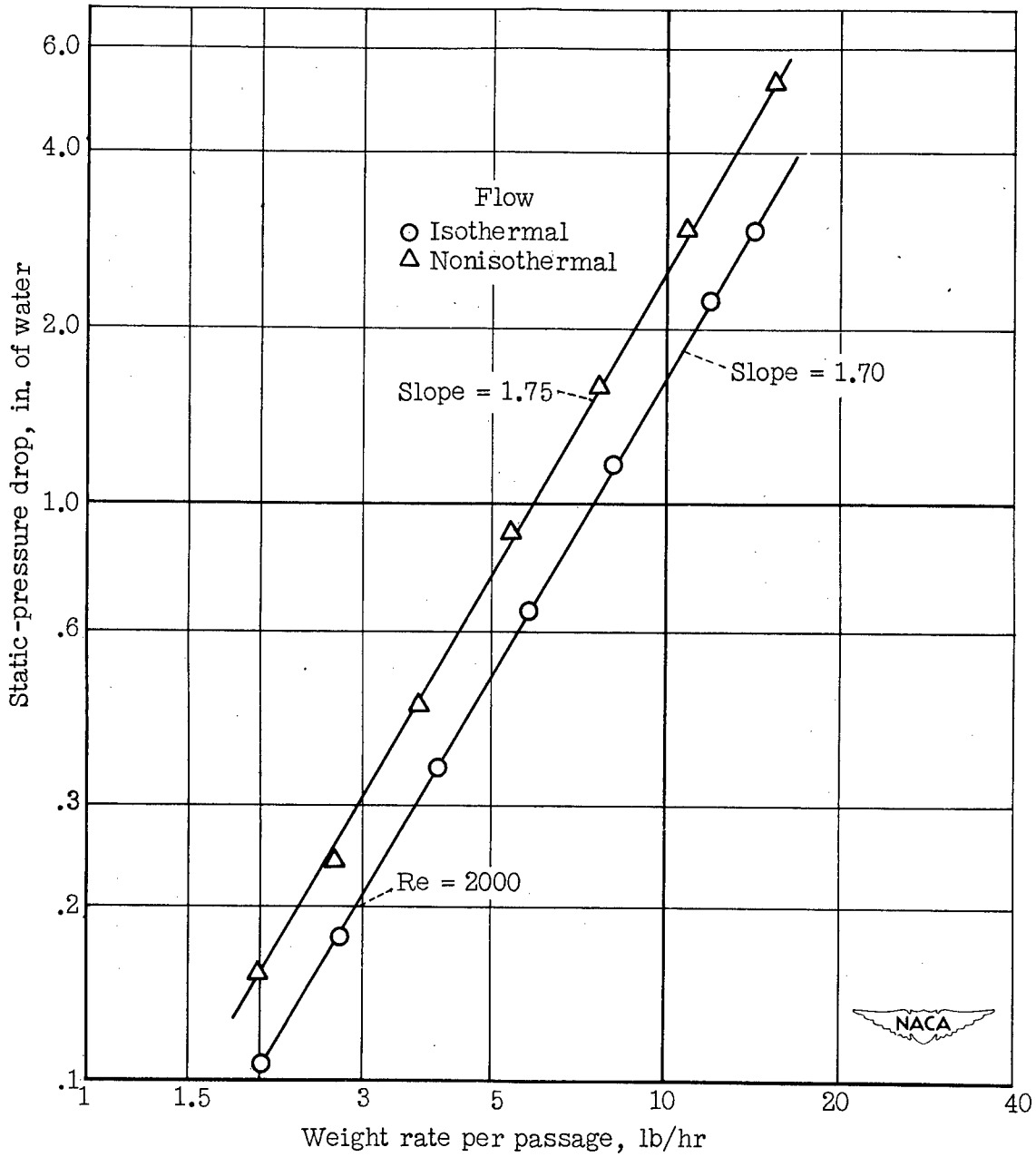
(b) Trapezoidal ducts.
