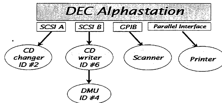
Fig. 2 — AV-8B Map-II SCSI and GRIP connections
