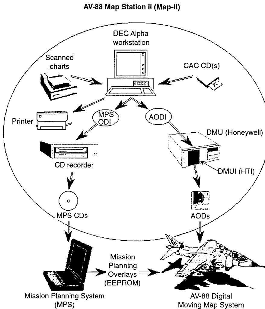
Fig. 1 — AV-8B Map-II hardware components
