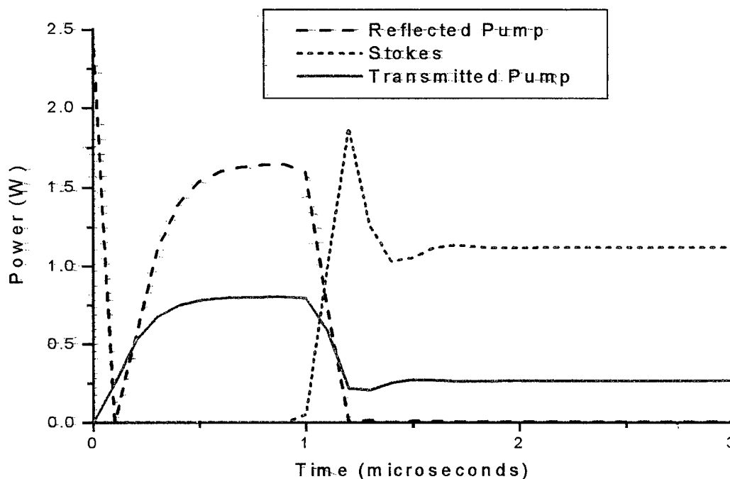
Figure 8. Time dependent behavior of a cw Raman laser. The time evolution of the pump reflected from the high-finesse cavity, the transmitted pump, and the Stokes is shown. In this case, a 2.5 W pump laser with a wavelength of 1.064 \mu\text{m} is assumed with a methane cw Raman laser.
