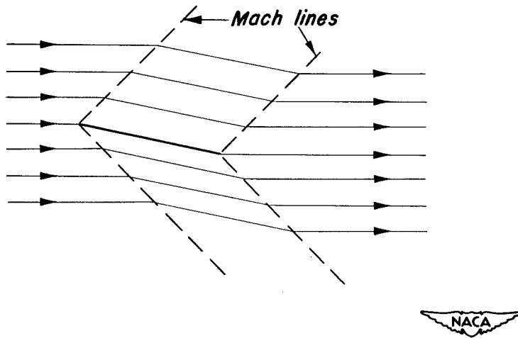
Figure 8.—Flow field produced by wing alone.
