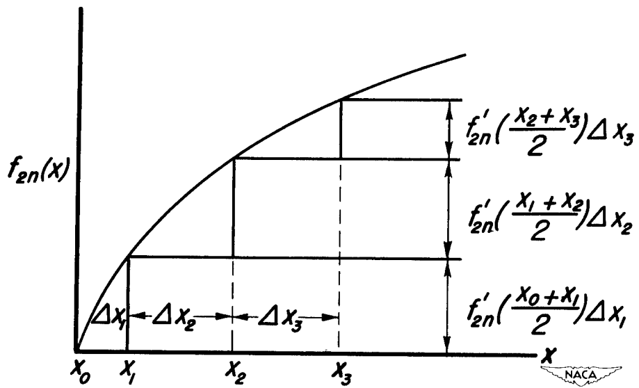
Figure 25.— Approximation of velocity amplitude function by series of step functions.
