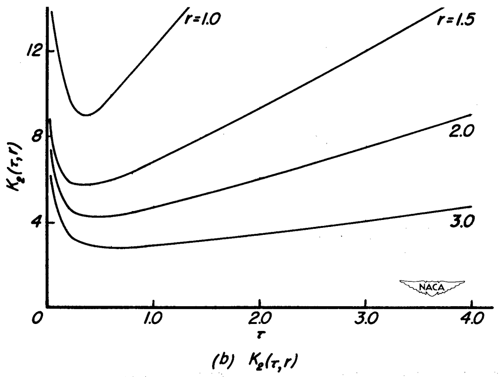
Figure 13. - Curves of K_0(\tau, r) and K_2(\tau, r) .
