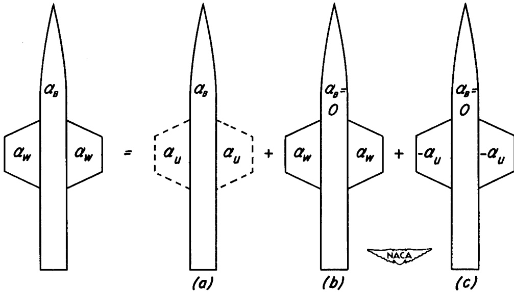
Figure 2.- Decomposition of wing-body combination into component configurations.
