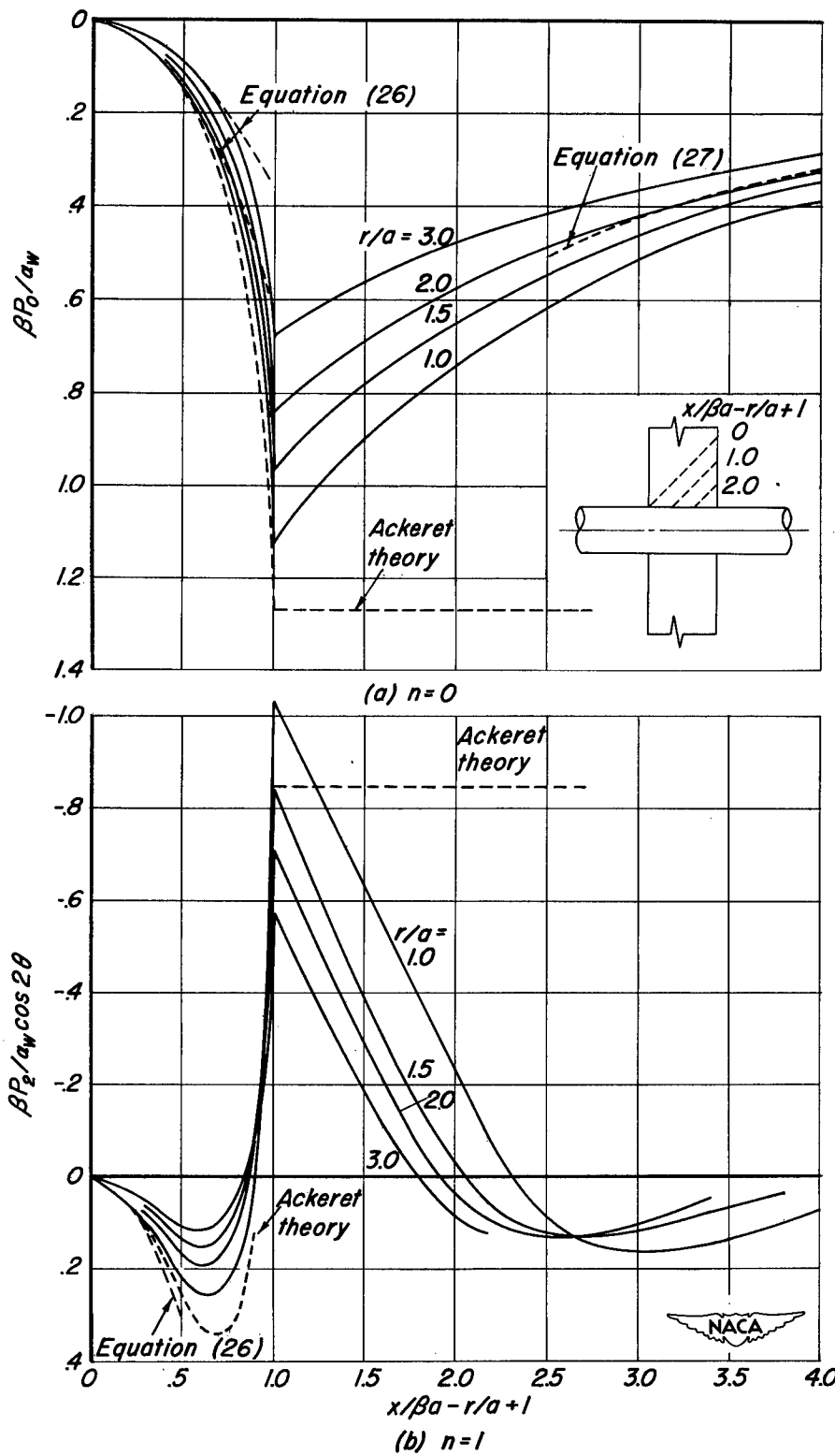
Figure 15.- Interference pressure distributions of various Fourier components.
