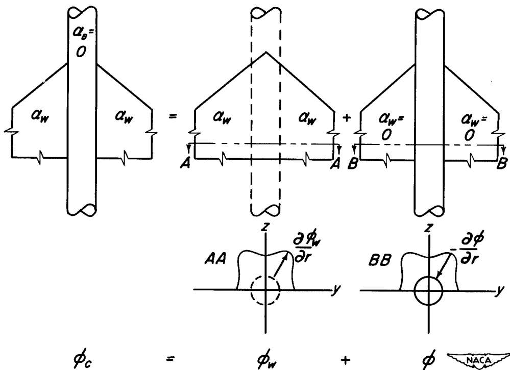
Figure 3.- Wing-body combination as the sum of wing alone plus interference combination.
