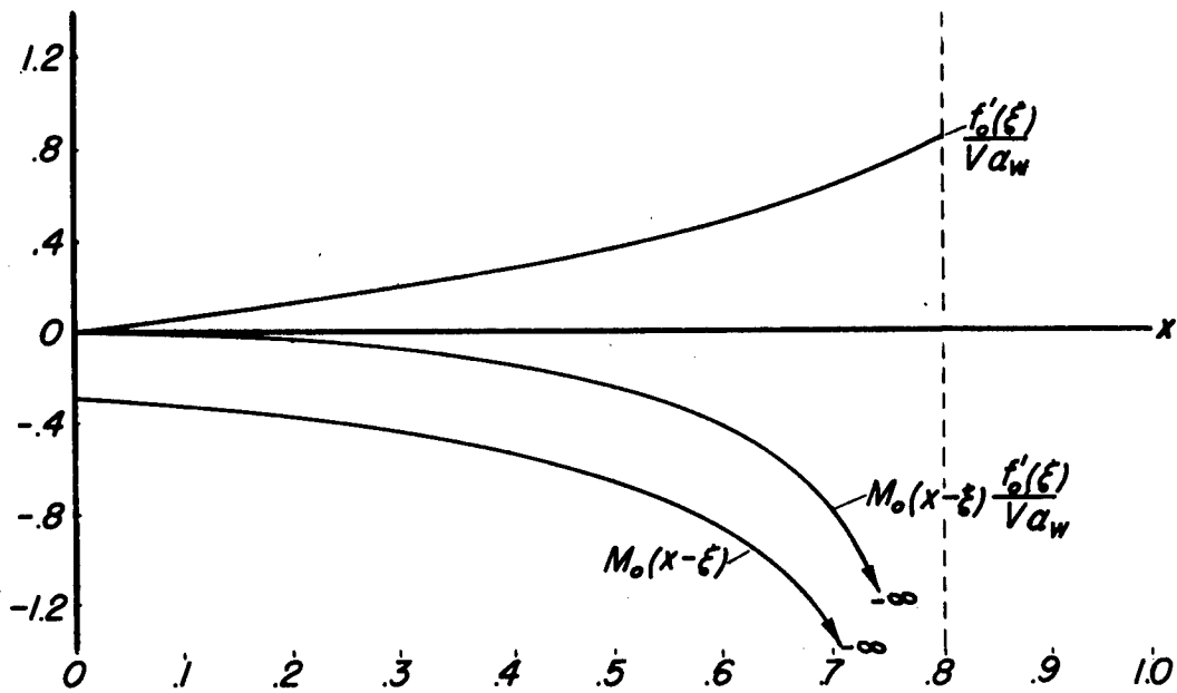
(a) x < 1
