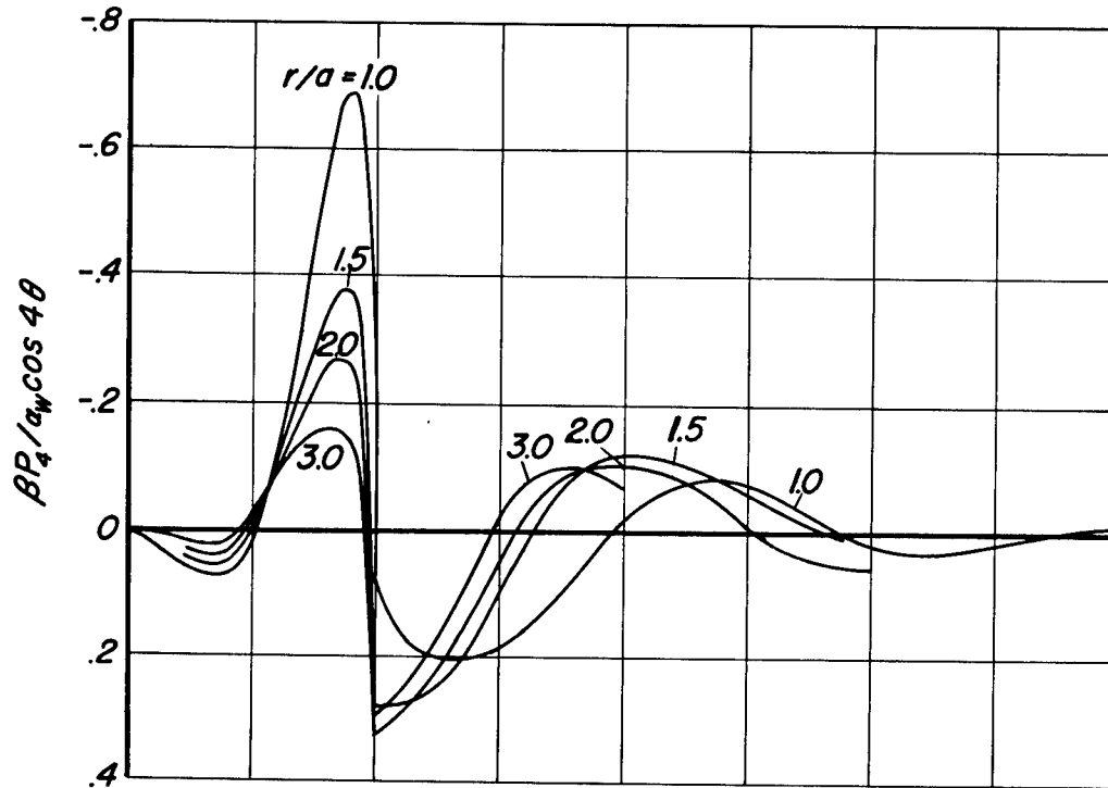
(c) n = 2
