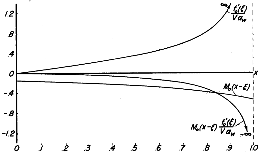
(b) x > 1
