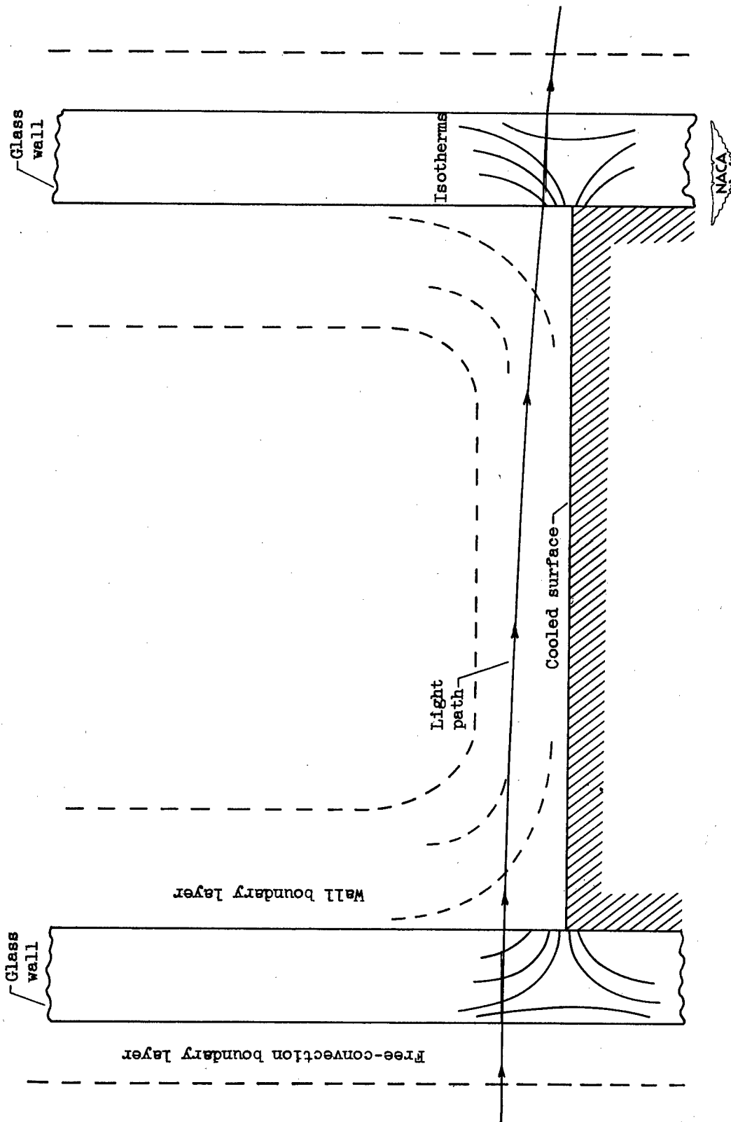
Figure 1. - Schematic diagram of path of light ray through two-dimensional test section.
