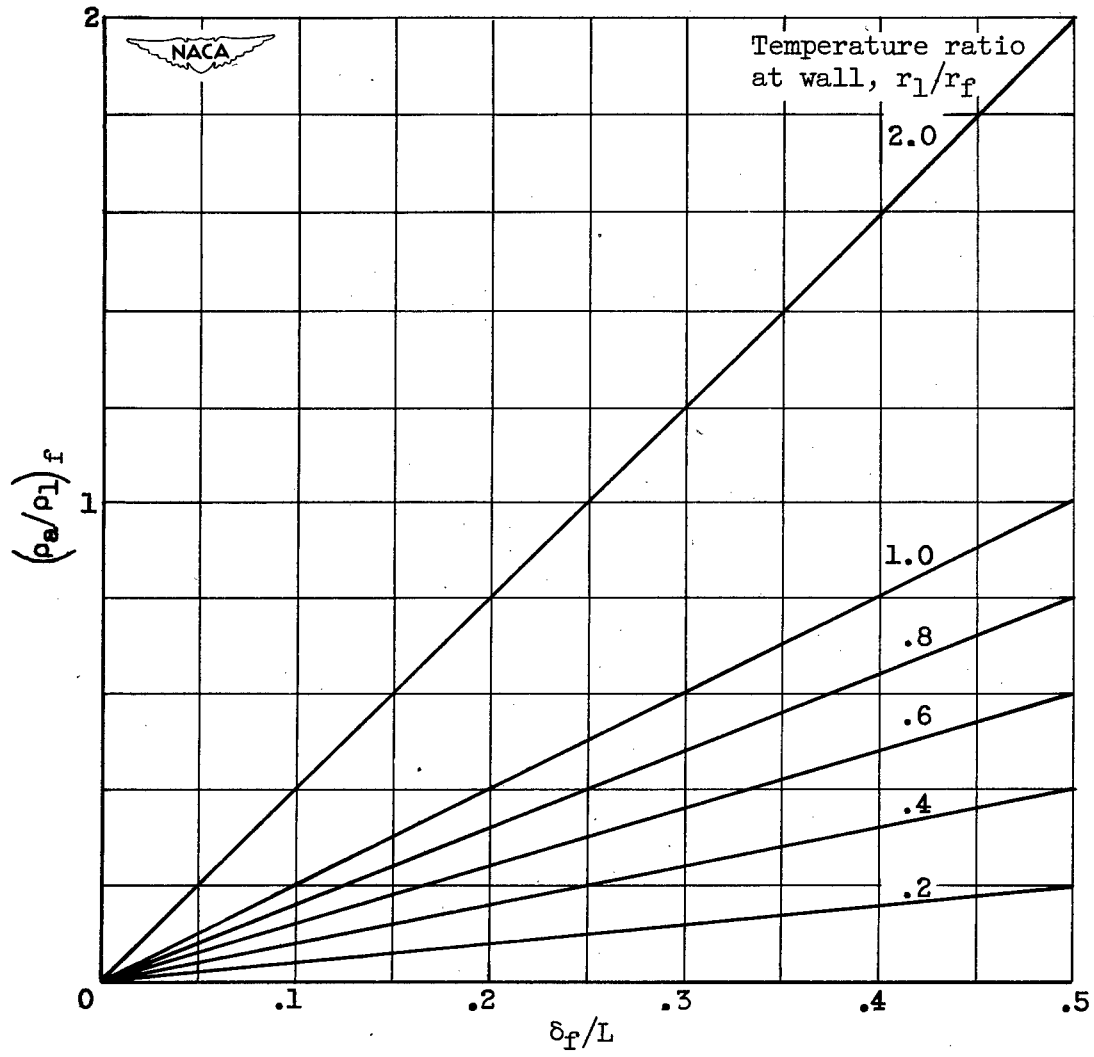
Figure 7. - Effect of wall boundary layer on (\rho_a/\rho_l)_f .
