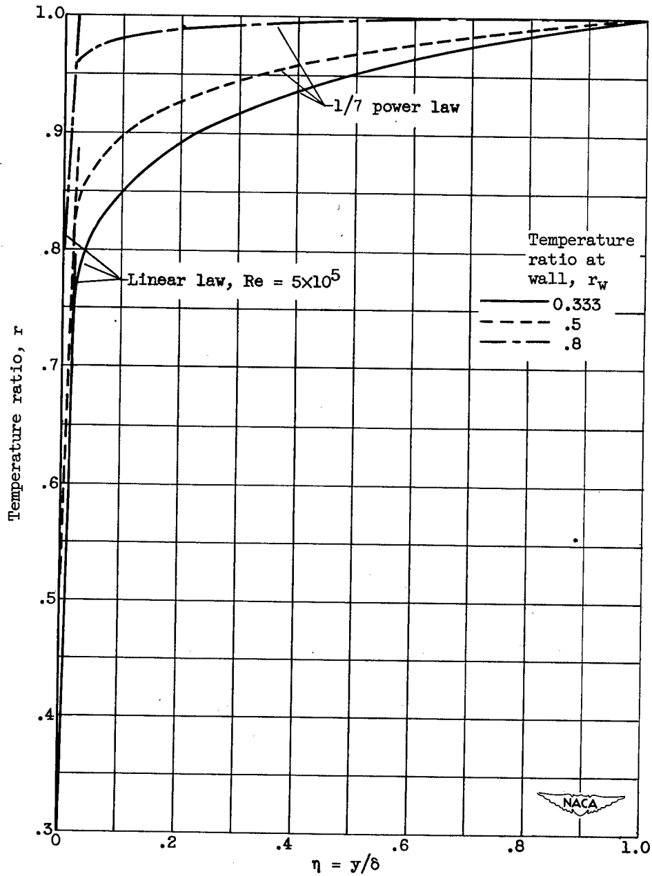
(b) Turbulent boundary layer; \gamma = 1.4 .
