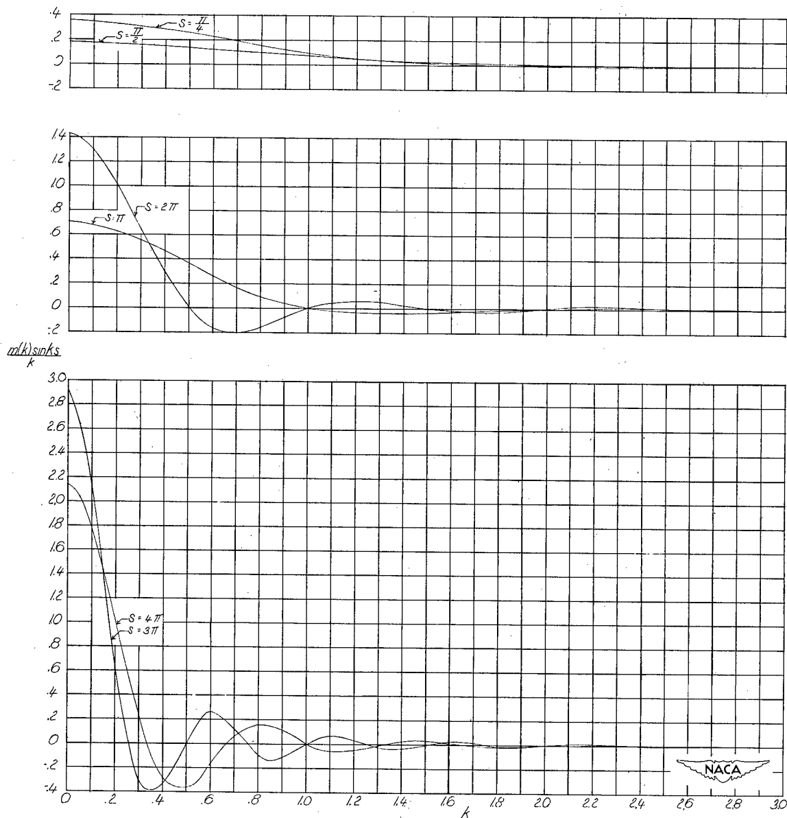
Figure 7.- Plots of the integrand in equation (21) for determining the indicial moment m_l(s) about the quarter chord at M = 0.7 .
