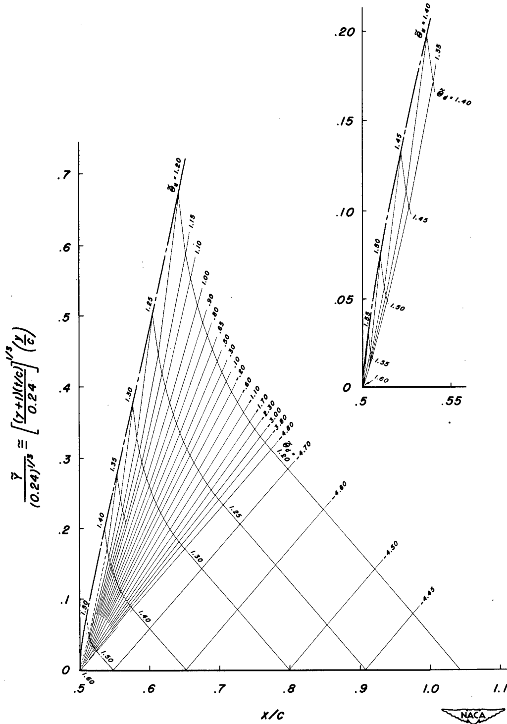
Figure 4.- Mach net over rear of airfoil for \bar{\theta}_w = 1.6 ( \xi_o = 0.921 ).
