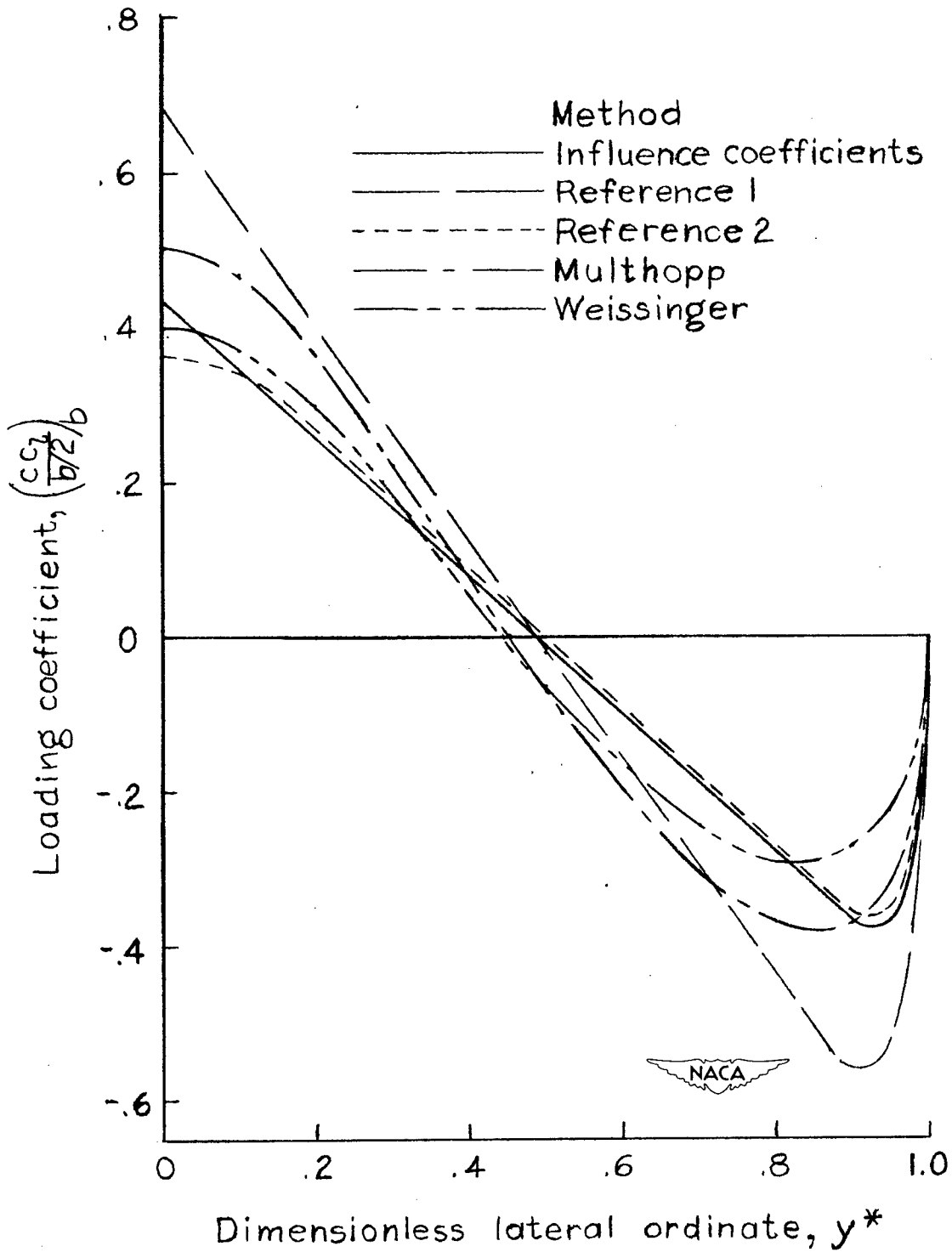
Figure 4.- Basic lift distribution of rectangular wing of aspect ratio 5 with unit linear symmetric twist in incompressible flow.
