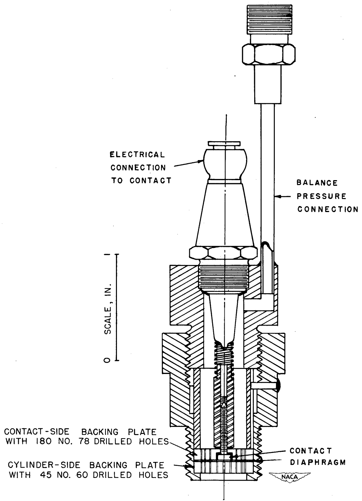
Figure 6.- Construction of pickup unit of M.I.T. balanced-pressure indicator.
