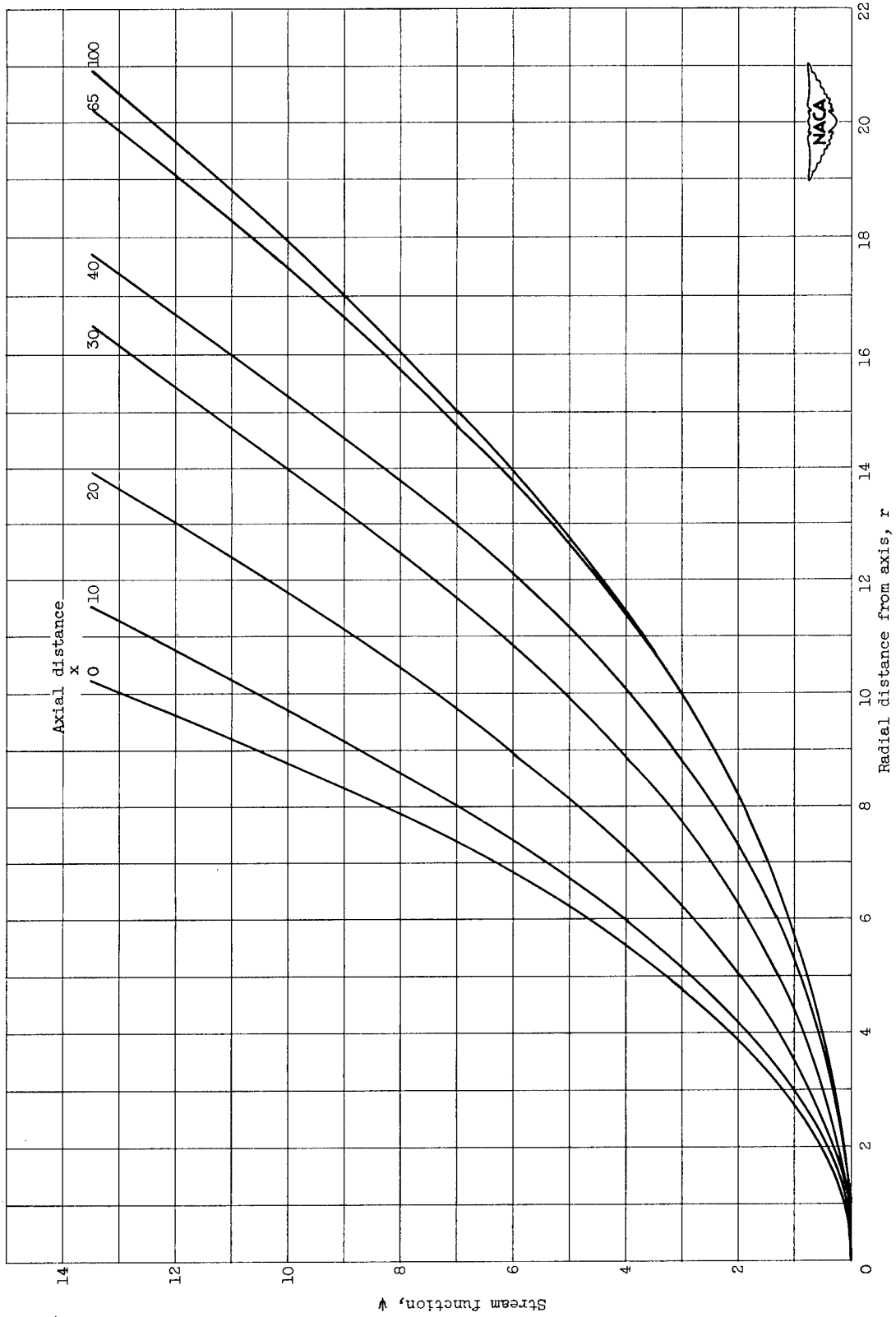
Figure 1. - Variation of stream function with position for Mach number of 2.98.
