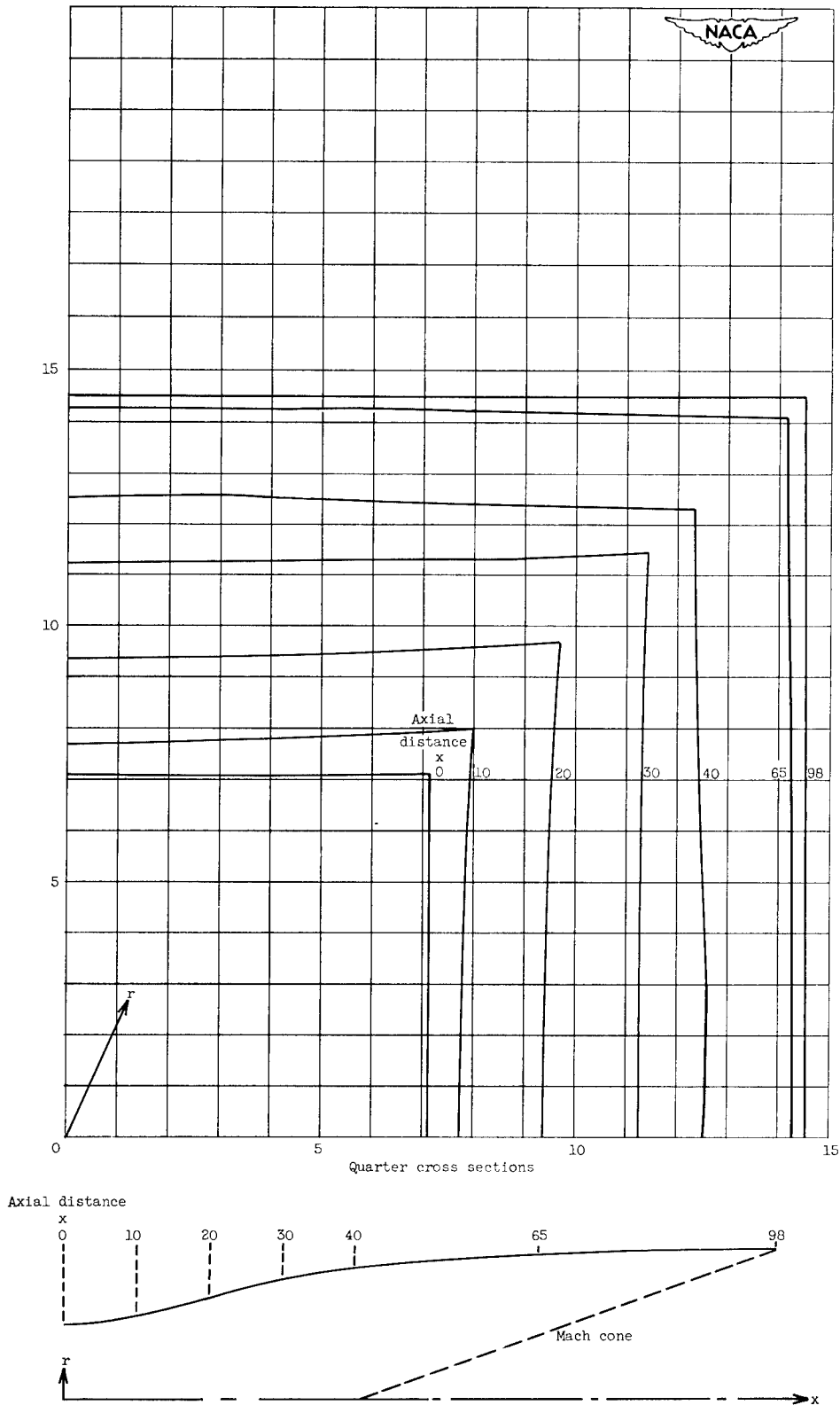
Figure 3. - Square nozzle for Mach number of 2.96.
