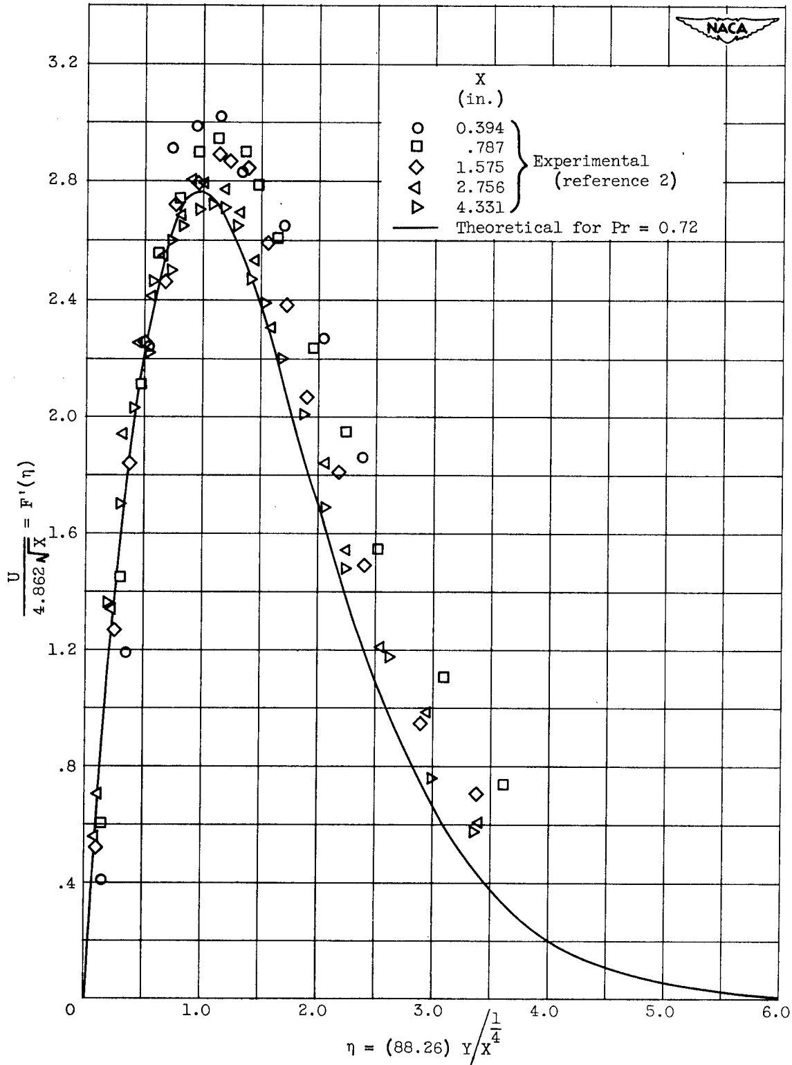
Figure 3. - Comparison of small plate experimental and theoretical velocity distributions for Prandtl number of 0.72.
