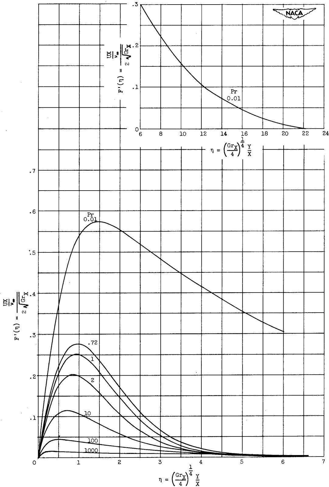
Figure 1. - Dimensionless velocity distributions for various Prandtl numbers.
