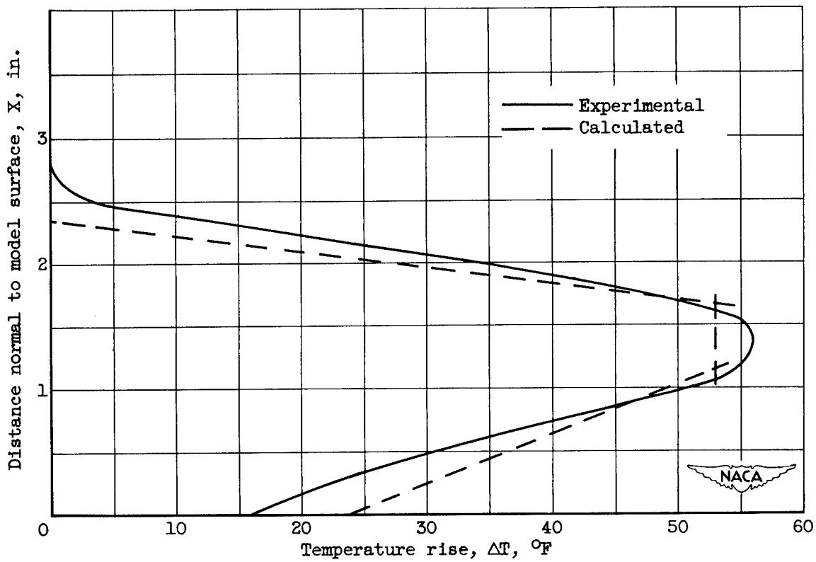
Figure 20. - Comparison of calculated and experimental profile for jet operating at pressure ratio less than choking. Jet pressure ratio, 1.33; orifice diameter, 0.625 inch; jet total temperature, 860° R; tunnel-air velocity, 290 feet per second; rake station, 4.81 inches.
