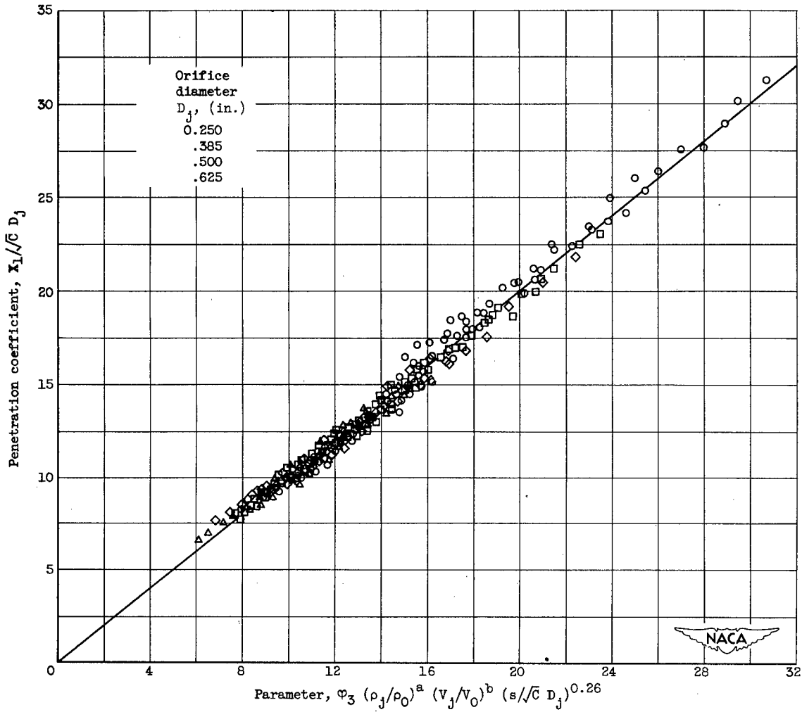
Figure 10. - Variation of penetration coefficient X_1/\sqrt{C} D_j with parameter \varphi_3 (\rho_j/\rho_0)^a (V_j/V_0)^b (s/\sqrt{C} D_j)^{0.26} for various temperature ratios.
