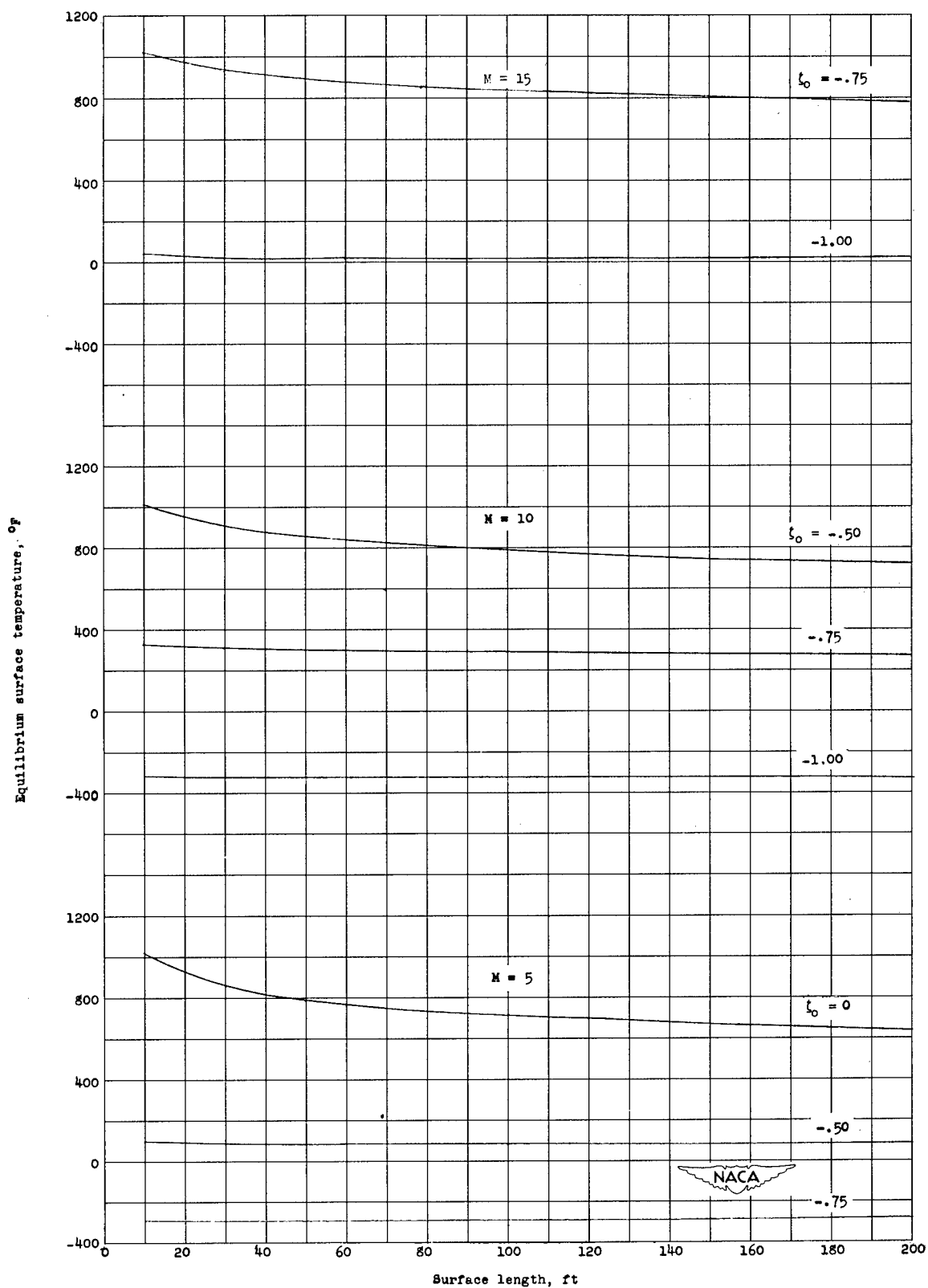
Figure 5.- Equilibrium surface temperature for various amounts of blowing.
