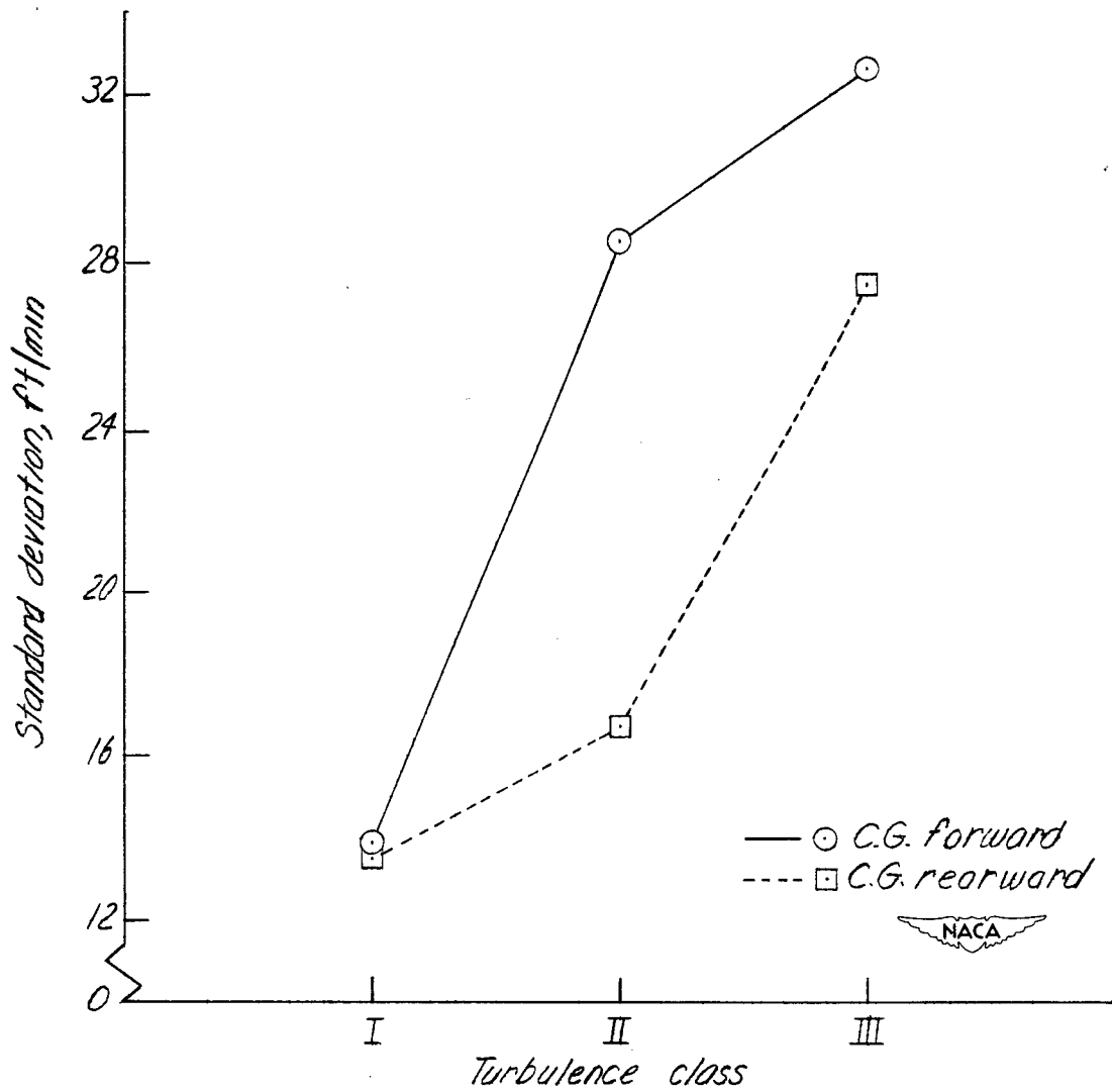
Figure 2.- Standard deviation of the rate of climb as a function of turbulence class.
