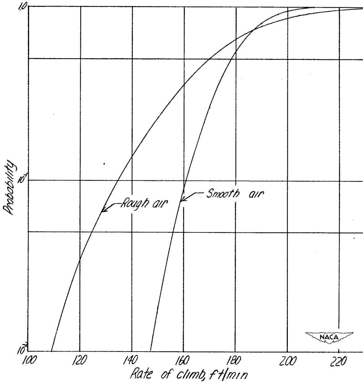
(b) Rearward center of gravity.
