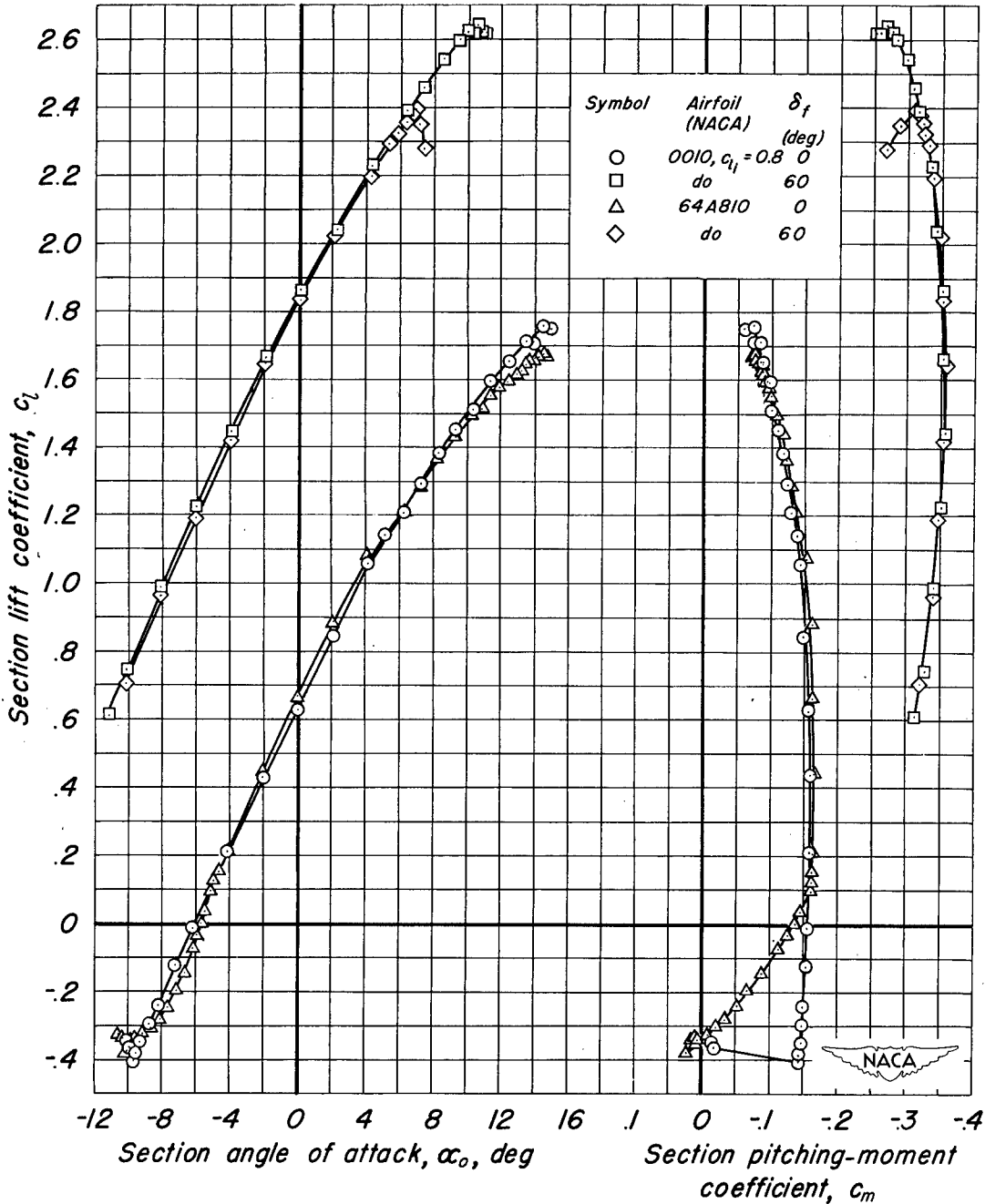
(a) Smooth airfoils; Reynolds number 3.7 \times 10^6 .
