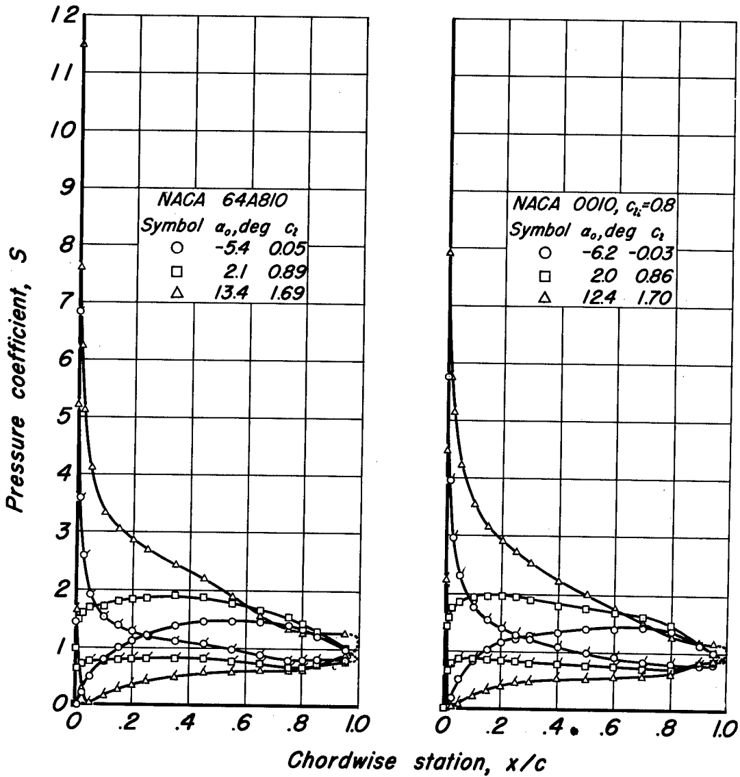
(b) Airfoils cambered for a design lift coefficient of 0.8.
