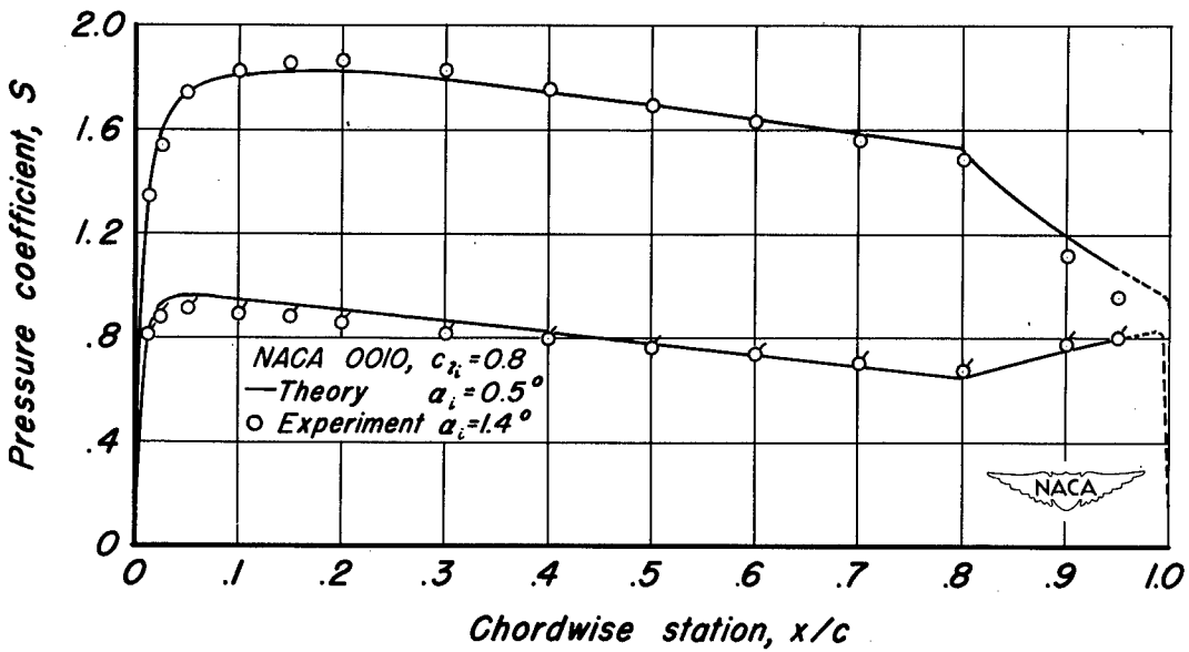
(b) Airfoils cambered for a design lift coefficient of 0.8.
