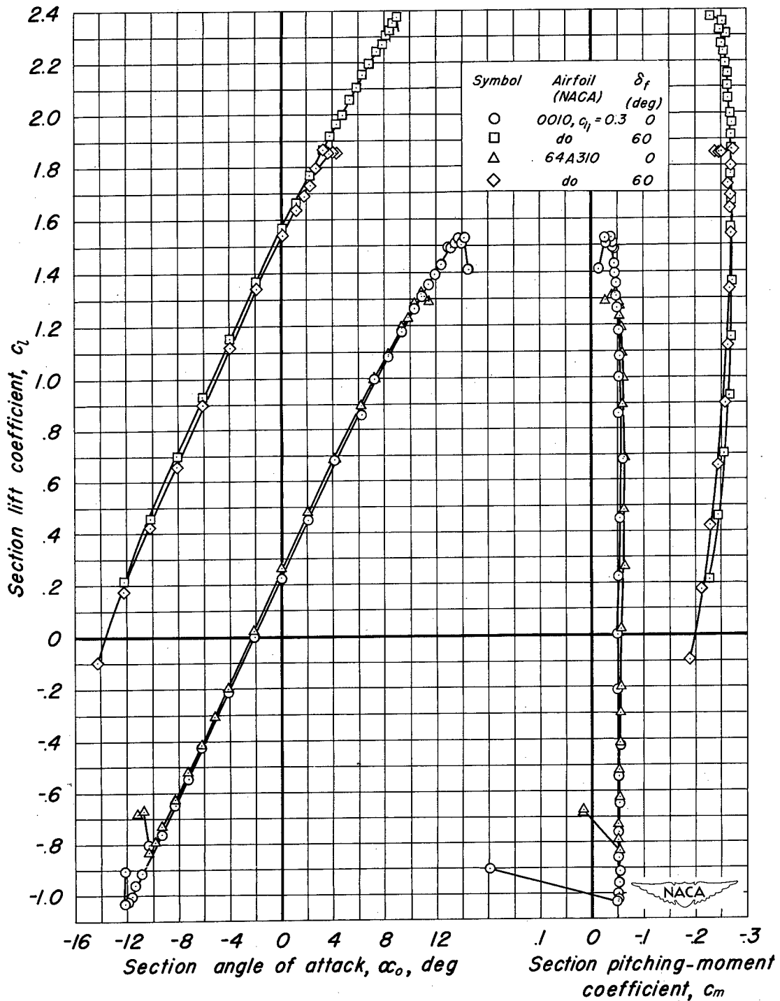
Figure 2.—Section lift and pitching-moment characteristics of the two models cambered for a design lift coefficient of 0.3.
