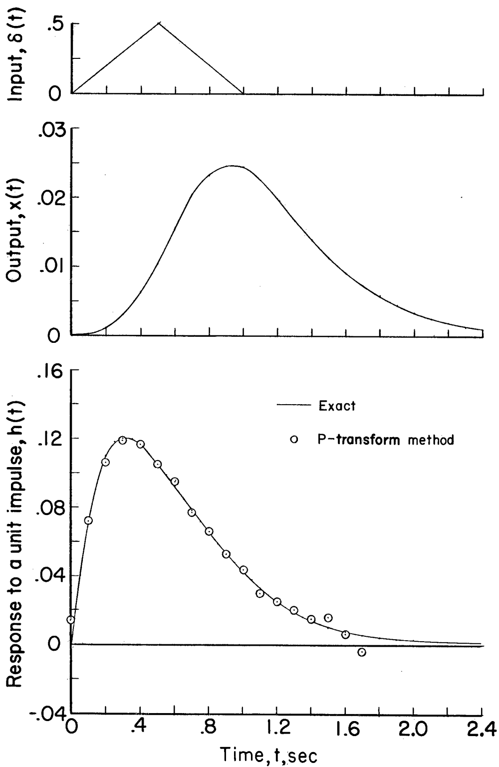
Figure 7.- Time response to a unit impulse obtained from the P-transform method compared to the exact values for the second-order system.
