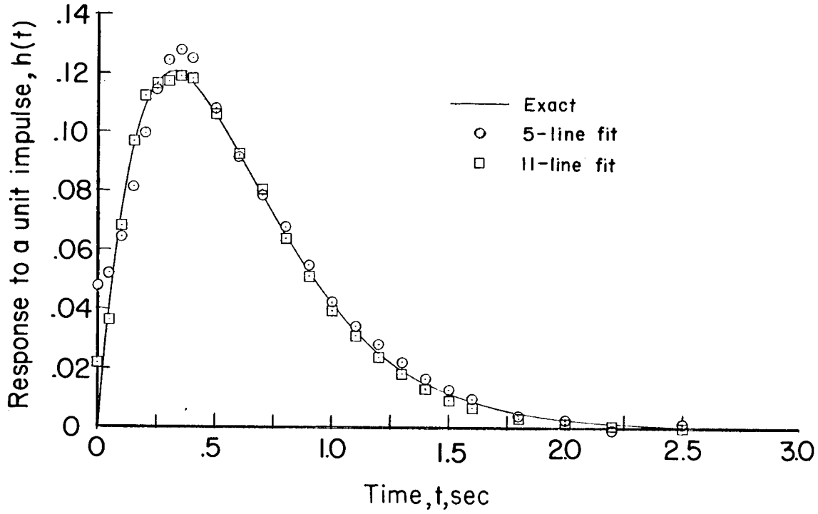
Figure 2.- Time response to a unit impulse obtained from Floyd's method compared to the exact values for the second-order system.
