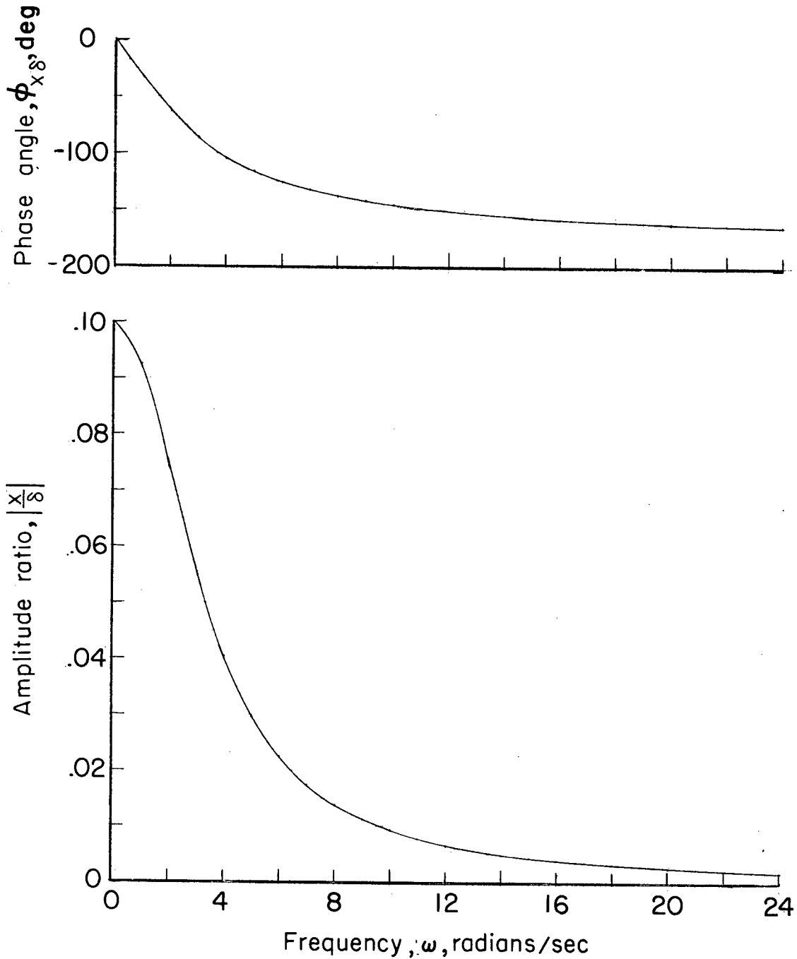
Figure 1.- Frequency response of second-order system. \frac{x}{s}(s) = \frac{1}{s^2 + 6s + 10} .
