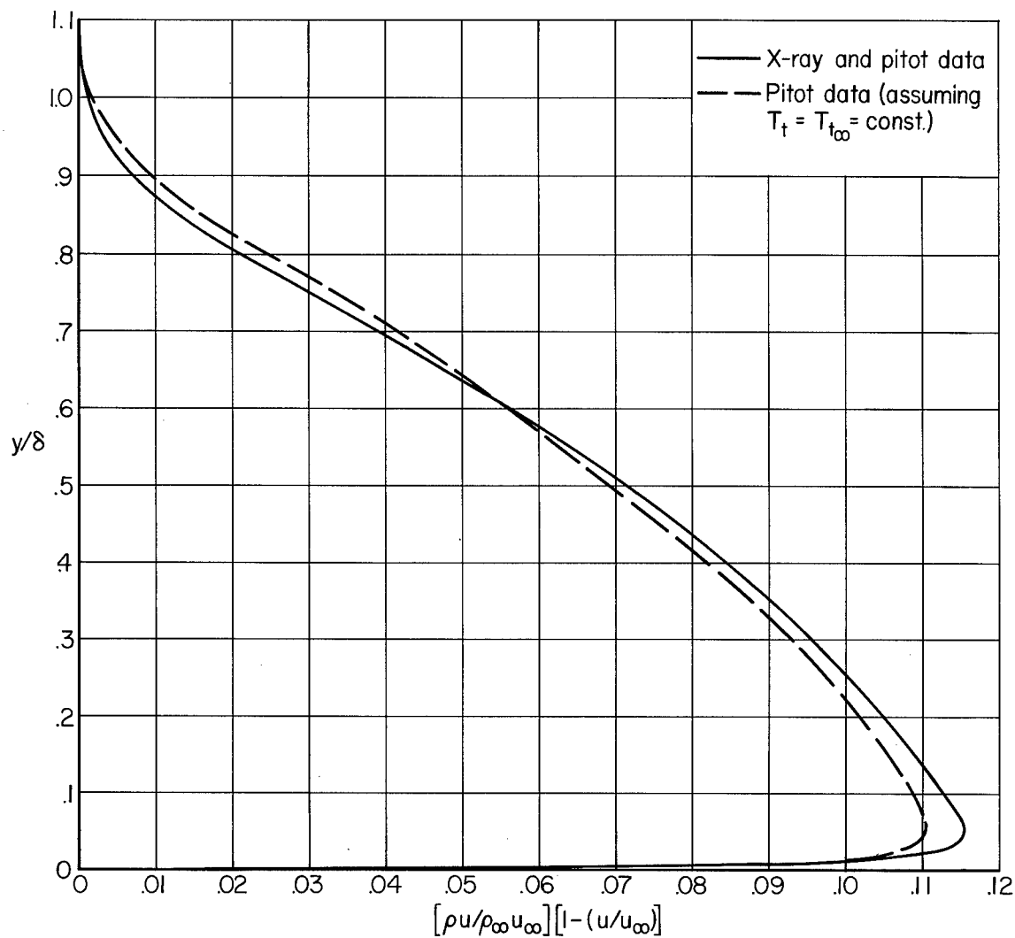
Figure 16.- Momentum-loss distributions through the turbulent boundary layer.
