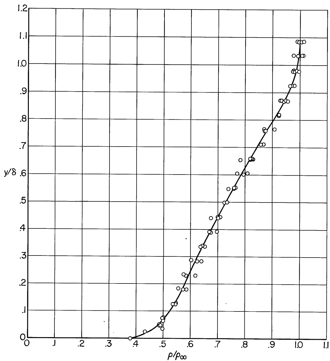
Figure 8.- Density distribution through the turbulent boundary layer from X-ray densitometer measurements.
