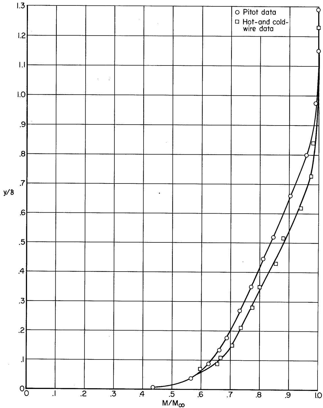
Figure 12.- Mach number distributions through the turbulent boundary layer on the side wall of the Ames 1-by 3-foot supersonic wind tunnel from pitot, cold-wire, and hot-wire data; M_\infty = 1.95 , \delta = 2.84 inches.
