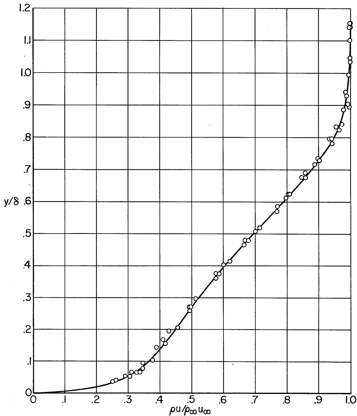
Figure 10.- Mass-flow distribution through the turbulent boundary layer from hot-wire measurements.
