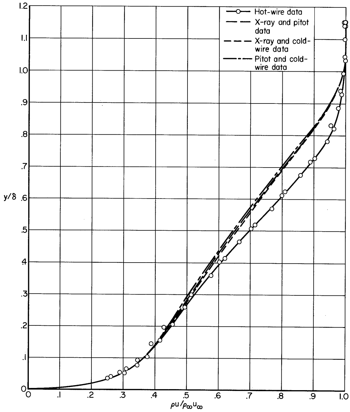
Figure 14.- Mass-flow distributions through the turbulent boundary layer from pitot, X-ray, cold-wire, and hot-wire data.
