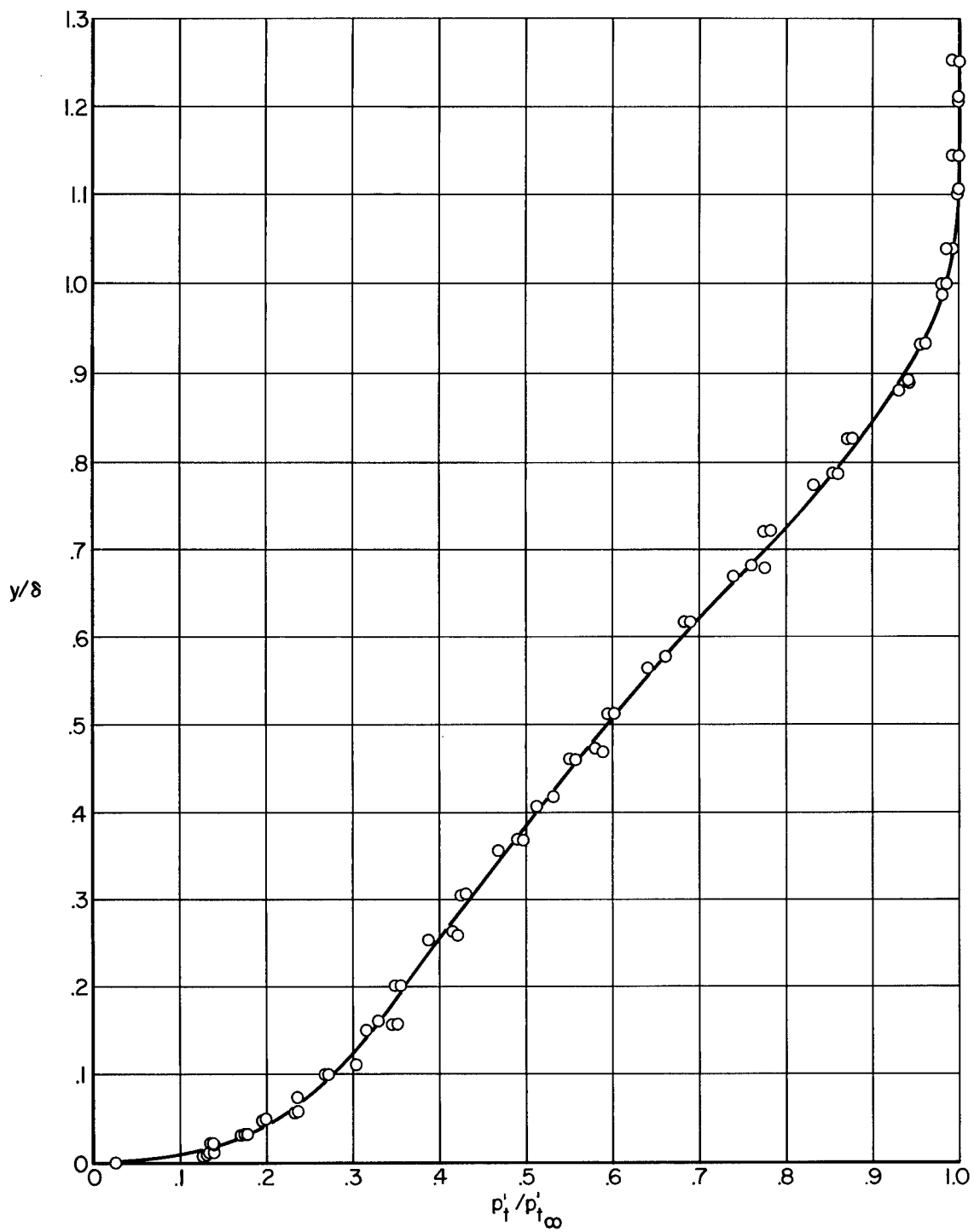
Figure 7.- Pitot-pressure distribution through the turbulent boundary layer from pitot-probe measurements.
