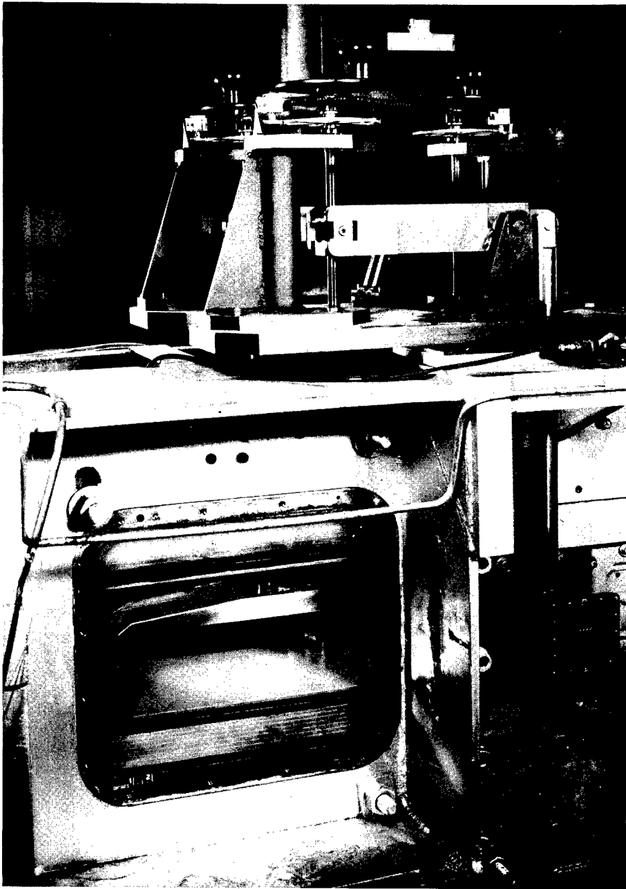
Figure 1.- General arrangement of flat-plate motion mechanism and flat plate in test region of 8- by 8-inch supersonic nozzle.
