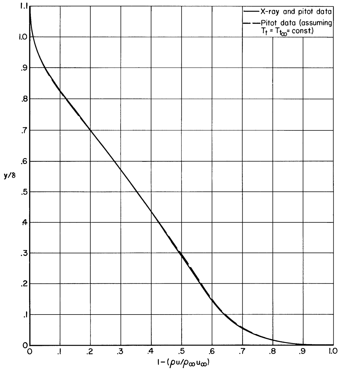
Figure 15.- Mass-flow-defect distributions through the turbulent boundary layer.
