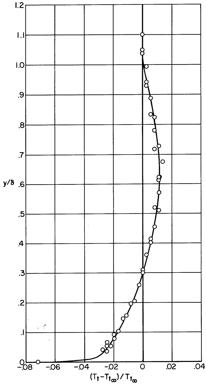
Figure 9.- Total-temperature distribution through the turbulent boundary layer from cold-wire-resistance measurements.
