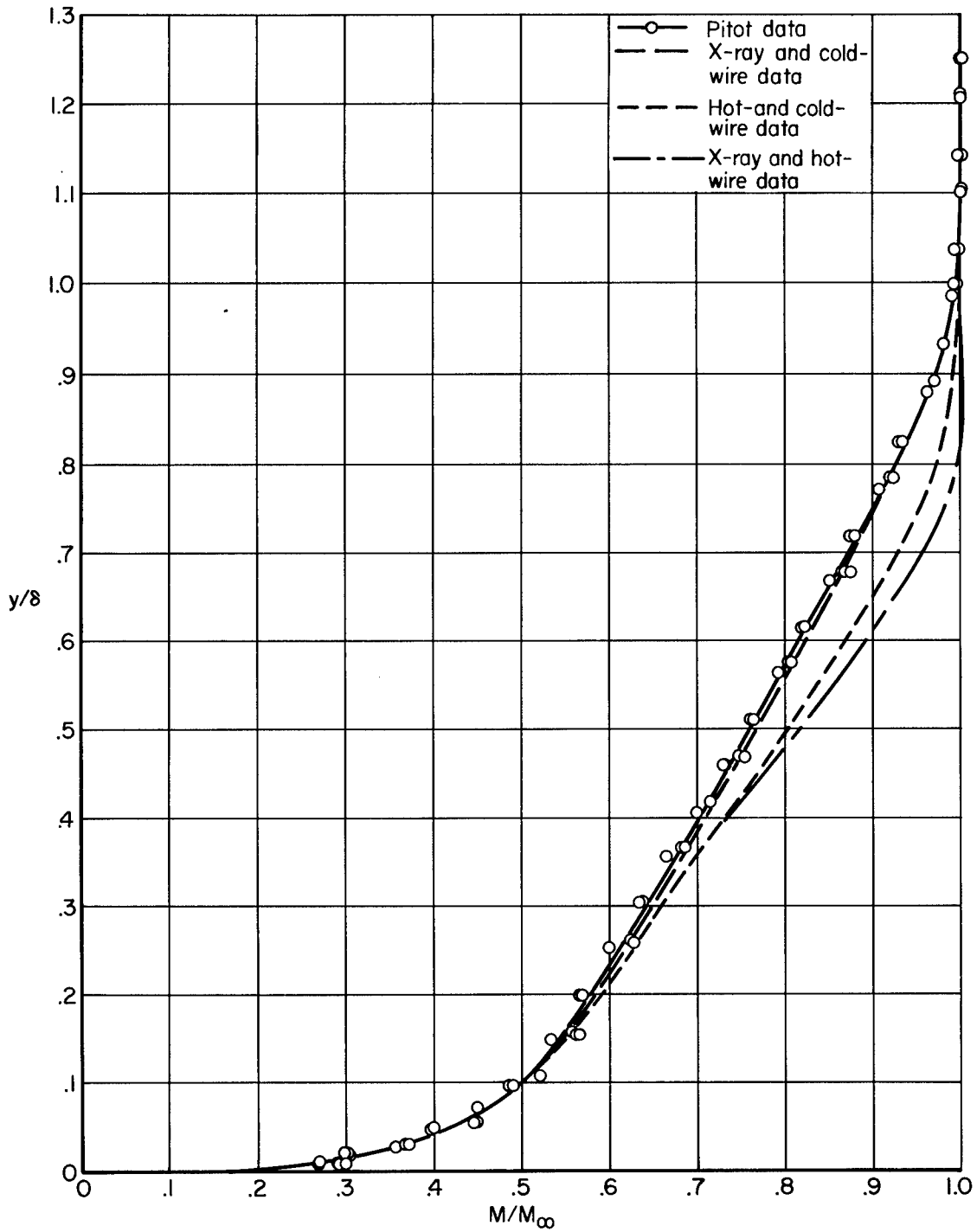
Figure 11.- Mach number distributions through the turbulent boundary layer from pitot, X-ray, cold-wire, and hot-wire data.
