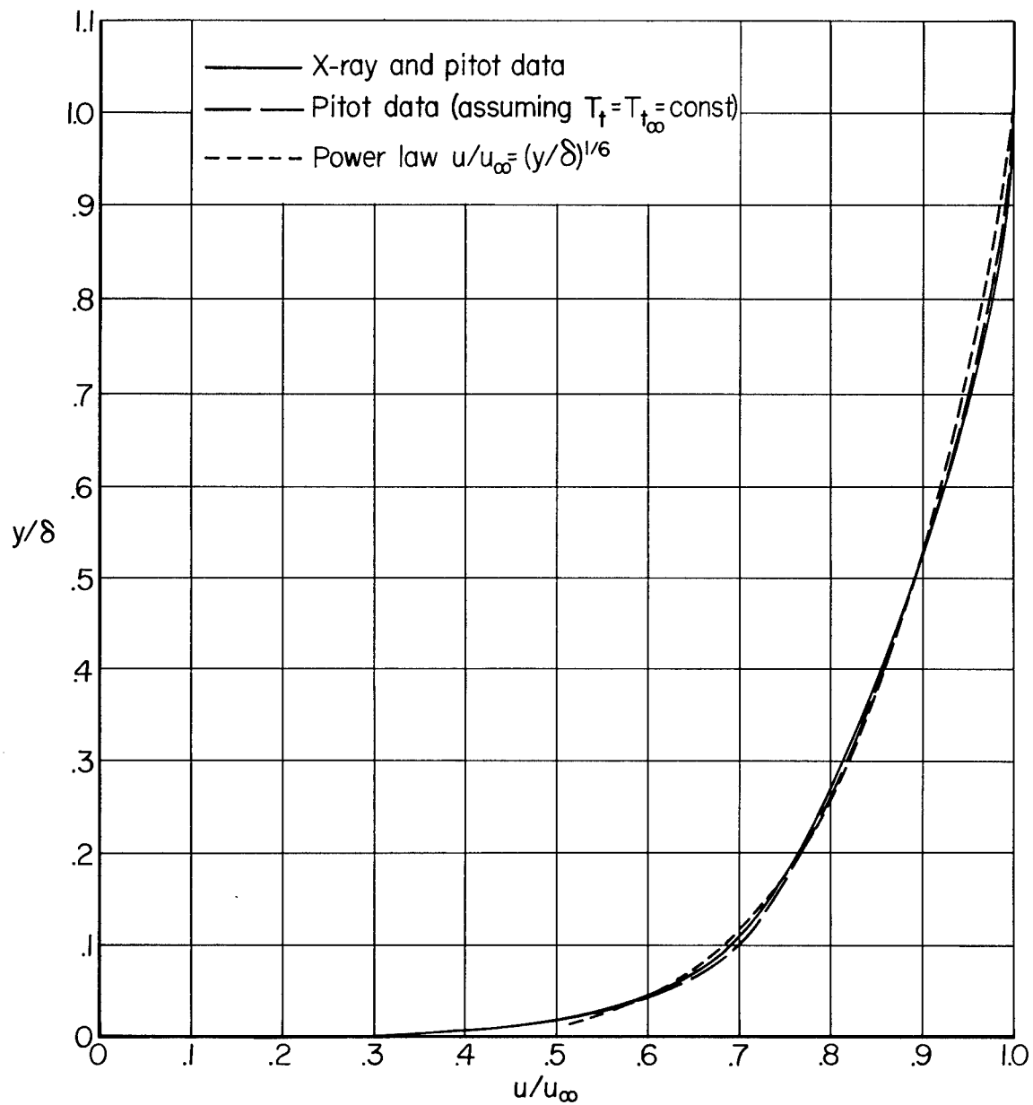
Figure 17.- Velocity distributions through the turbulent boundary layer.
