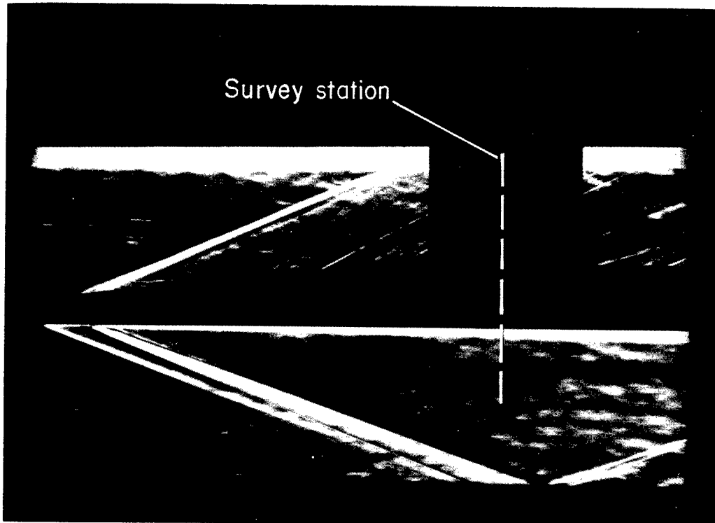
Figure 6.- Schlieren photograph of turbulent boundary layer on the flat plate.
