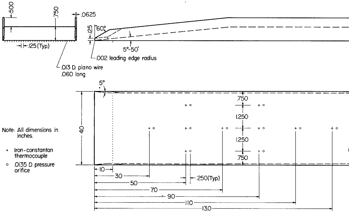
Figure 3.- Sketch of flat plate.
