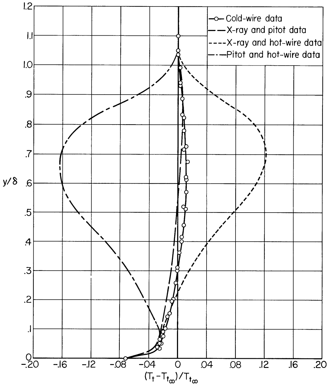
Figure 13.- Total-temperature distributions through the turbulent boundary layer from pitot, X-ray, cold-wire, and hot-wire data.
