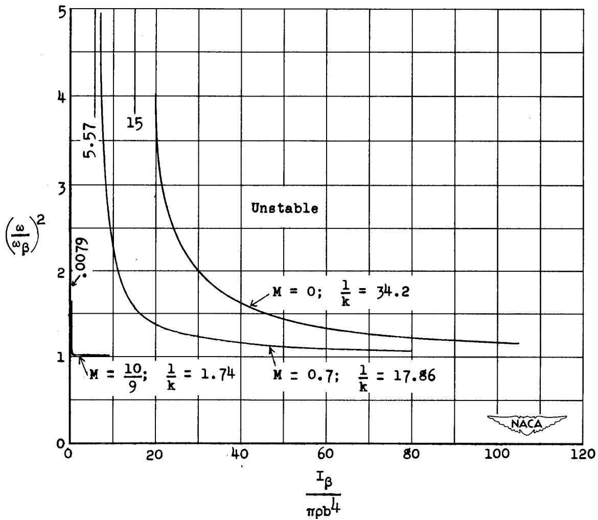
Figure 10.- Plot of frequency ratio (\frac{\omega}{\omega_\beta})^2 against an inertia parameter \frac{I_\beta}{\pi\rho b^4} for several values of Mach number M . c = 0.7 .
