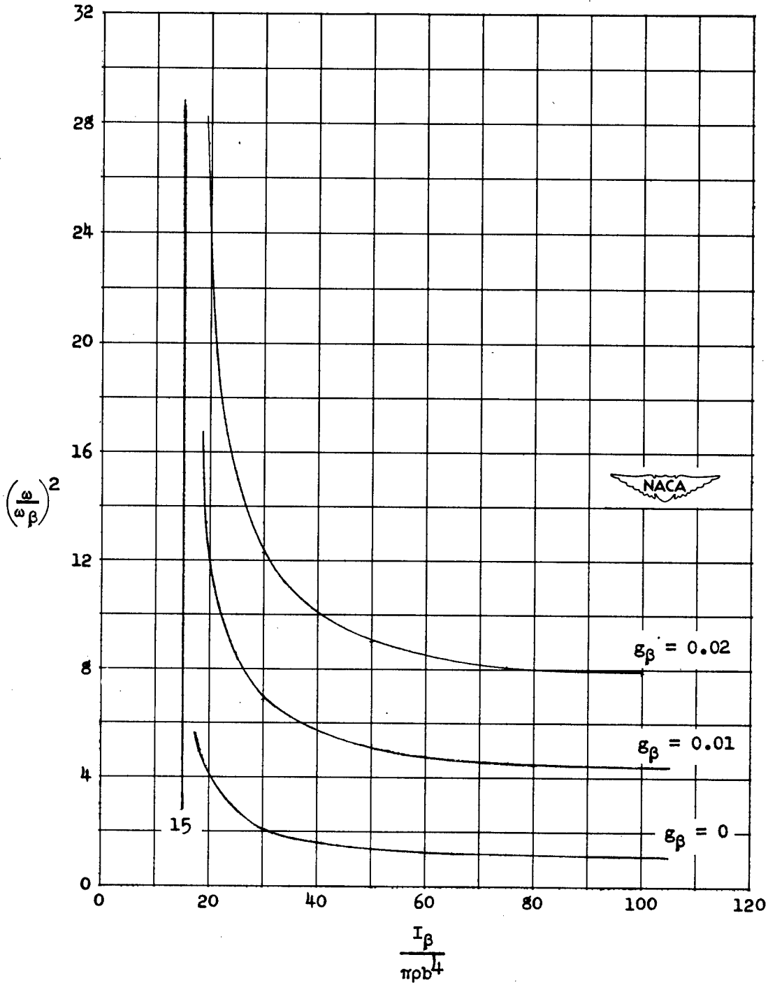
Figure 6.- Plots of frequency ratio (\frac{\omega}{\omega_\beta})^2 against an inertia parameter \frac{I_\beta}{\pi \rho b^4} for several values of structural damping \xi_\beta . c = 0.7 .
