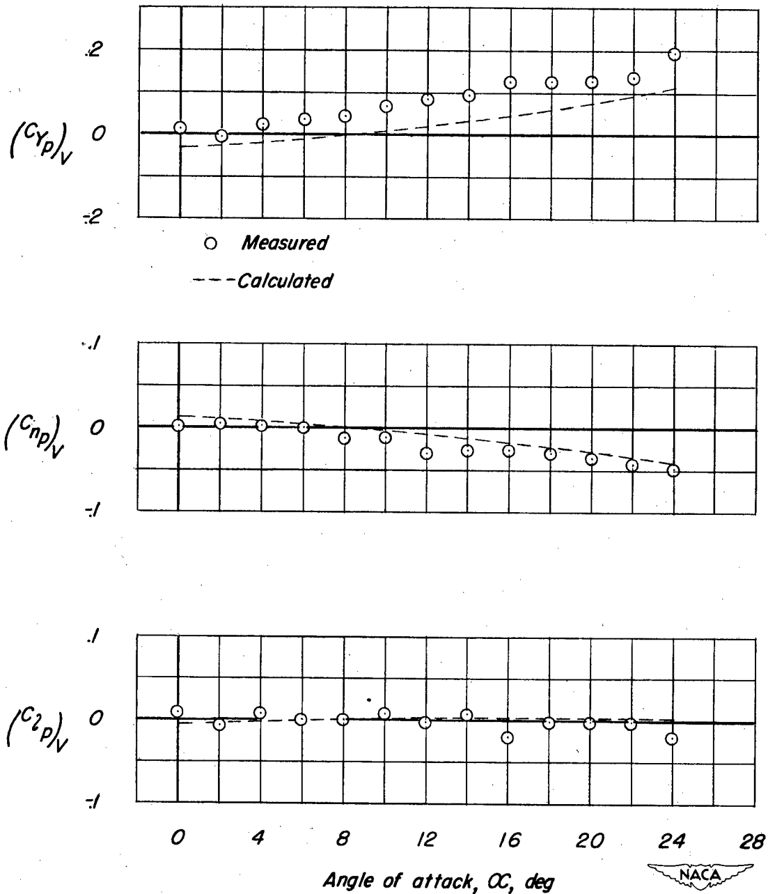
Figure 21.- Comparison of measured and calculated variation with angle of attack of (C_{Yp})_V , (C_{np})_V , and (C_{lp})_V for a 41.57^\circ sweptback near-midwing semitailless model (unpublished). Calculations based on \left(\frac{\partial \sigma_1}{\partial pb}\right)_{\frac{\partial \sigma_2}{\partial 2V}}_{\alpha=0^\circ} from reference 11 and \frac{\partial \sigma_2}{\partial pb} from equation (10).
