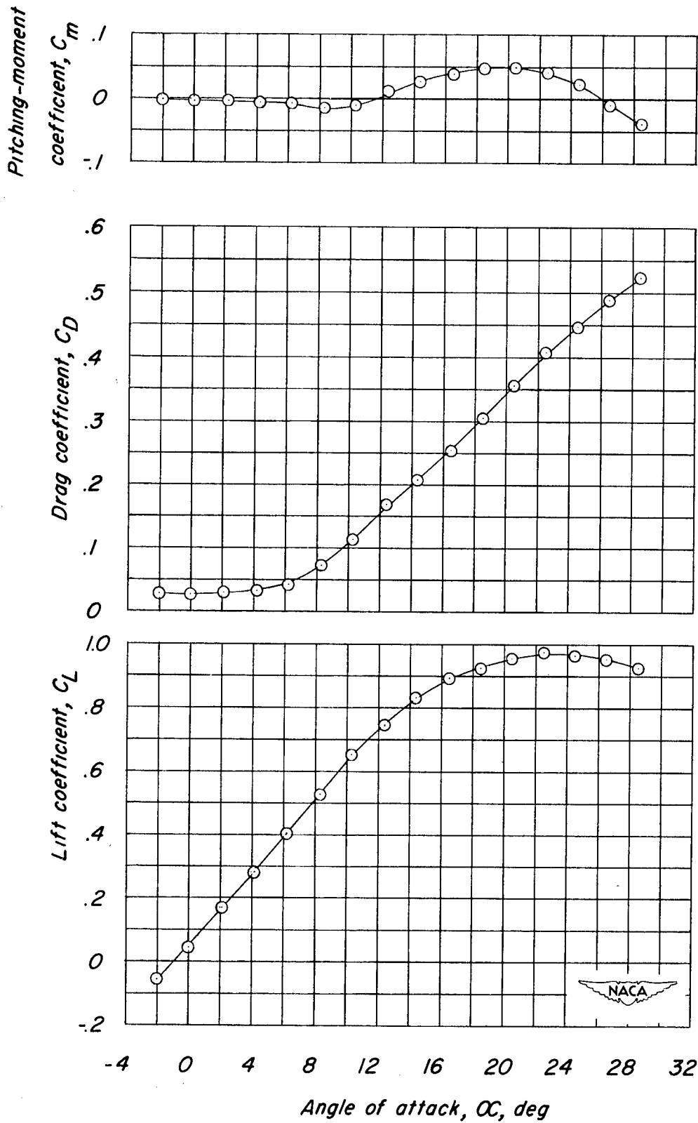
Figure 6.- Static longitudinal stability characteristics of the wing.
