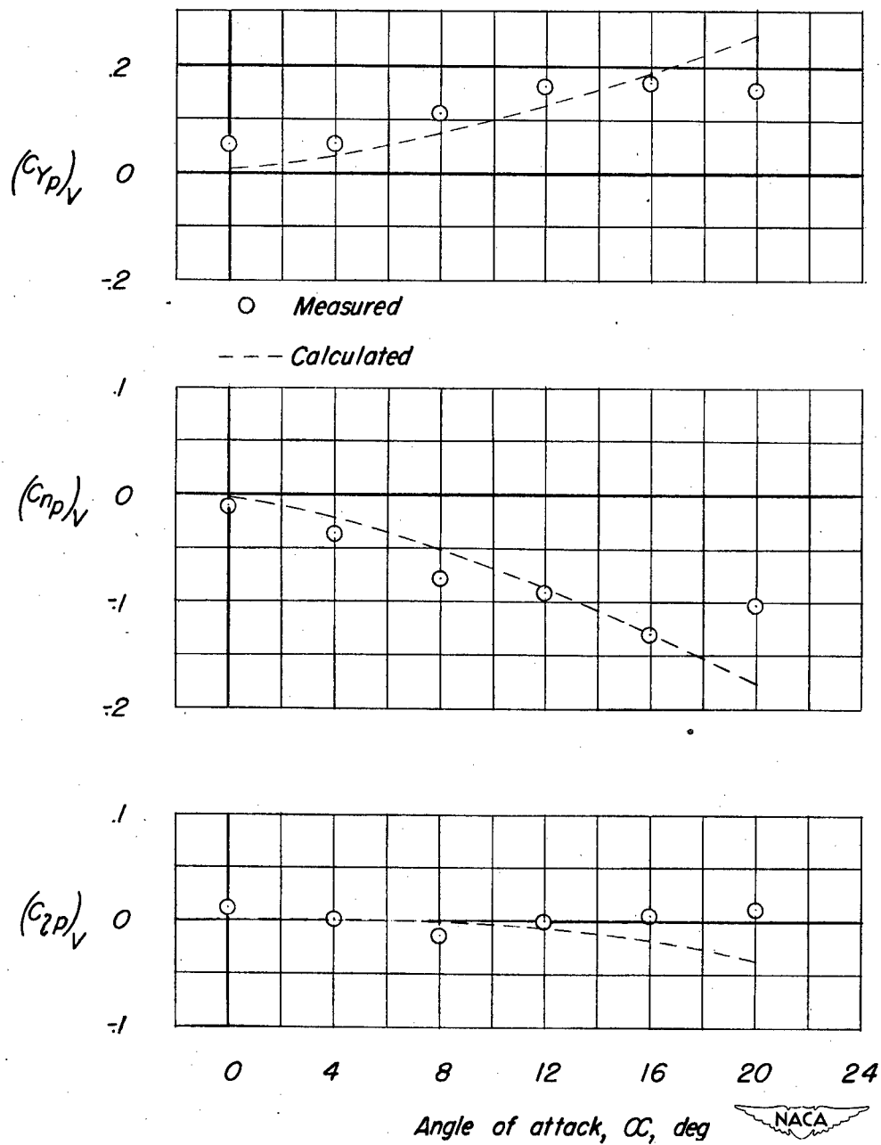
(c) Fuselage F_3 .
