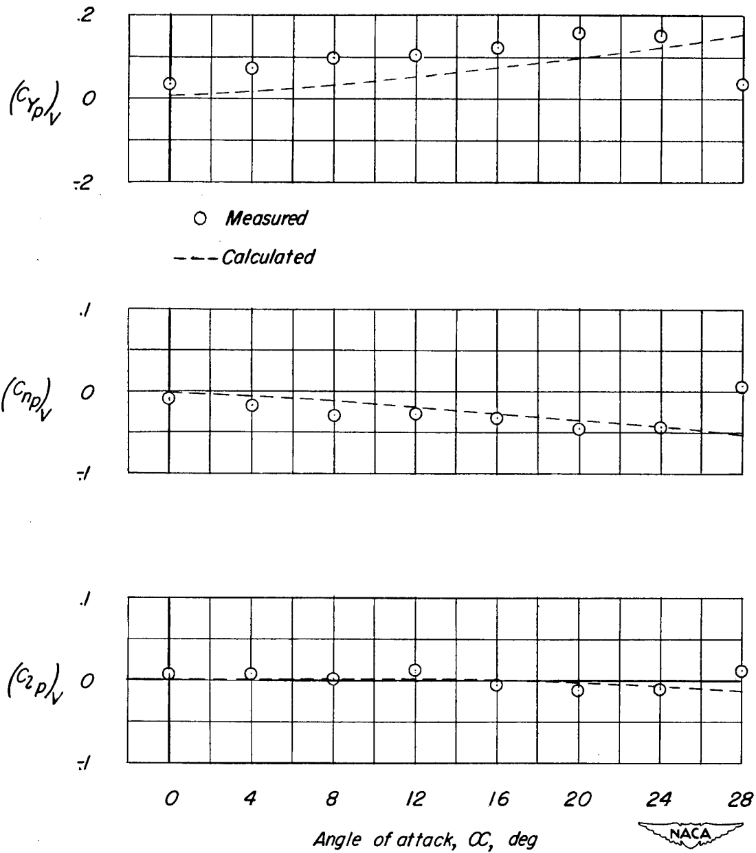
(b) Fuselage F_1 .
