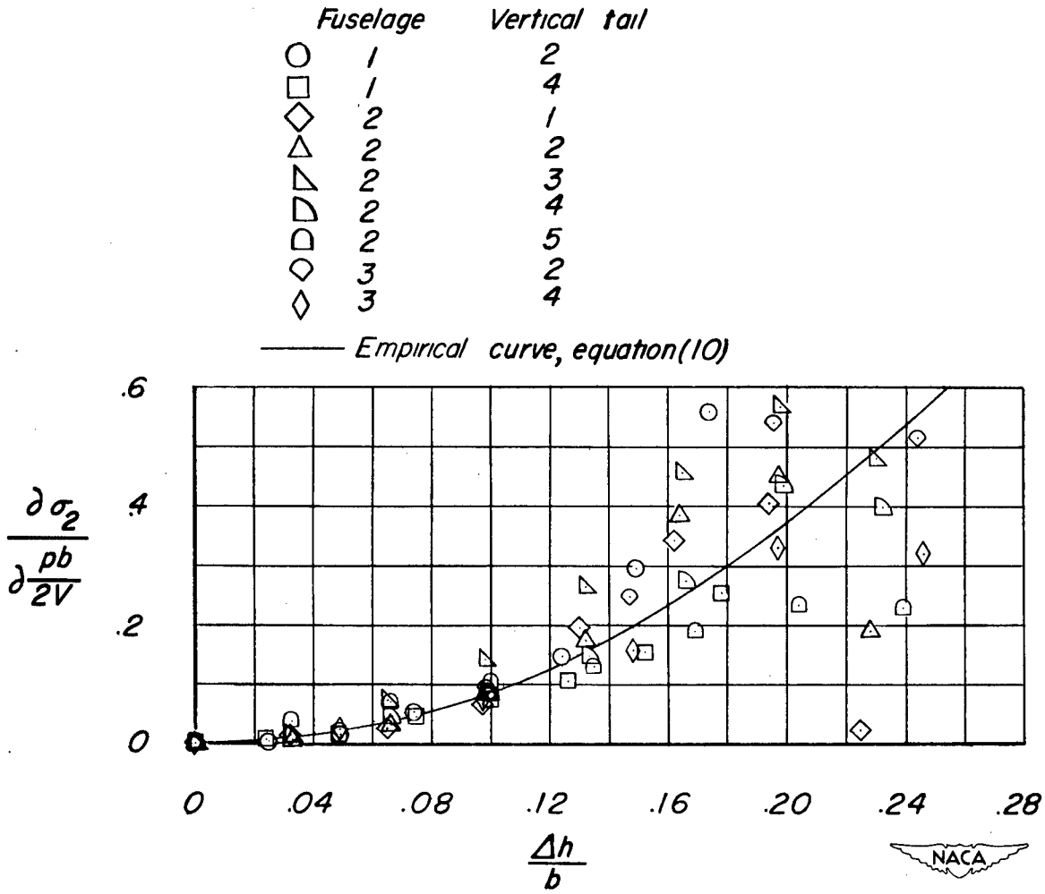
Figure 14.- Variation of \frac{\partial \sigma_2}{\partial \frac{pb}{2V}} with \frac{\Delta h}{b} . Wing off.
