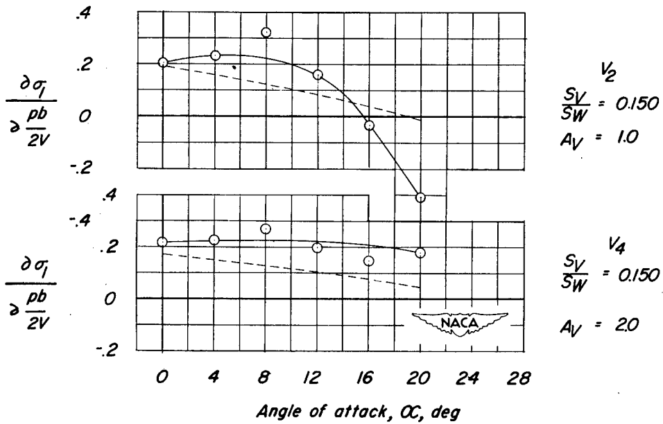
(c) Fuselage F 3 .
