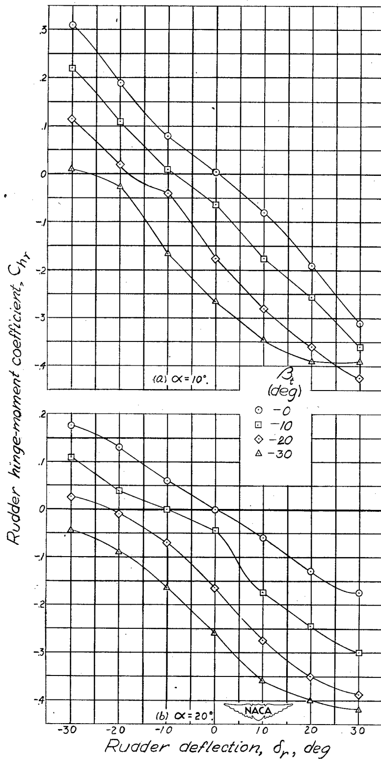
Figure 9.— Rudder hinge-moment coefficient as a function of rudder deflection for various angles of sideslip at specific angles of attack. Plain rudder; horizontal tail in high position; \delta_\theta = 0^\circ . Data from reference 4.
