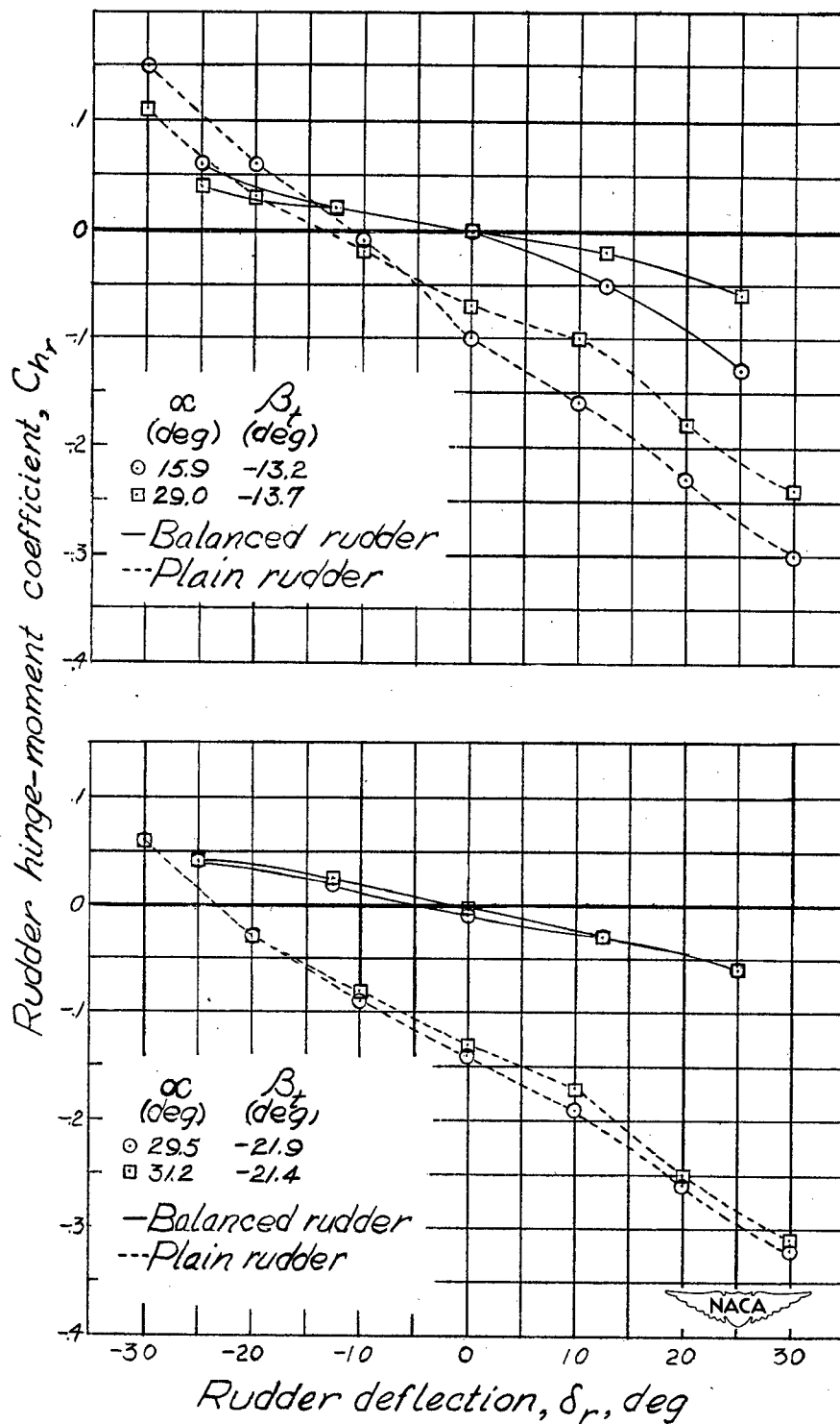
Figure 16.— Rudder hinge-moment coefficient as a function of rudder deflection at various spinning attitudes for a 27.9-percent-overhang-balanced and a plain rudder.
