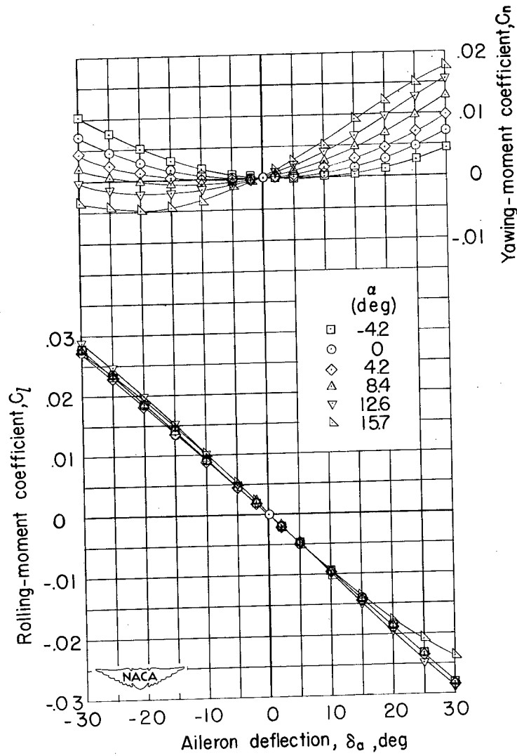
Figure 5.- Variation of lateral control characteristics with aileron deflection on the unswept semispan wing having an aspect ratio of 3.13.
