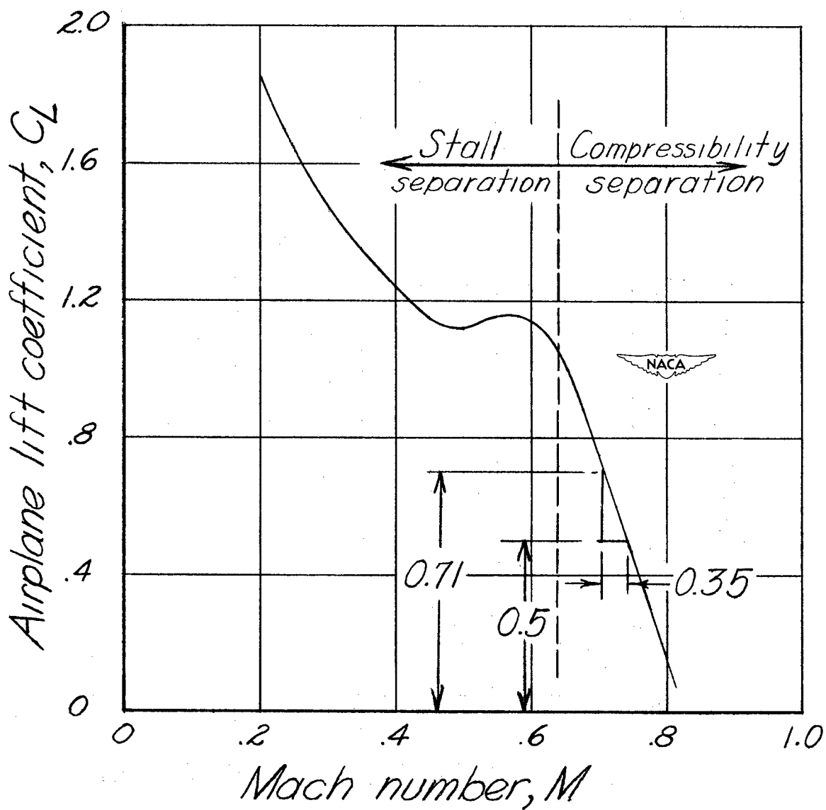
Figure 1.- Typical buffeting boundary for high-speed fighter airplane 1.
