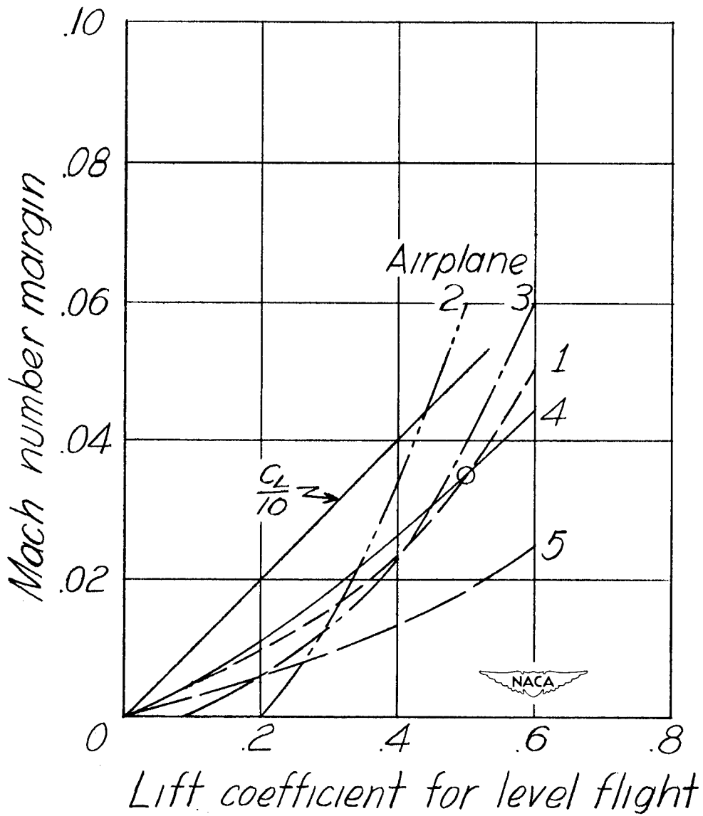
Figure 2.- Mach number margin required to execute 45^\circ bank without crossing the buffet boundary.
