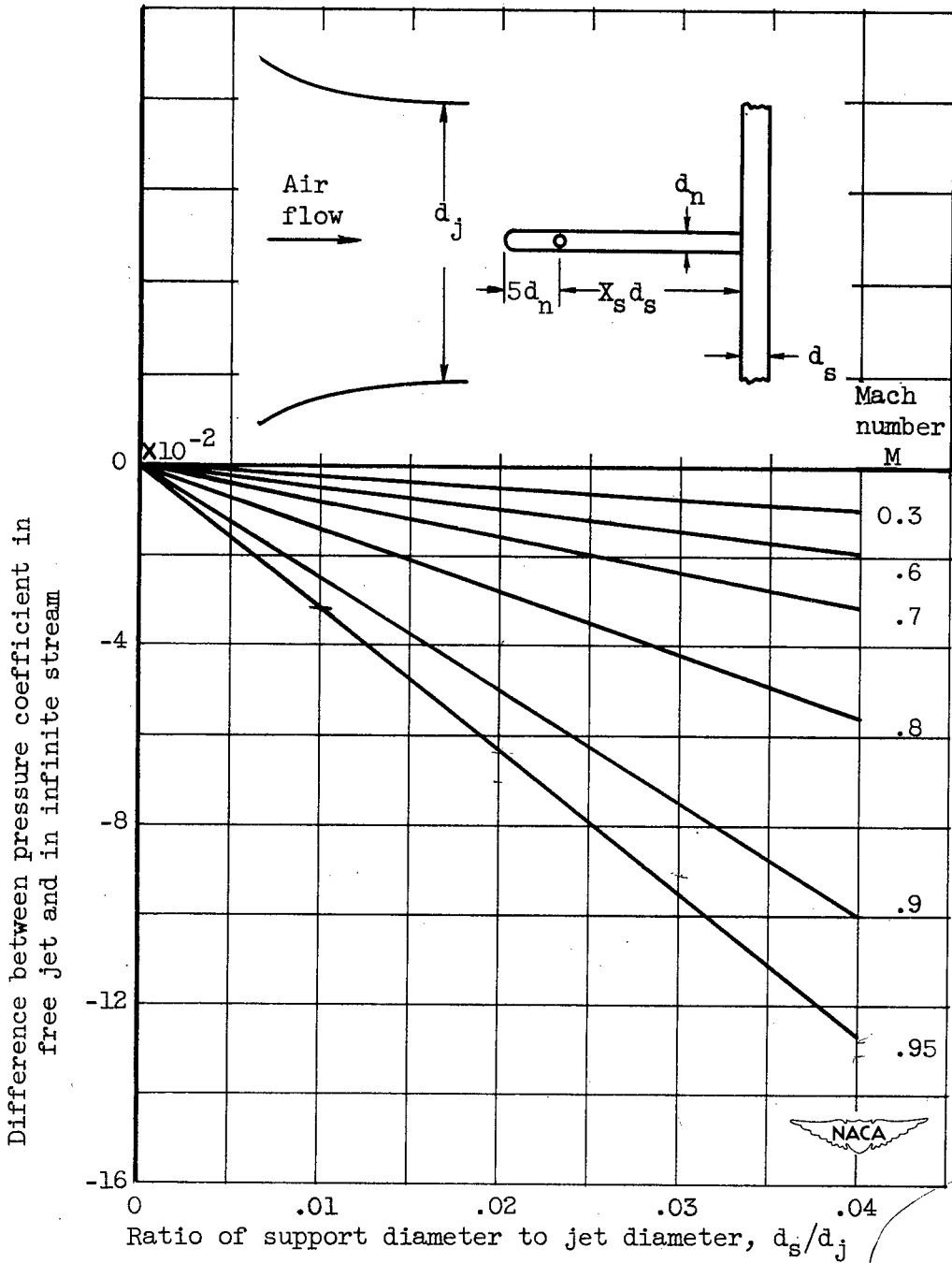
Figure 5. - Variation of difference between pressure coefficient in free jet and in infinite stream with ratio of support diameter to jet diameter; d_n/d_s , 0.5; X_s , 5 to 10.
