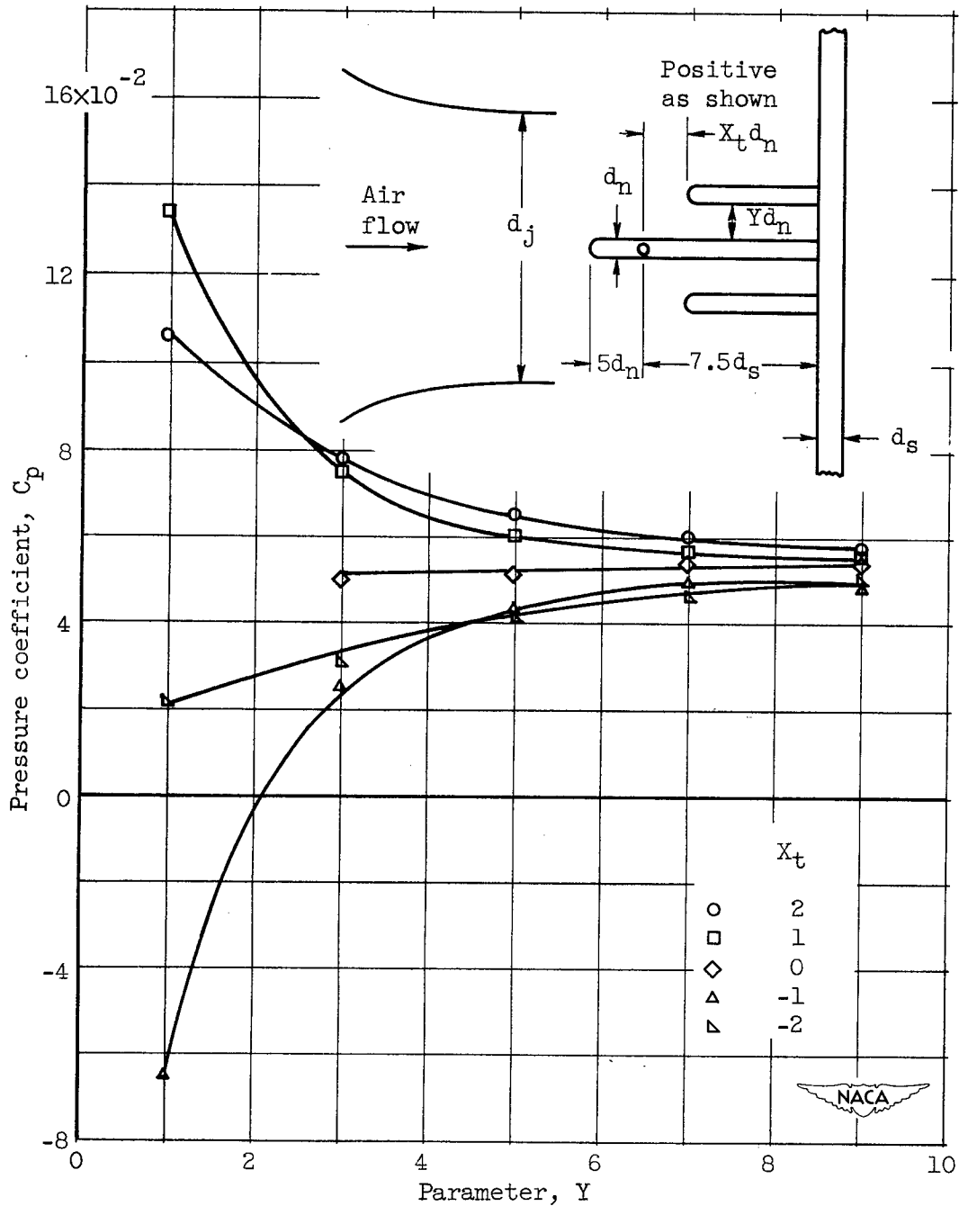
(c) Mach number, M = 0.8 .
