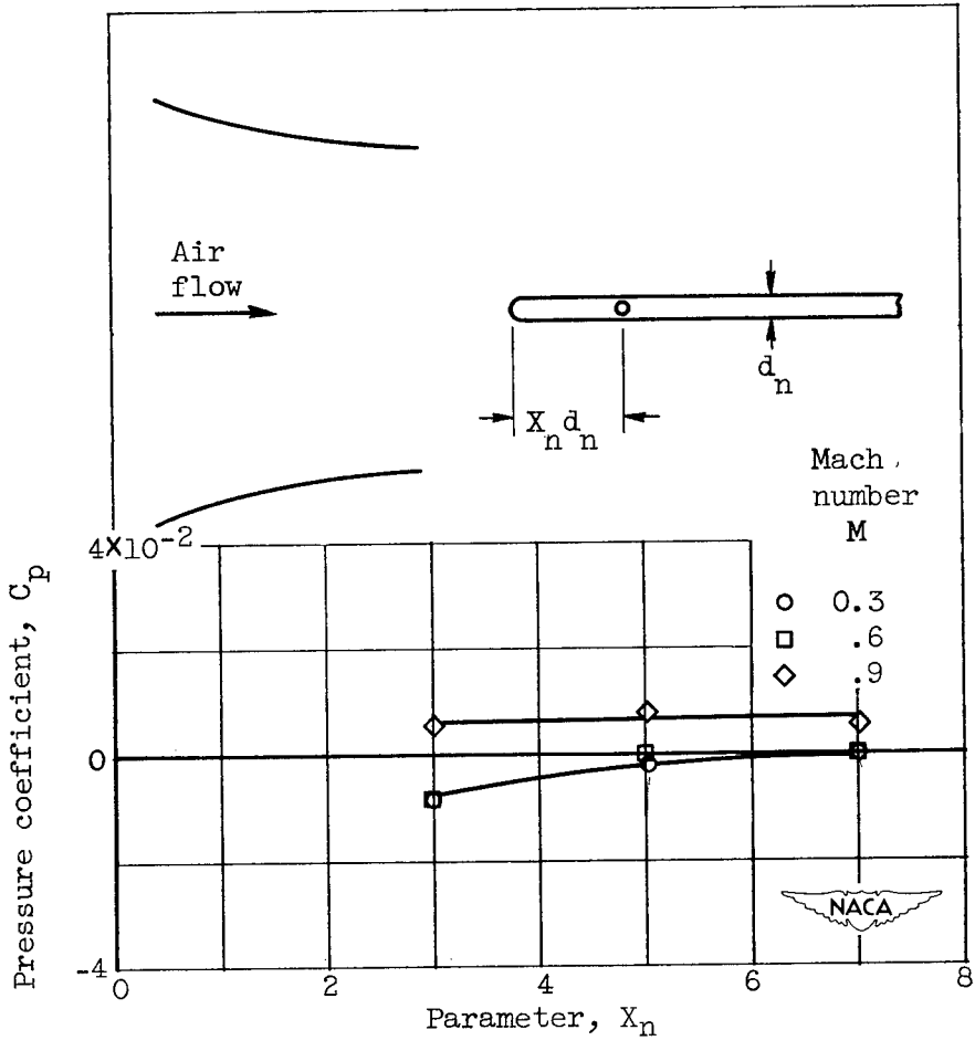
Figure 2. - Variation of pressure coefficient with distance from static orifices to leading edge of static-pressure tube.
