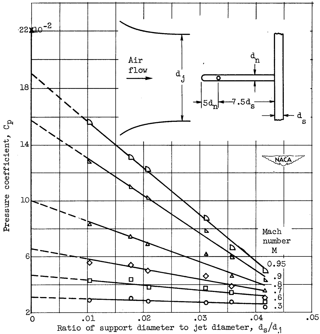
(b) Parameter, X_s = 7.5 .
