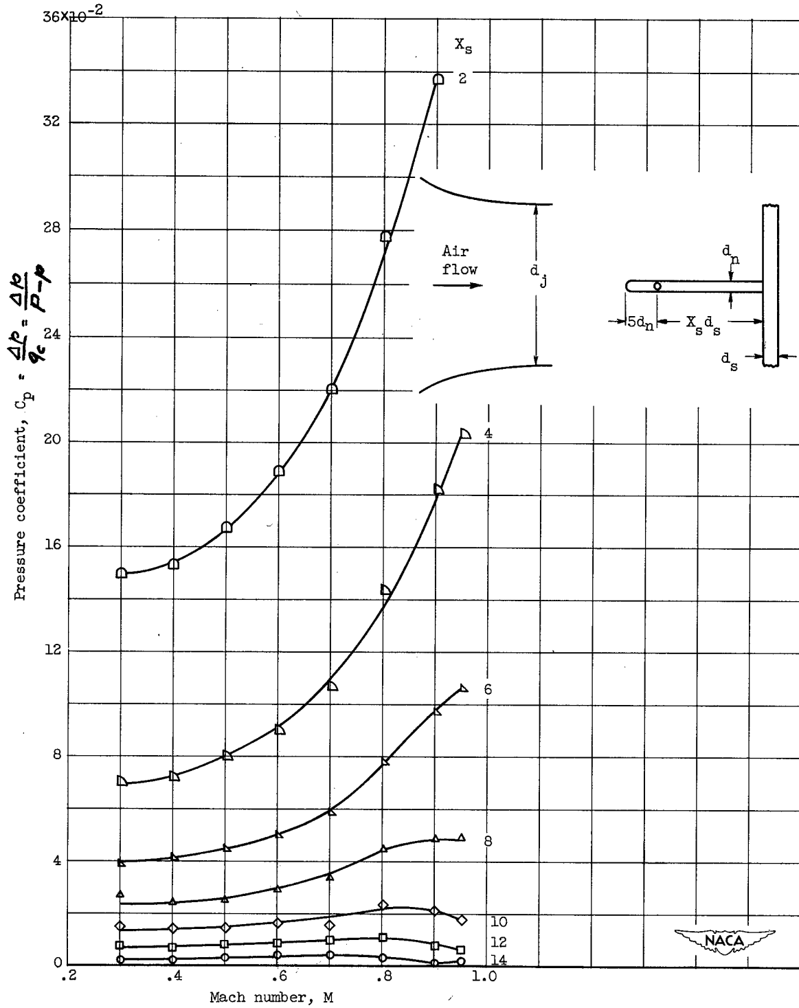
Figure 3. - Variation of pressure coefficient with Mach number for support at distance X_s d_s behind static orifices; d_n/d_s, 0.5 ; d_s/d_j, 0.036 .
