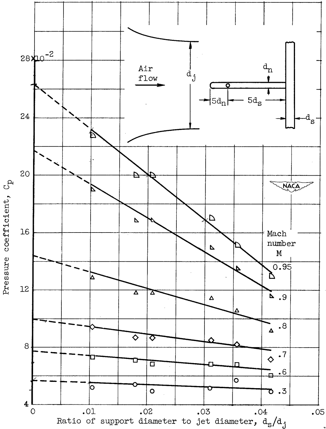
(a) Parameter, X_s = 5 .
