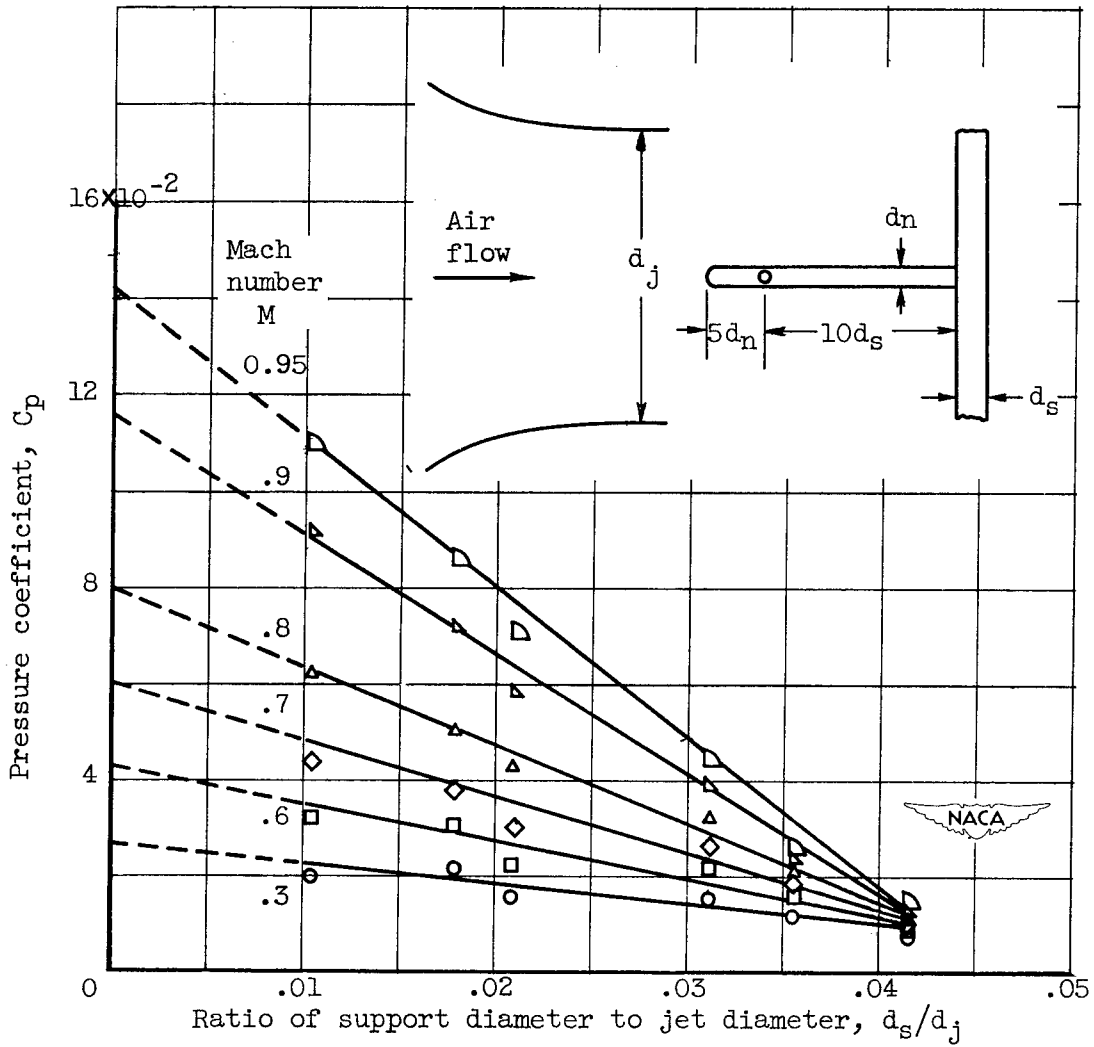
(c) Parameter, X_s = 10 .
