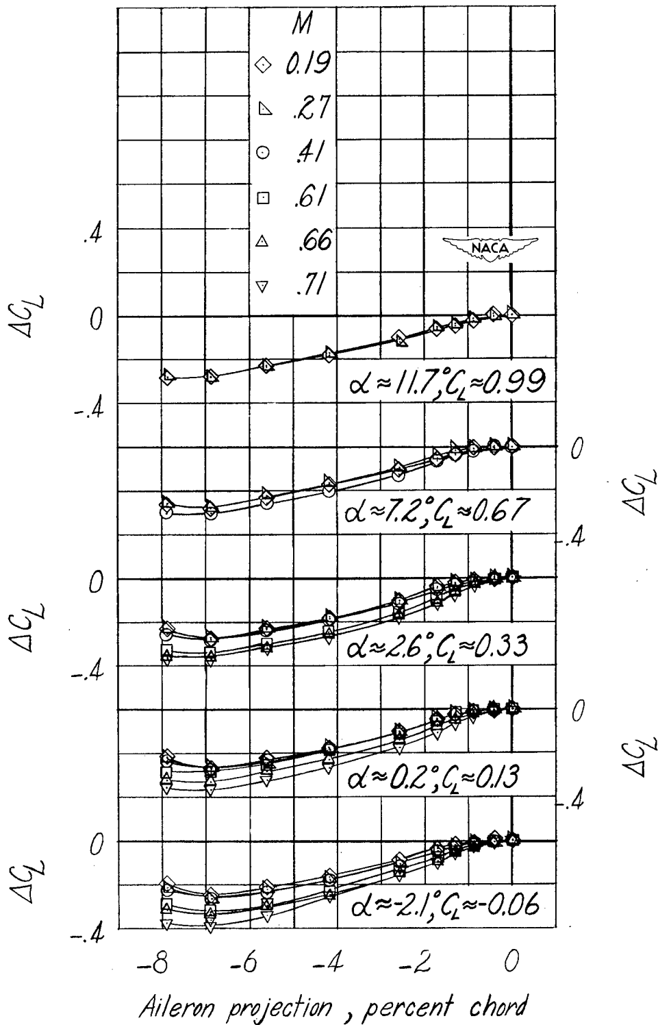
Figure 10.— Incremental values of lift, drag, and pitching-moment coefficients obtained by projection of the basic retractable aileron on both semispans of the NACA 65-210 wing. Flap retracted.
