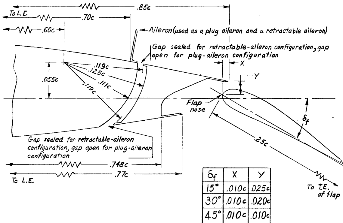
(a) Aileron configuration on the plain wing.
