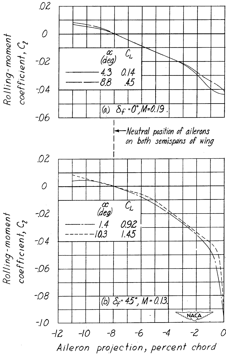
Figure 29.— Variation of rolling-moment coefficient of complete wing with projection of plug aileron on one semispan of NACA 65 2 -215 wing.
