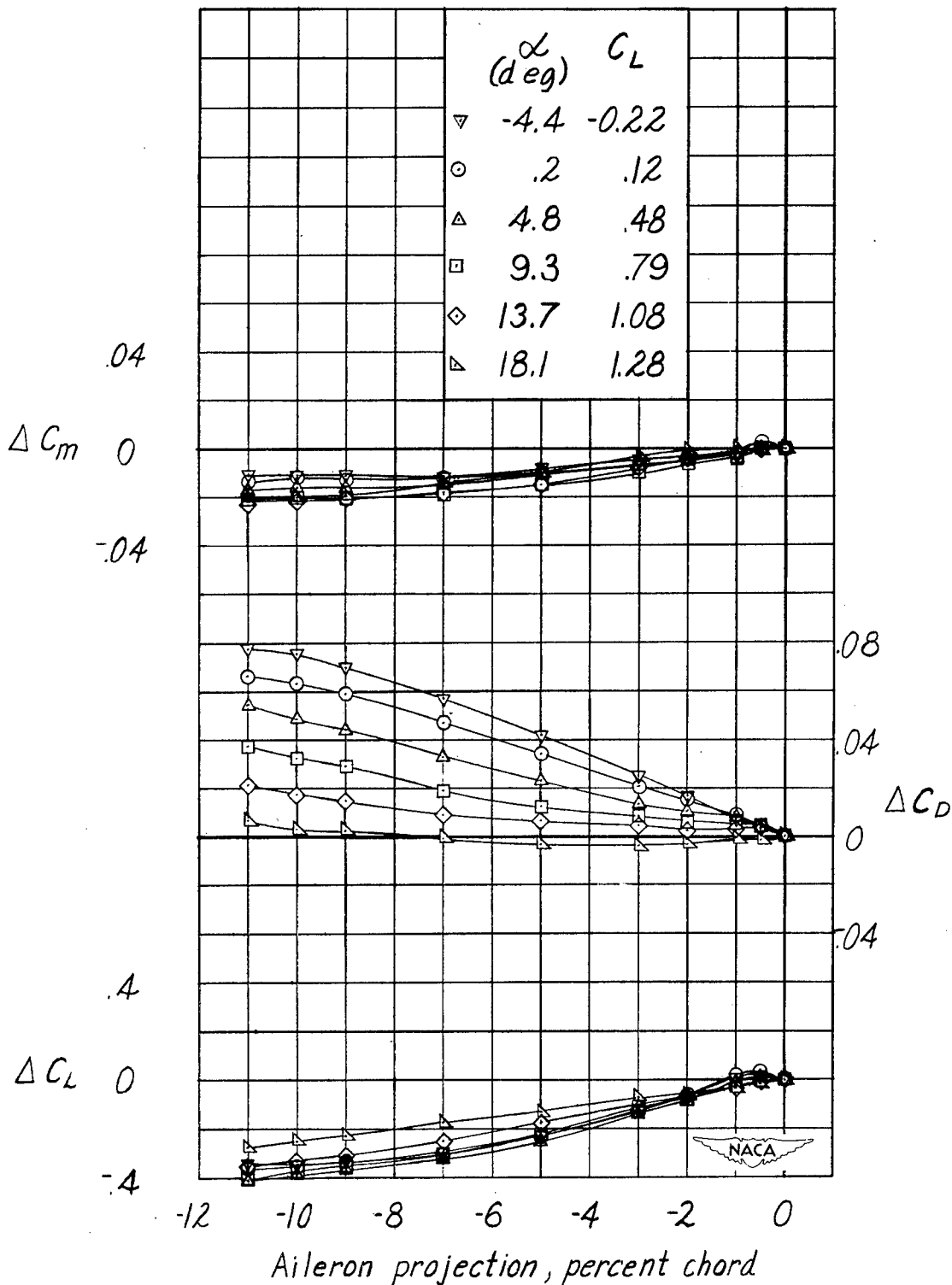
Figure 20.— Incremental values of lift, drag, and pitching-moment coefficients obtained by projection of the retractable aileron on both semispans of the NACA 65 2 -215 wing. Plain wing; M = 0.19.
