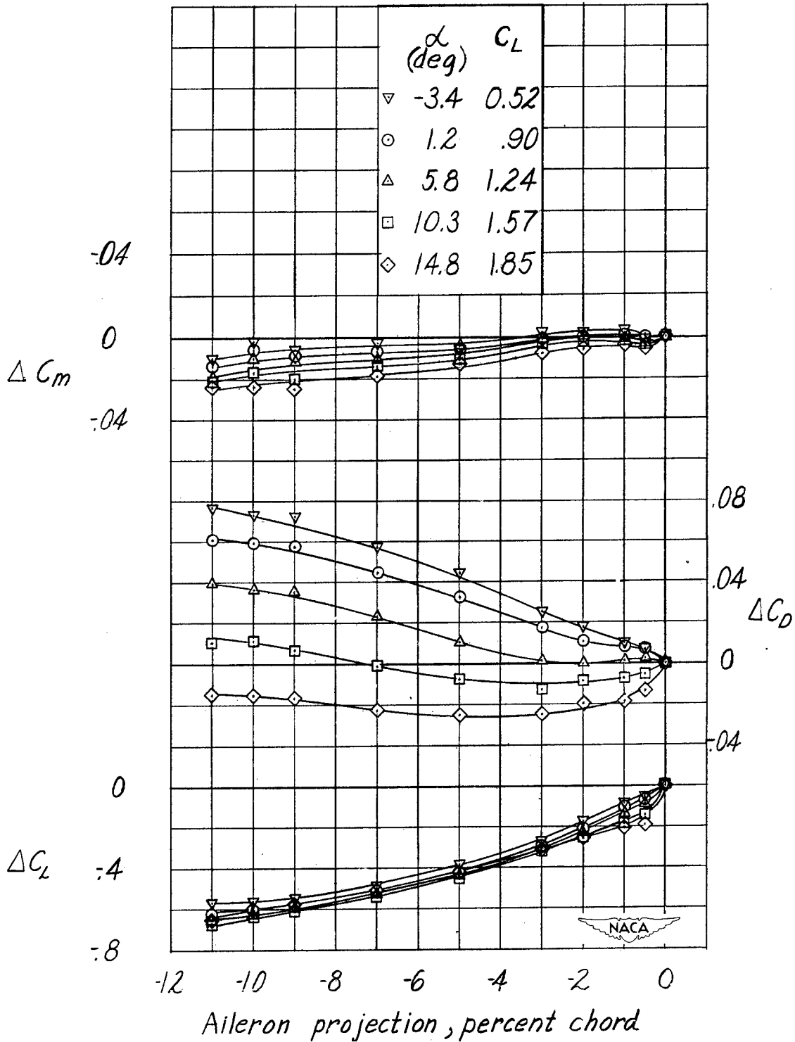
Figure 17.— Incremental values of lift, drag, and pitching-moment coefficients obtained by projection of the plug aileron on both semispans of the NACA 65 2 -215 wing. Flap deflected 15°; M = 0.13.
