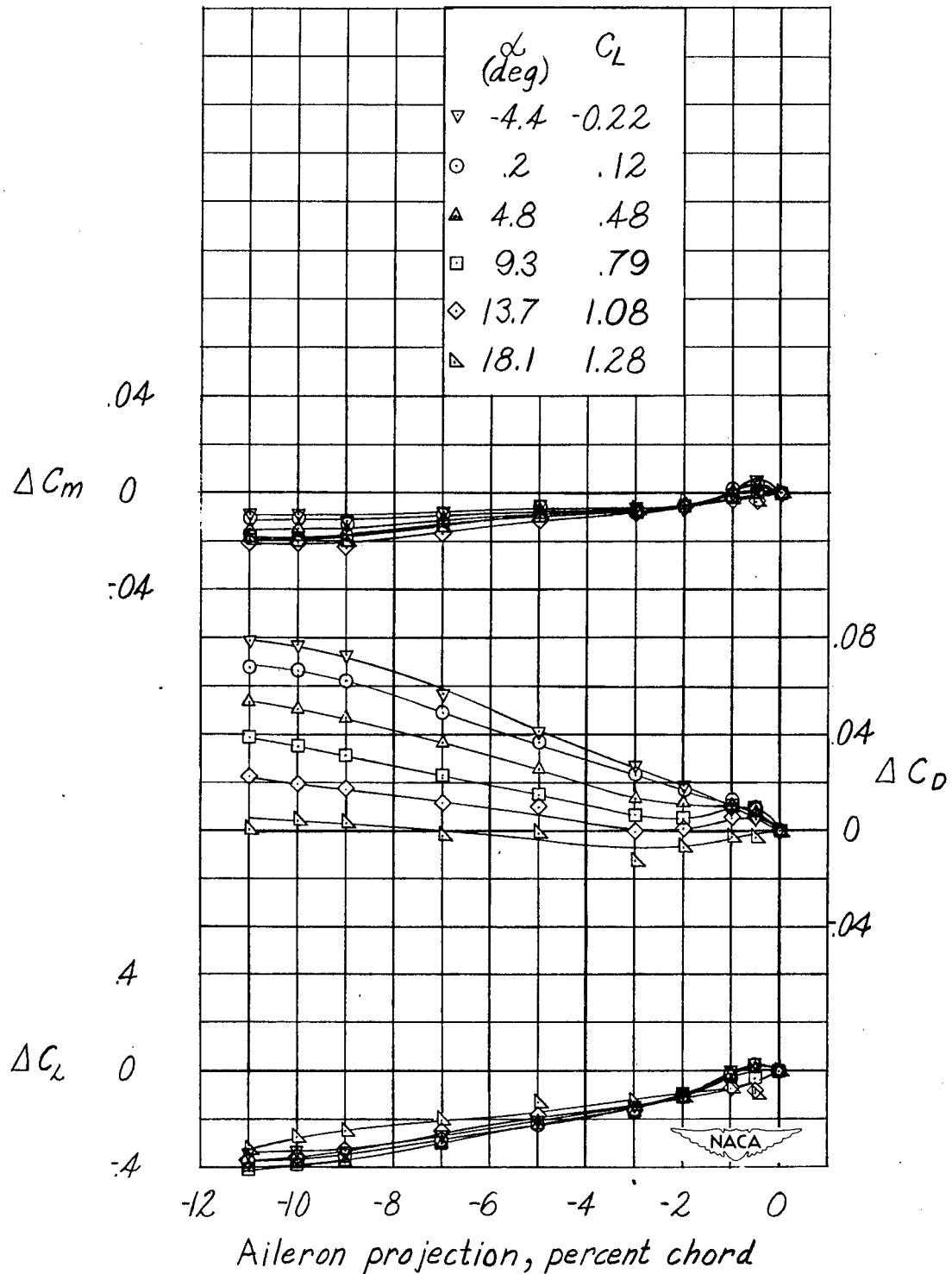
Figure 16.- Incremental values of lift, drag, and pitching-moment coefficients obtained by projection of the plug aileron on both semispans of the NACA 65 2 -215 wing. Plain wing; M = 0.19.
