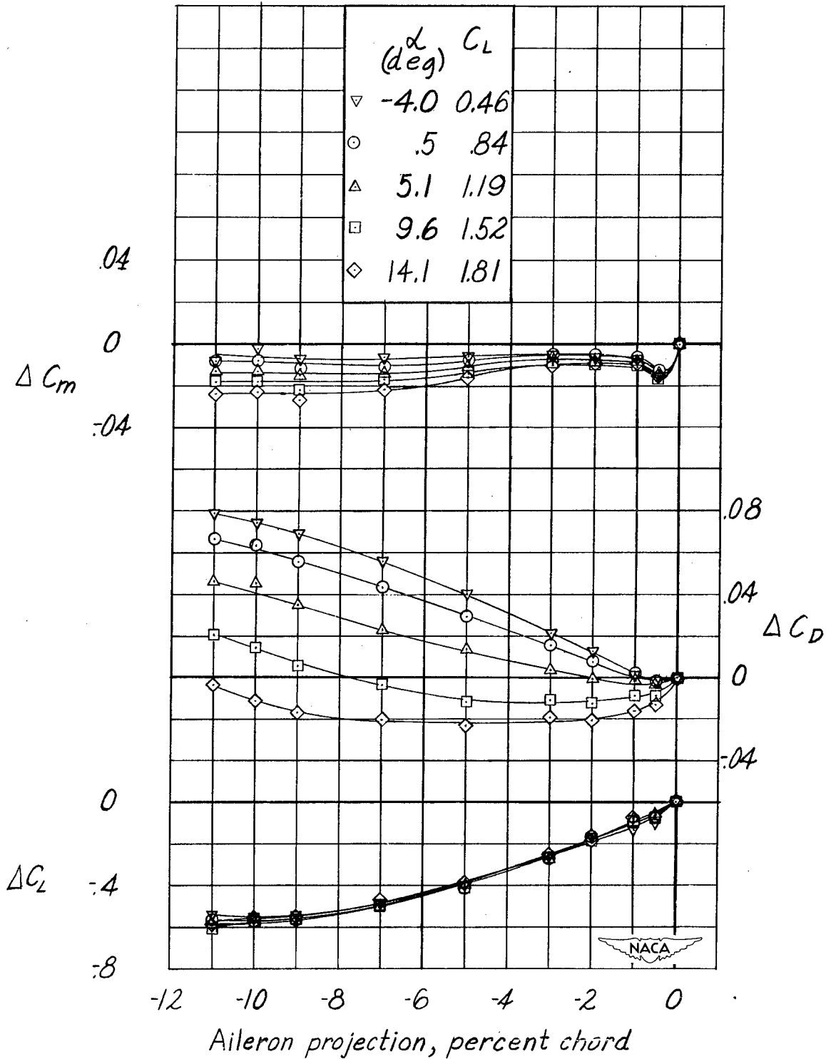
Figure 21.— Incremental values of lift, drag, and pitching-moment coefficients obtained by projection of the retractable aileron on both semispans of the NACA 65 2 -215 wing. Flap deflected 15°; M = 0.13.
