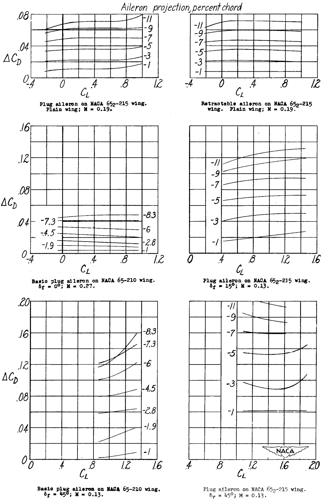
Figure 24.— Incremental values of drag coefficient obtained at constant lift coefficient for several of the wing aileron configurations investigated.
