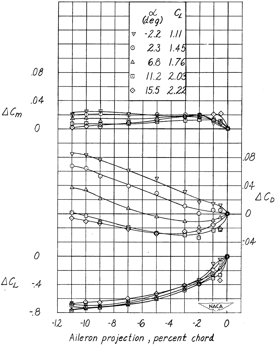
Figure 18.- Incremental values of lift, drag, and pitching-moment coefficients obtained by projection of the plug aileron on both semispans of the NACA 65 2 -215 wing. Flap deflected 30°; M = 0.13.
