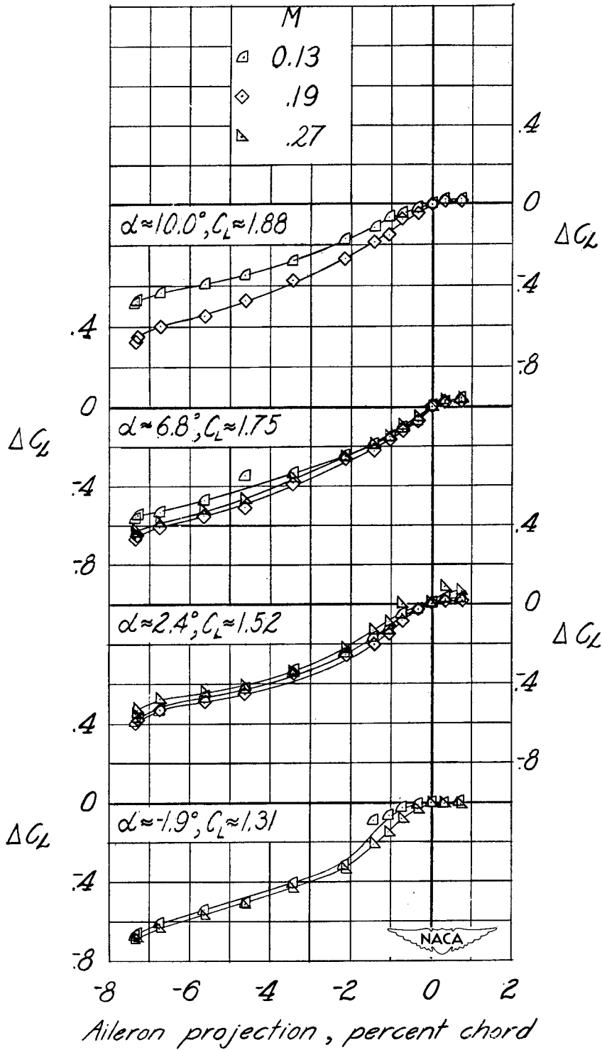
Figure 15.- Incremental values of lift, drag, and pitching-moment coefficients obtained by projection of the double-walled circular plug aileron on both semispans of the NACA 65-210 wing. Flap deflected 45^\circ .
