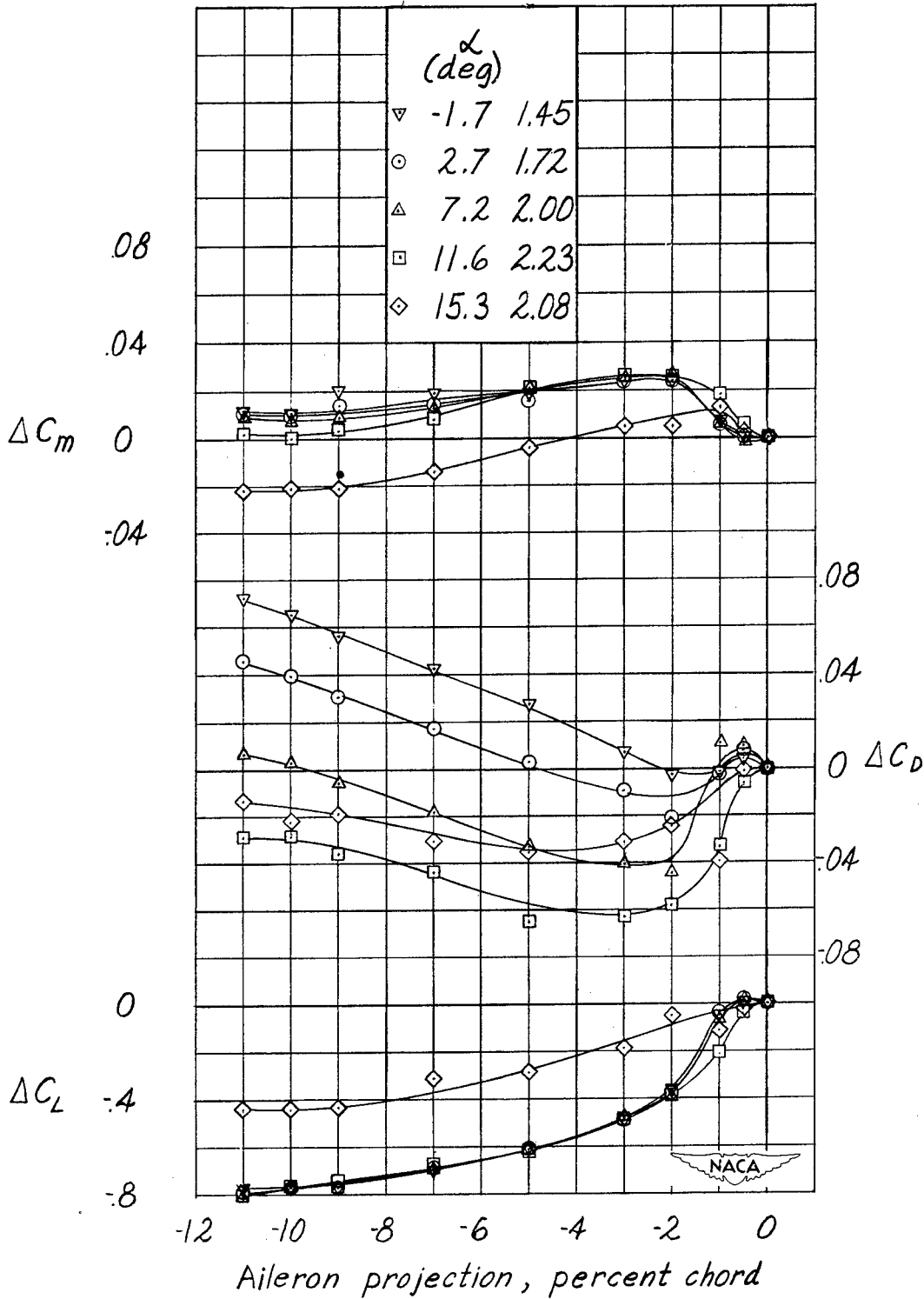
Figure 23.— Incremental values of lift, drag, and pitching-moment coefficients obtained by projection of the retractable aileron on both semispans of the NACA 65 2 -215 wing. Flap deflected 45°; M = 0.13.
