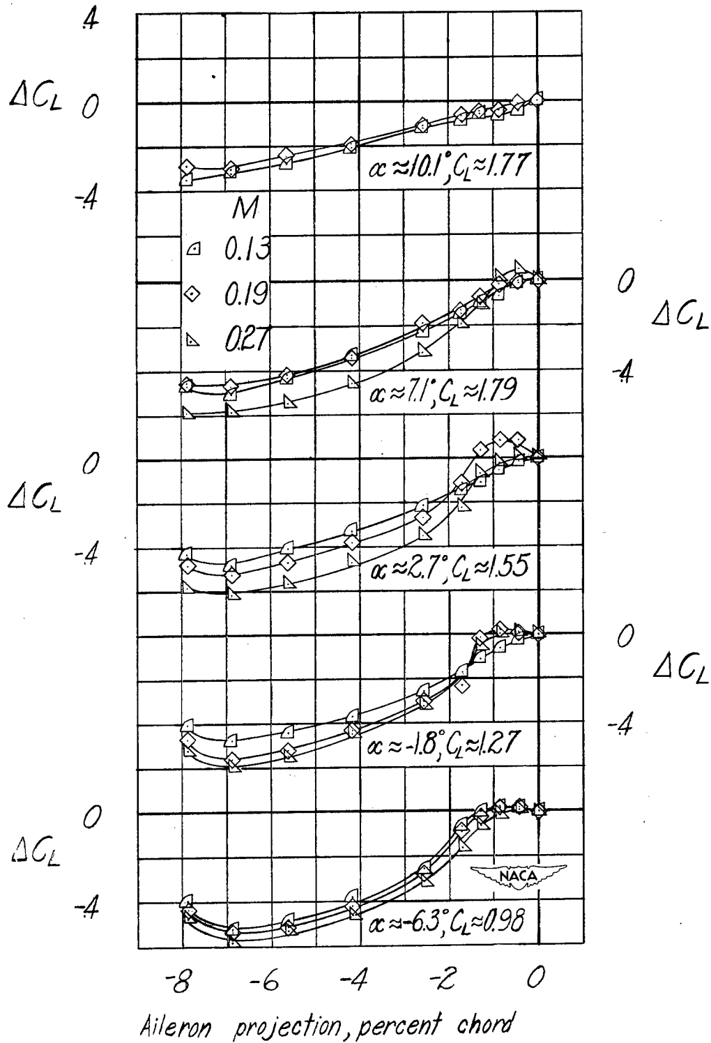
Figure 11.— Incremental values of lift, drag, and pitching-moment coefficients obtained by projection of the basic retractable aileron on both semispans of the NACA 65-210 wing. Flap deflected 45^\circ .
