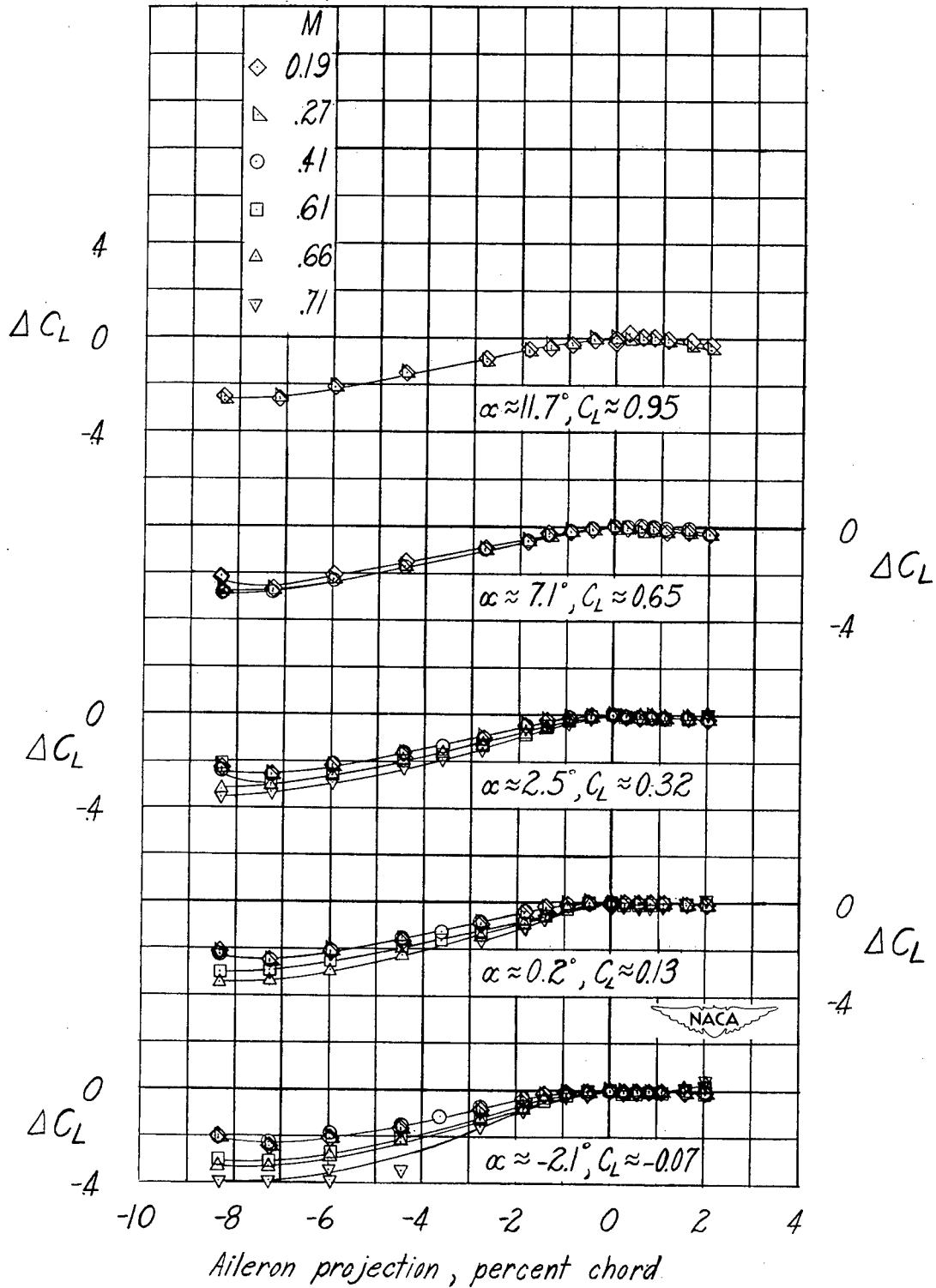
Figure 8.— Incremental values of lift, drag, and pitching-moment coefficients obtained by projection of the basic plug aileron on both semispans of the NACA 65-210 wing. Flap retracted.
