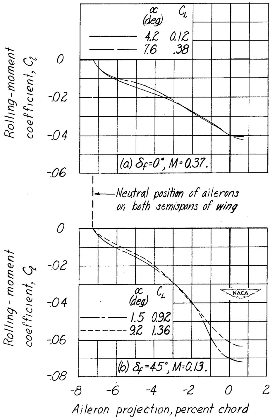
Figure 27.— Variation of rolling-moment coefficient of complete wing with projection of double-walled circular plug aileron on one semispan of NACA 65-210 wing. Neutral position of ailerons: -7.3-percent-chord projection on both semispans of a complete wing. (See reference 4.)
