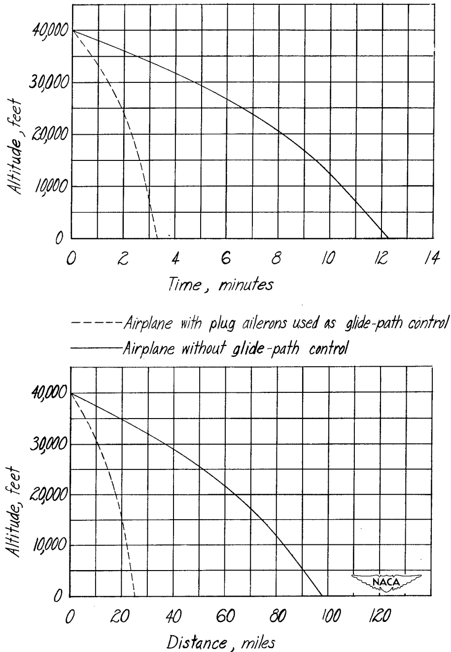
Figure 25.— Comparison of estimated elapsed time and ground distance covered during descent of a typical airplane from an altitude of 40,000 feet with and without a glide-path control. Plug ailerons raised to 8-percent-chord projection on both semispan wings used as glide-path control. (Assumed airplane conditions: wing loading, 63 lb/sq ft; wing aspect ratio, 10.18; wing taper ratio, 0.43; effective propeller thrust, 0; \delta_f = 0^\circ ; M = 0.7 until V_1 = 450 mph is attained.)
