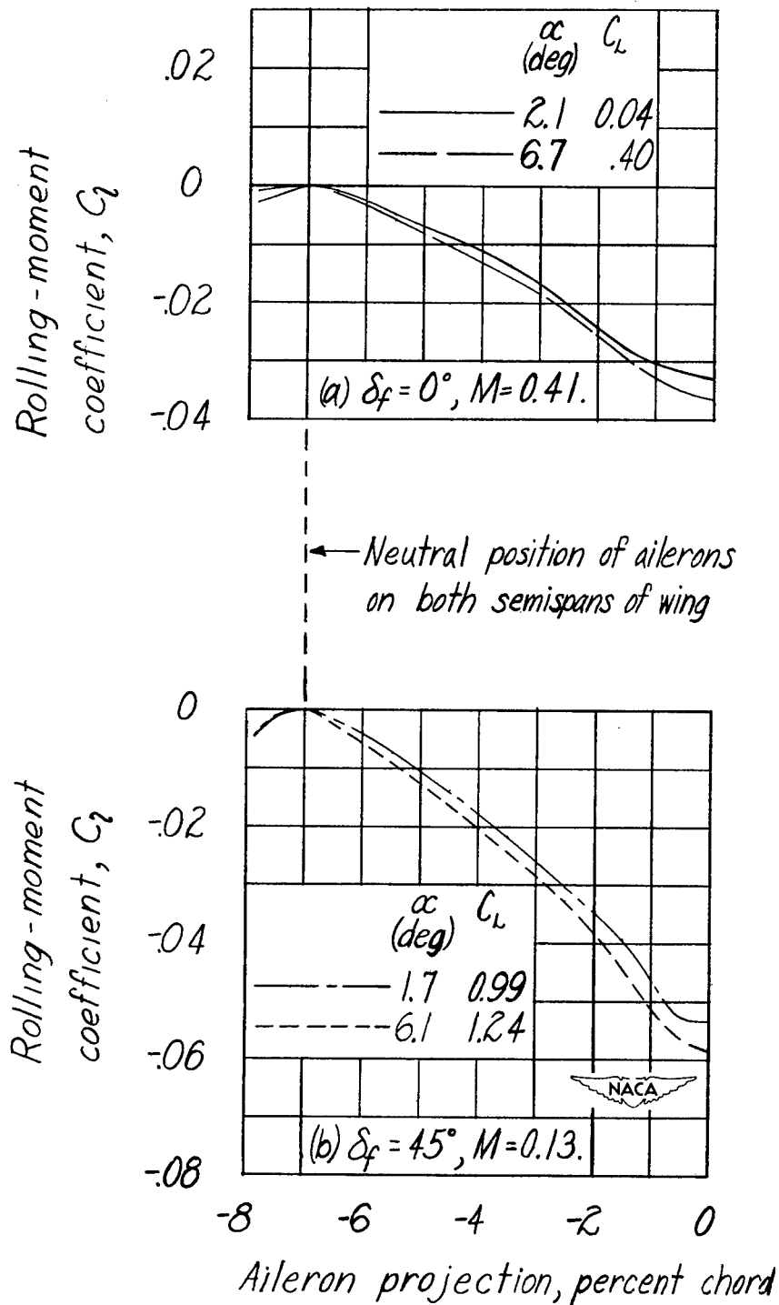
Figure 28.— Variation of rolling-moment coefficient of complete wing with projection of basic retractable aileron on one semispan of NACA 65-210 wing. Neutral position of ailerons: -7.0-percent-chord projection on both semispans of a complete wing. (See reference 3.)
