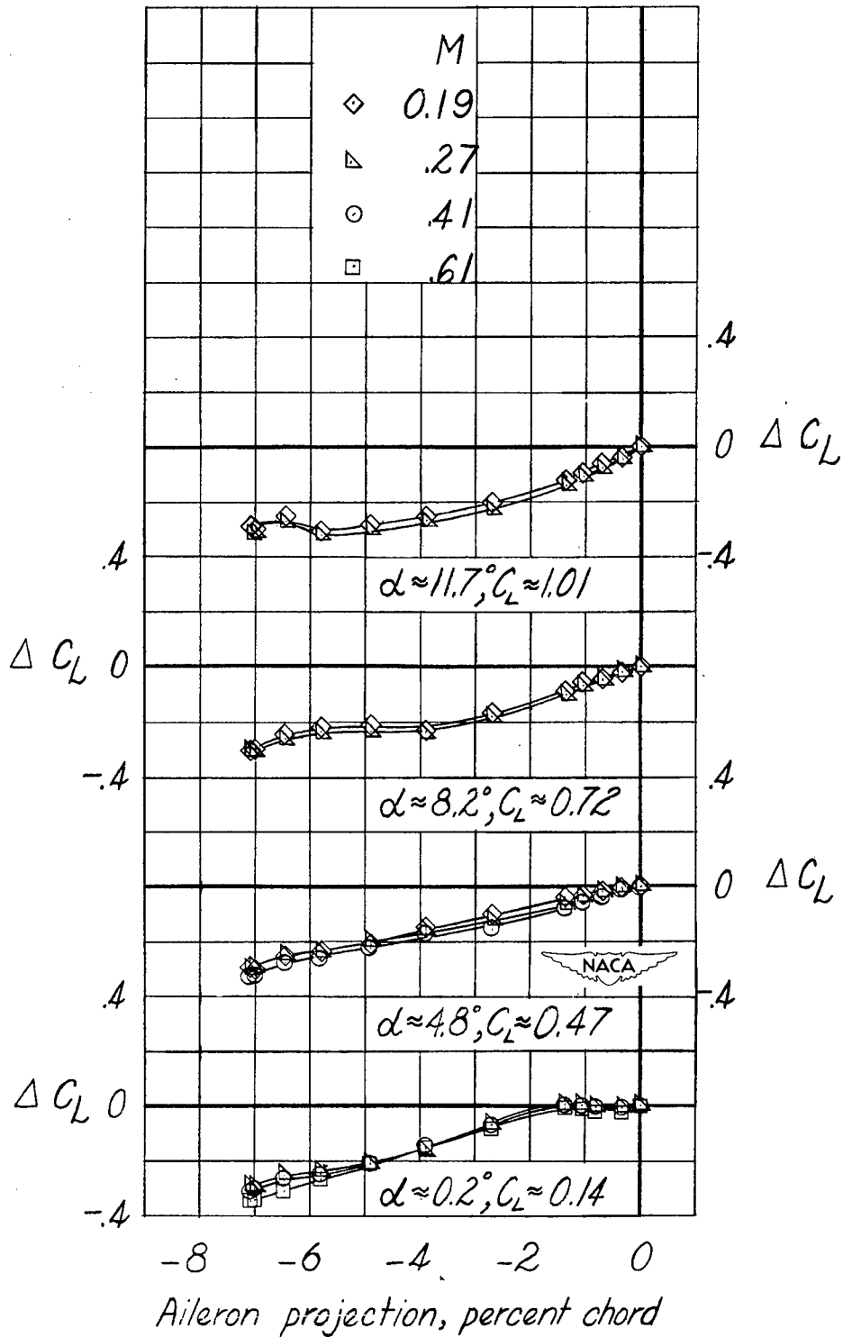
Figure 12.- Incremental values of lift, drag, and pitching-moment coefficients obtained by projection of the thin-plate circular plug aileron on both semispans of the NACA 65-210 wing. Flap retracted.
