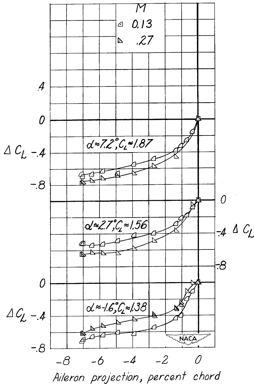
Figure 13.— Incremental values of lift, drag, and pitching-moment coefficients obtained by projection of the thin-plate circular plug aileron on both semispans of the NACA 65-210 wing. Flap deflected 45^\circ .
