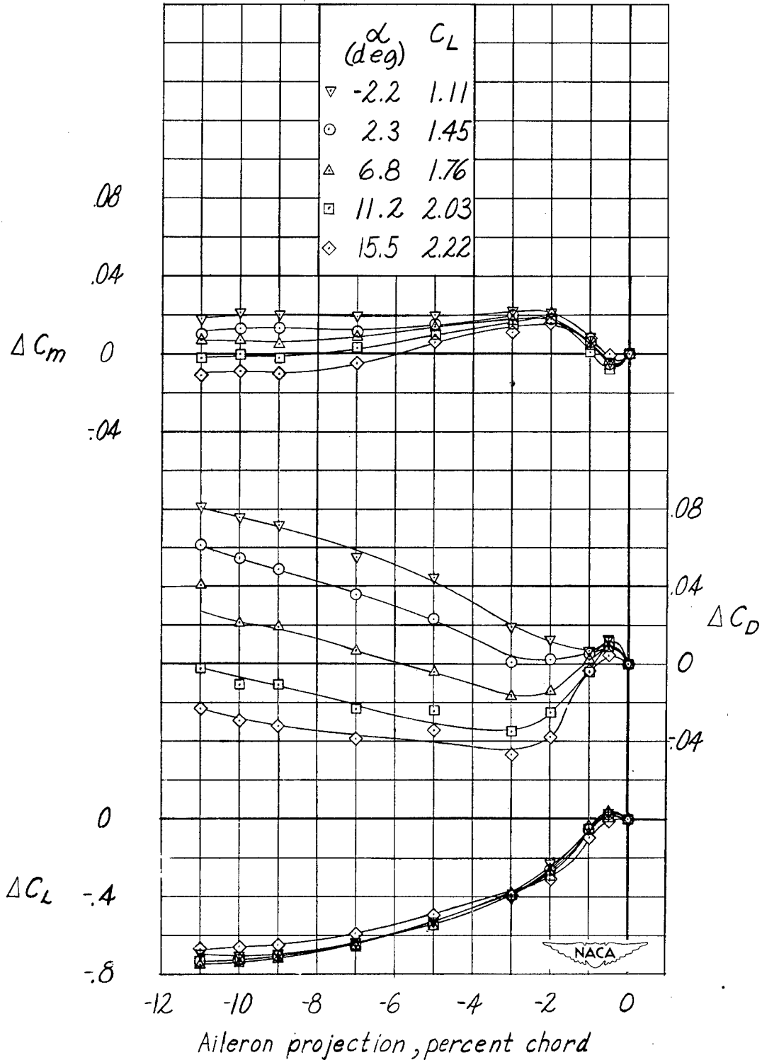
Figure 22.— Incremental values of lift, drag, and pitching-moment coefficients obtained by projection of the retractable aileron on both semispans of the NACA 65 2 -215 wing. Flap deflected 30°; M = 0.13.
