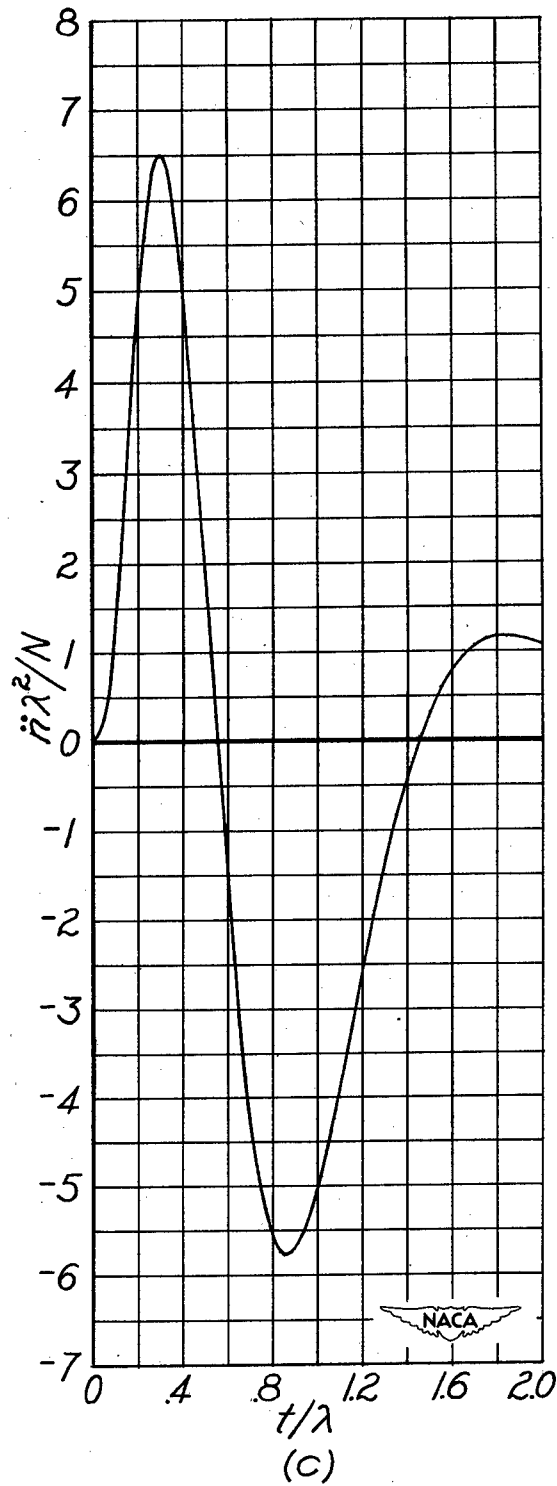
Figure 6.- Variation of incremental-load-factor curves with time ratio.
