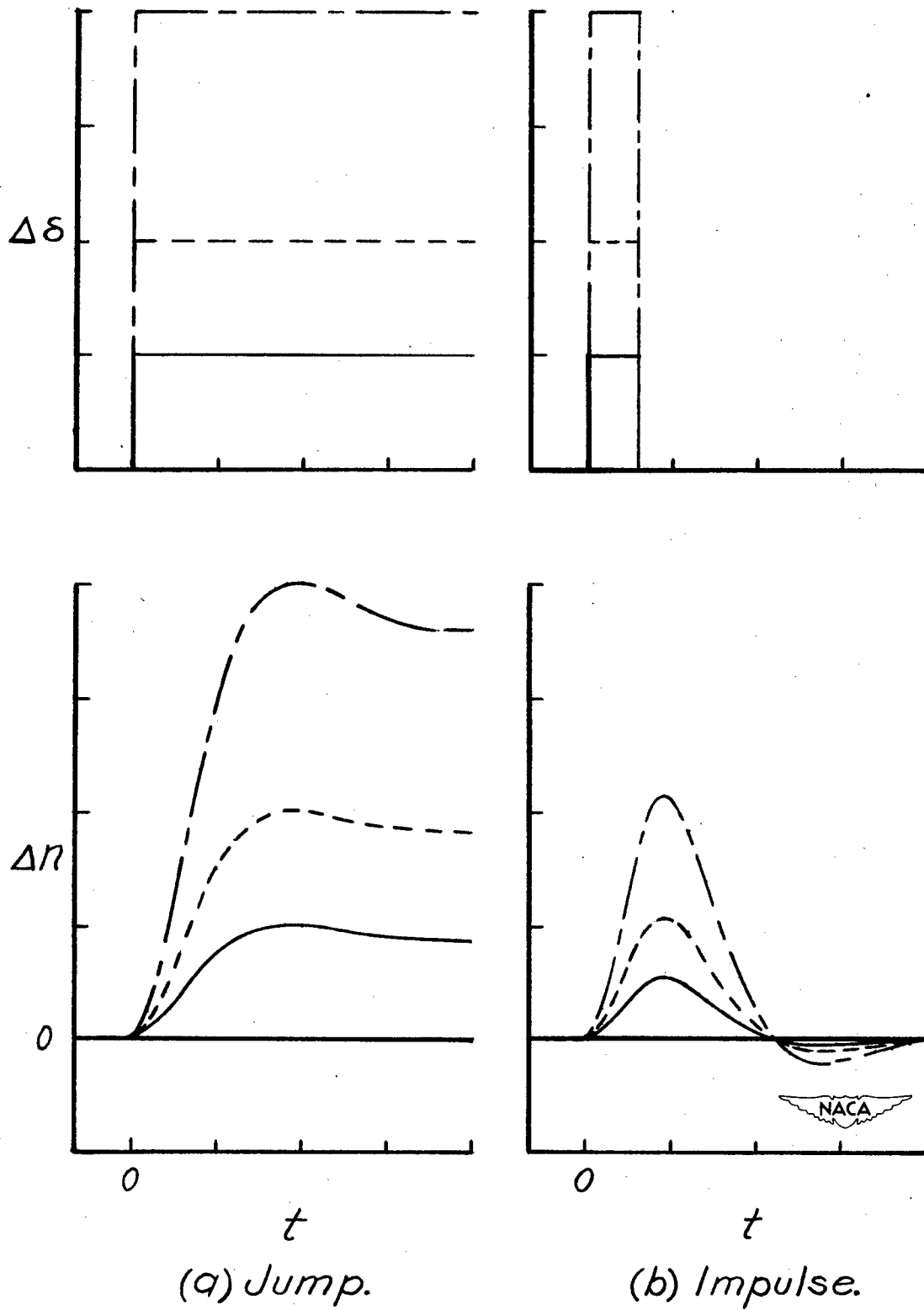
Figure 3.- Incremental-load-factor variations following control movement.
