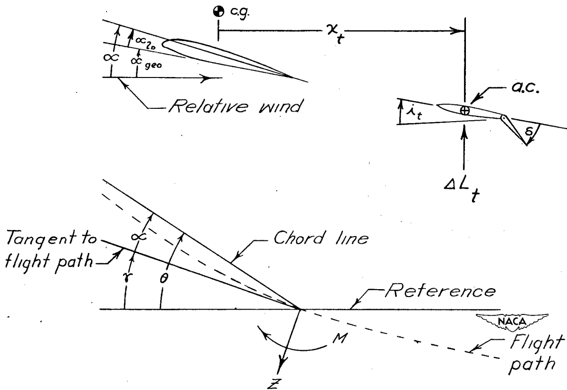
Figure 1.- Sign conventions employed. Positive directions shown.
