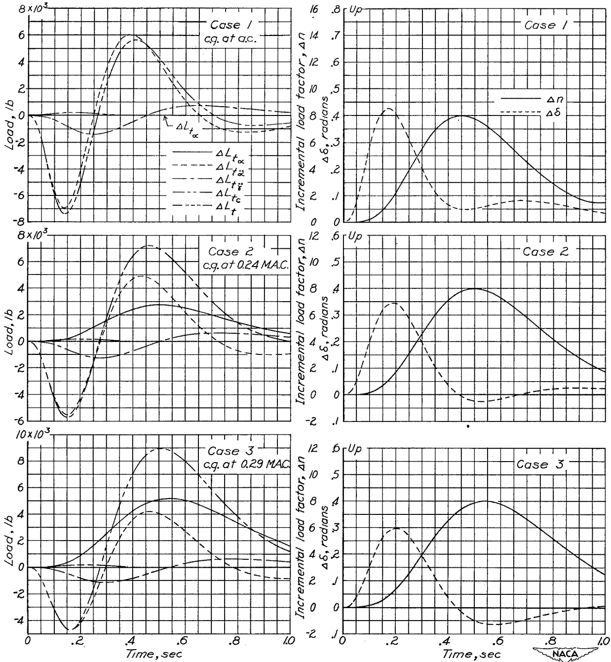
Figure 7.- Effect of center-of-gravity position on incremental-tail-load components.
