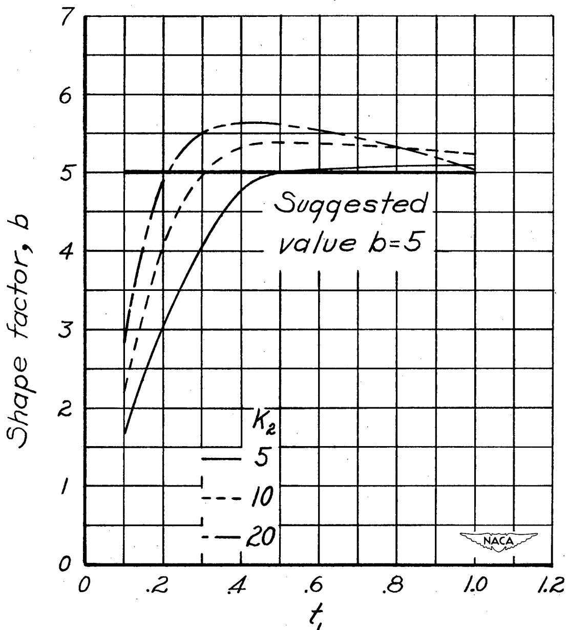
Figure 5.- Variation of shape factor b with t_1 .
