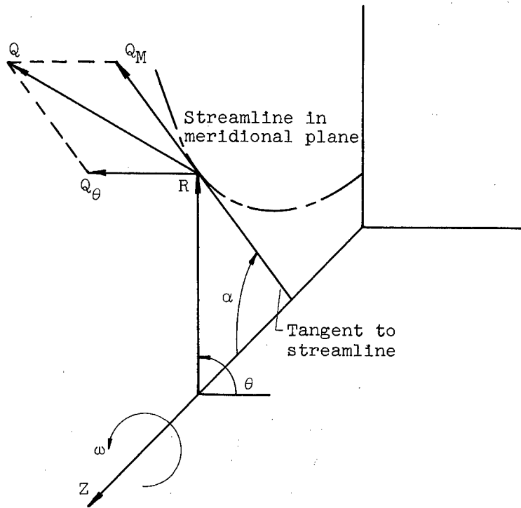
Figure 4. - Coordinates, velocities, and so forth at point on streamline in meridional plane (axial-symmetry solution).
