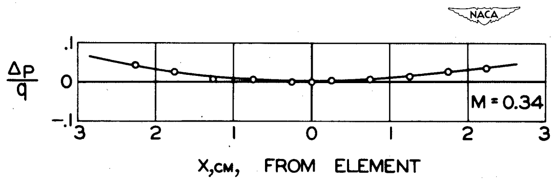
Figure 18.- Representative pressure distributions on flat plate with turbulent layer. Supersonic flow.
