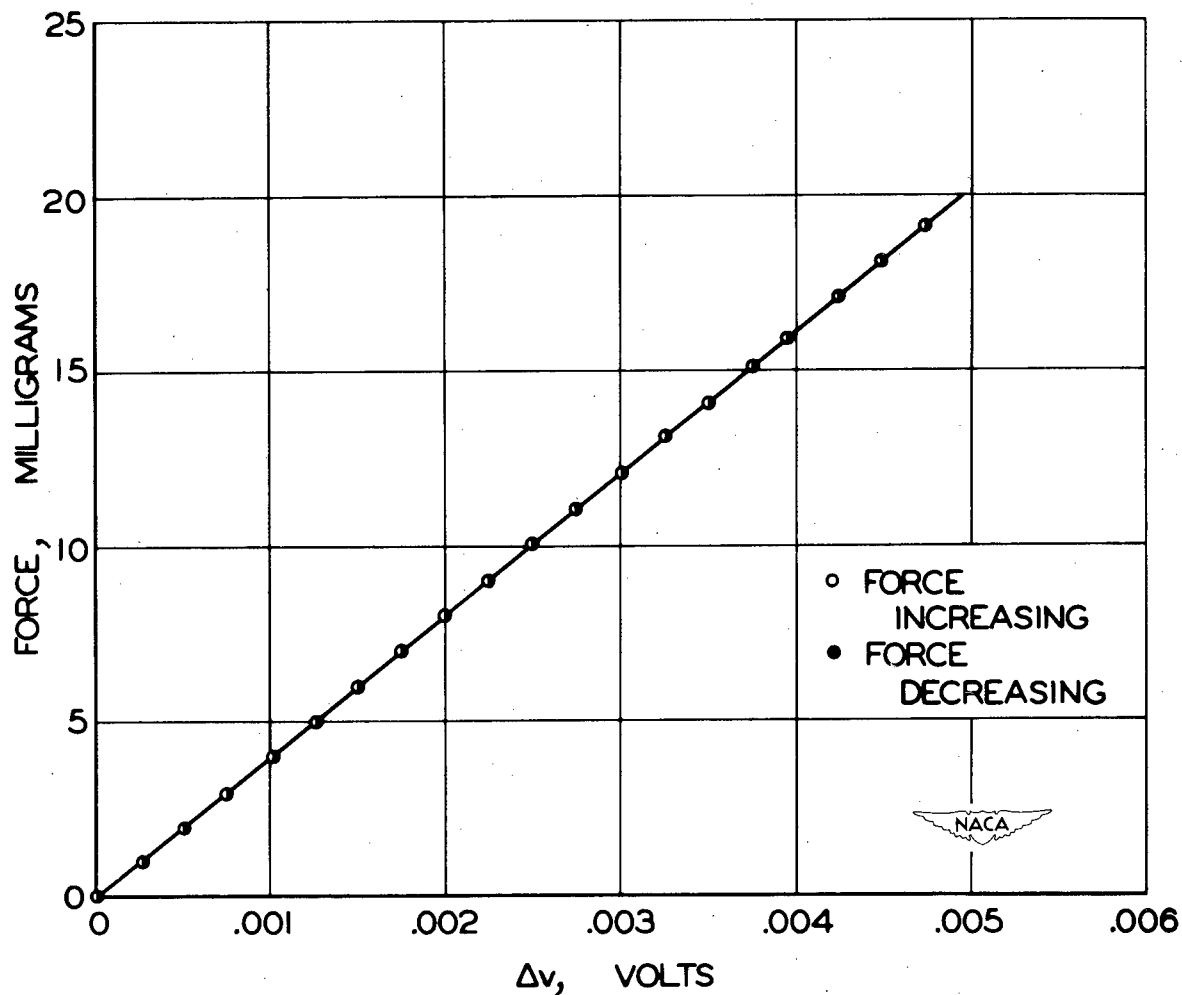
Figure 8.- Calibration of skin-friction instrument. Input, 5 volts at 20 kilocycles; 0.0005- by 1/4-inch links; \tau_0 , 39.25 \times \Delta v dynes per square centimeter.
