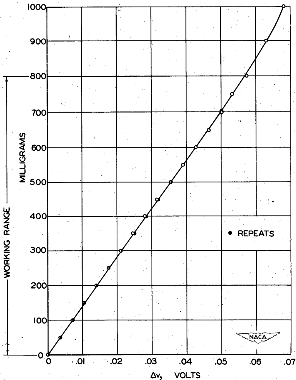
Figure 9.- Calibration curve of skin-friction instrument. 0.01- by 1/16-inch steel links; \tau_0 , 38.3 \times 10^3 \times \Delta v dynes per square centimeter.
