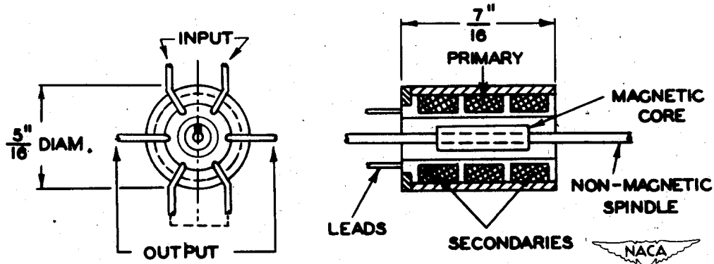
Figure 4.- Differential transformer.
