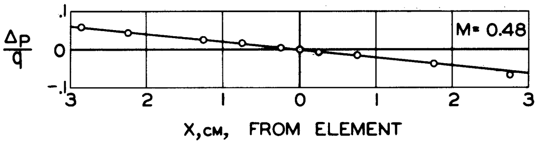
Figure 20.- Representative pressure distributions on flat plate with laminar boundary layer. Subsonic flow.
