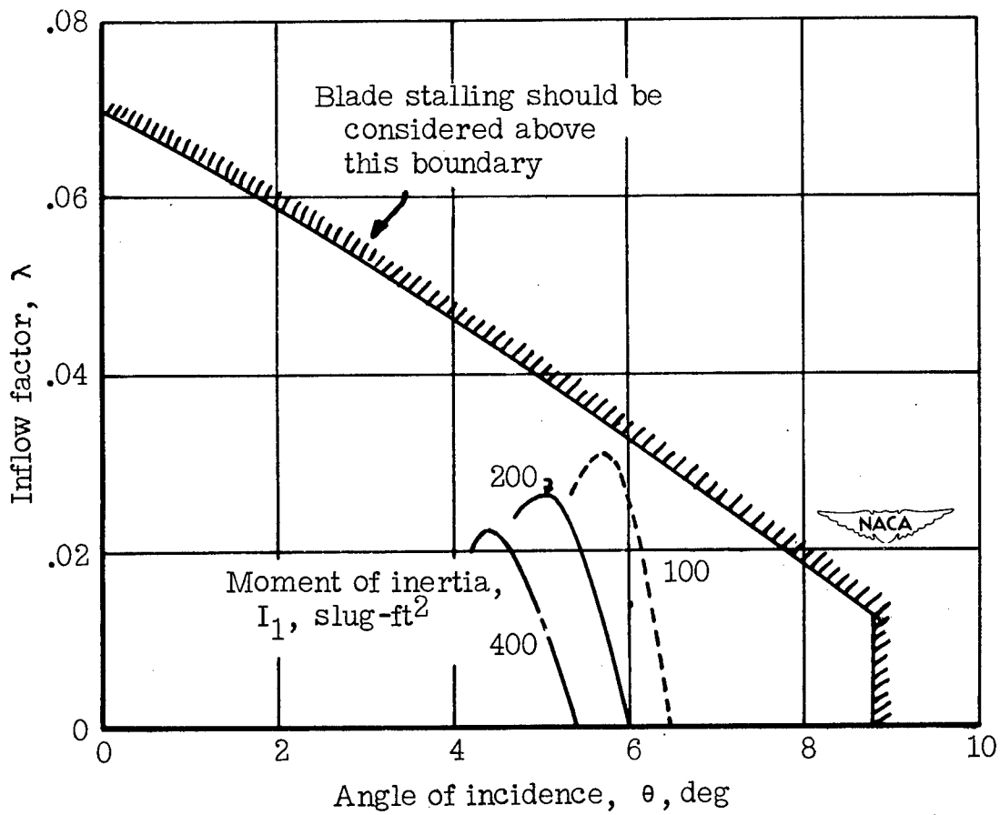
Figure 8.- Effect of blade moment of inertia on \lambda against \theta throughout the transition maneuver. Slow exponential pitch change.
