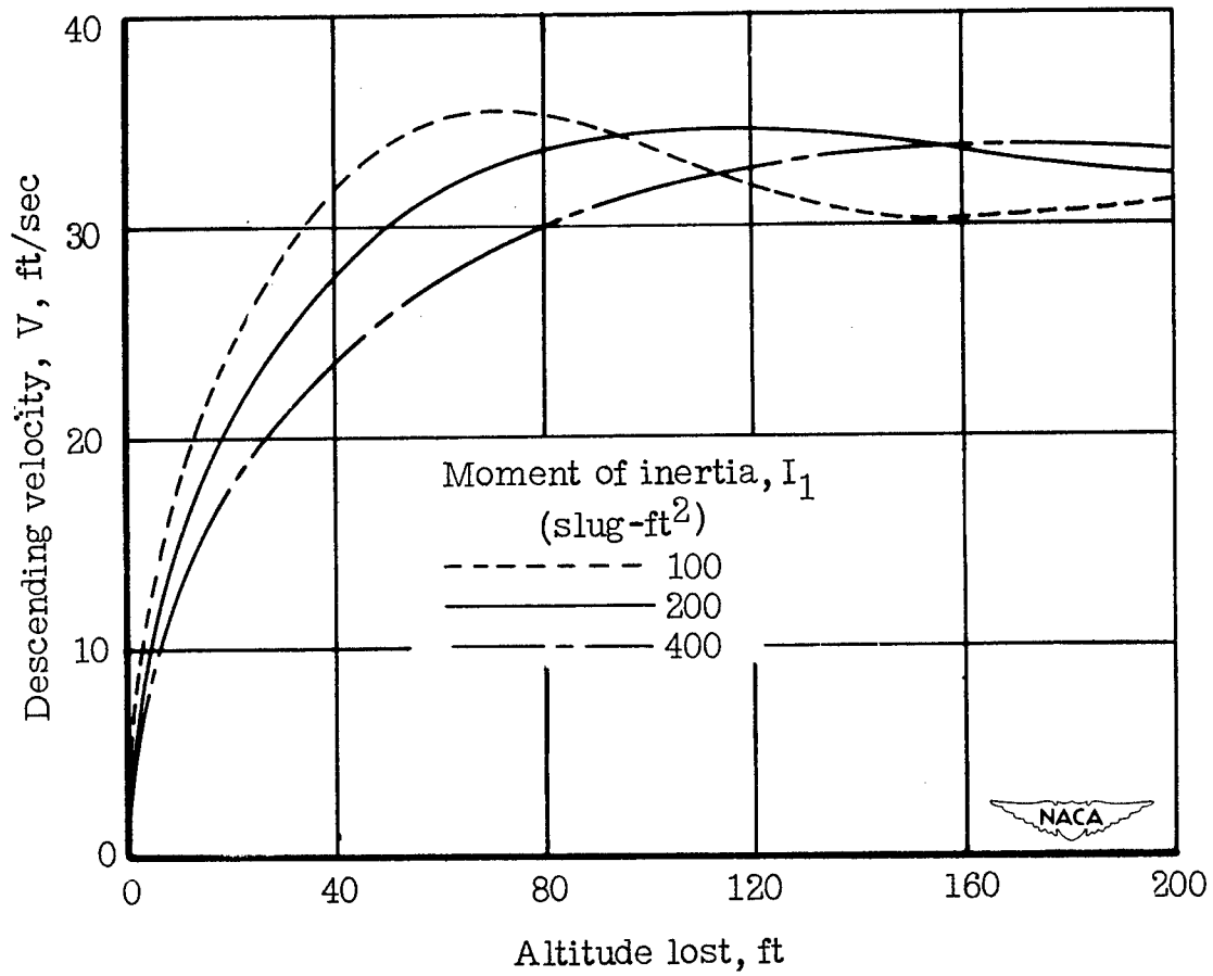
Figure 10.- Effect of blade moment of inertia on descending velocity against altitude lost. Slow exponential pitch change.
