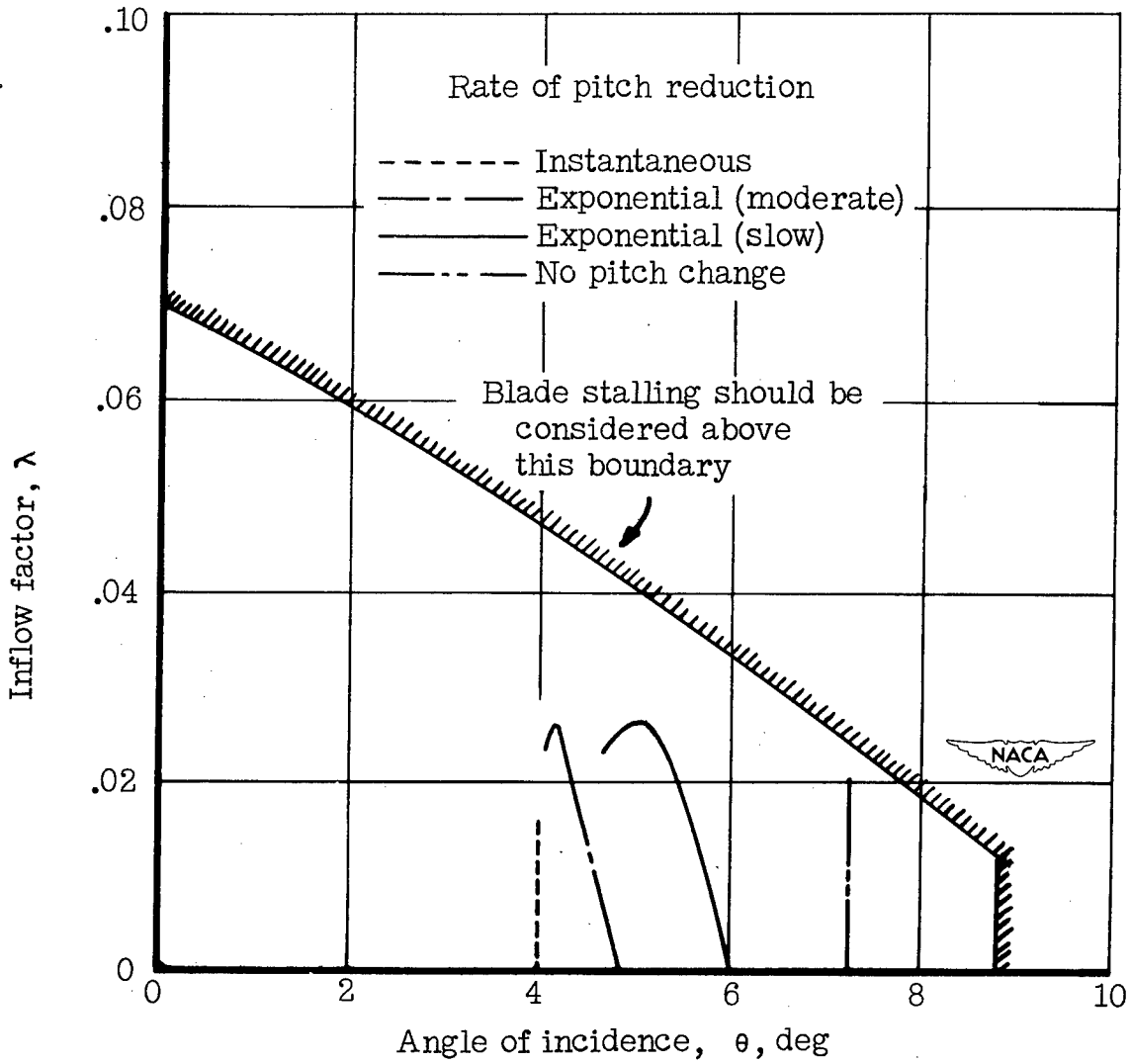
Figure 7.- Effect of rate of pitch reduction on \lambda against \theta throughout the transition maneuver. I_1 = 200 slug-feet 2 .
