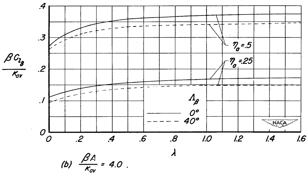
Figure 12.- Aileron rolling-moment-coefficient parameter \frac{\beta C_{l_{\beta}}}{K_{av}} , per radian, for outboard ailerons as a function of aspect ratio parameter, taper ratio, and compressible sweep parameter.
