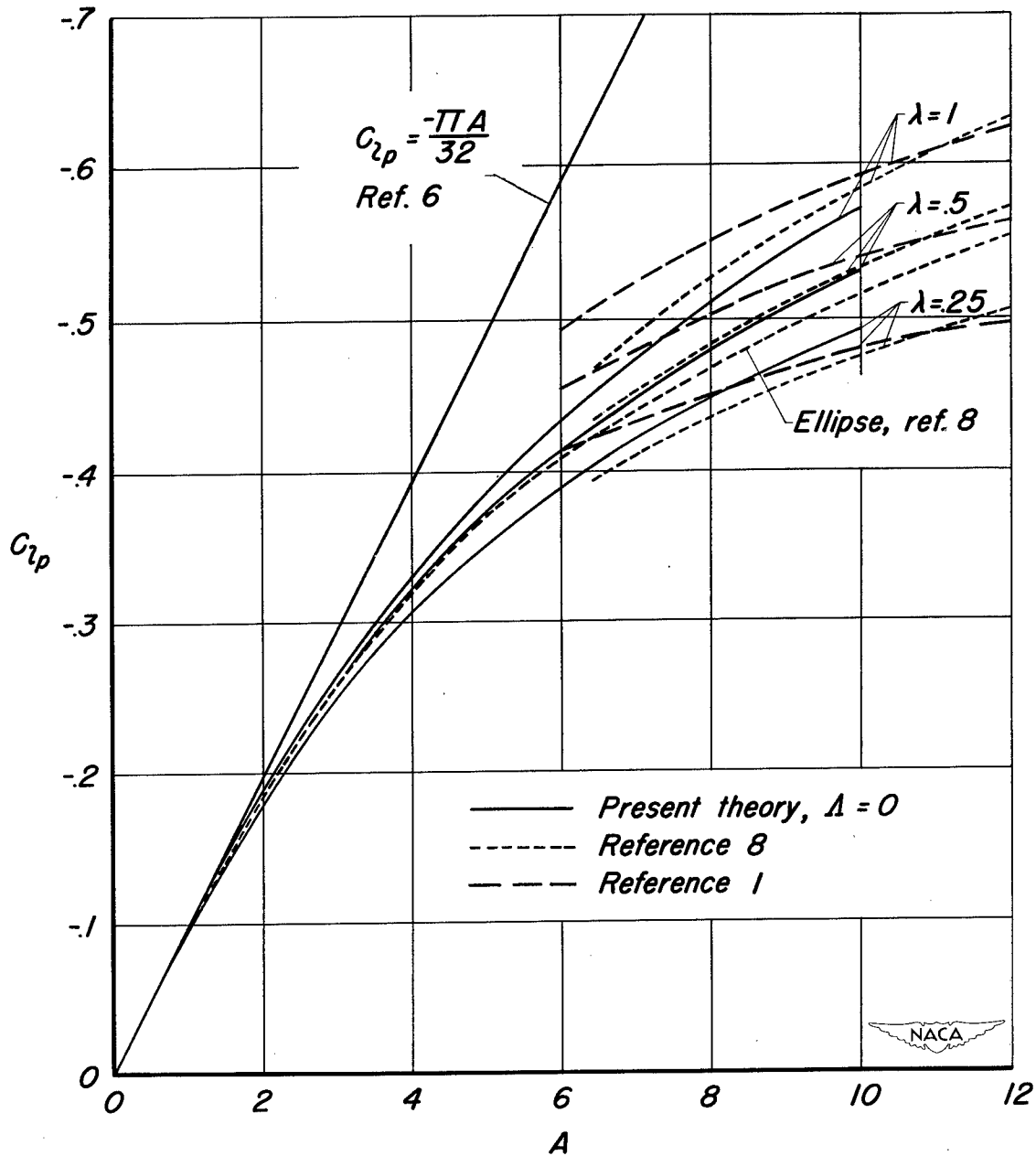
Figure 14.- Comparison of damping-in-roll coefficient C_{lp} of the present theory with those of the theories of references 1, 6, and 8.
