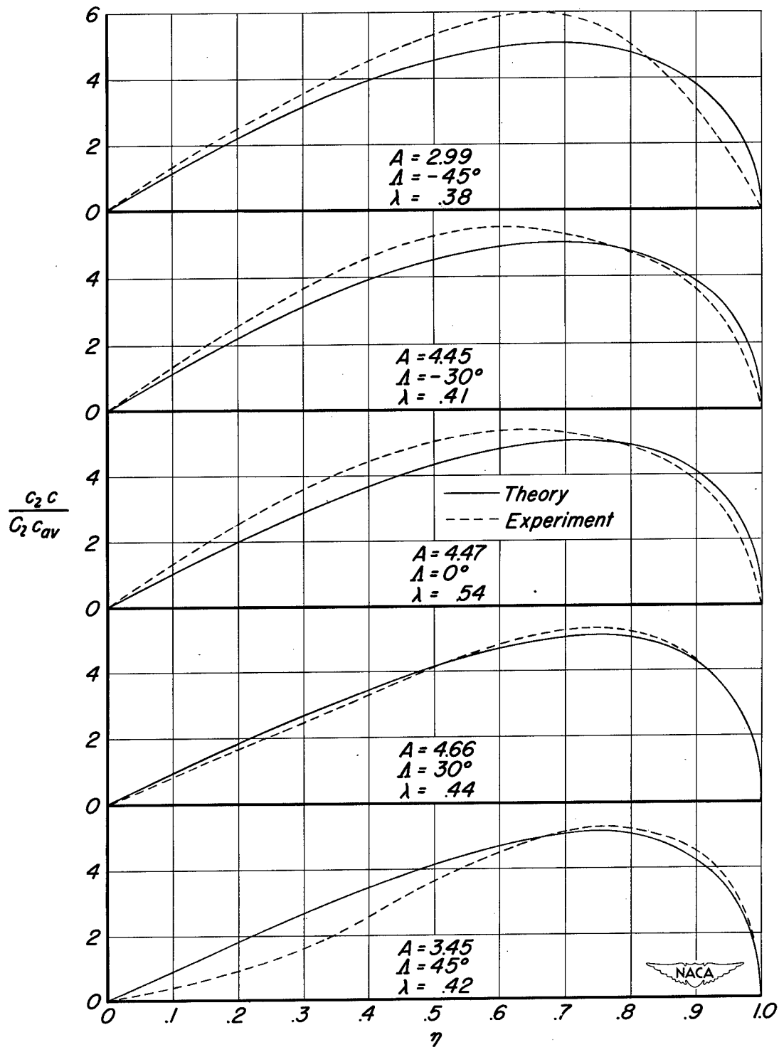
Figure 16.—Comparisons of theoretical and low-speed experimental spanwise loading coefficients \frac{C_2 C}{C_2 C_{av}} due to rolling of various swept wings.
