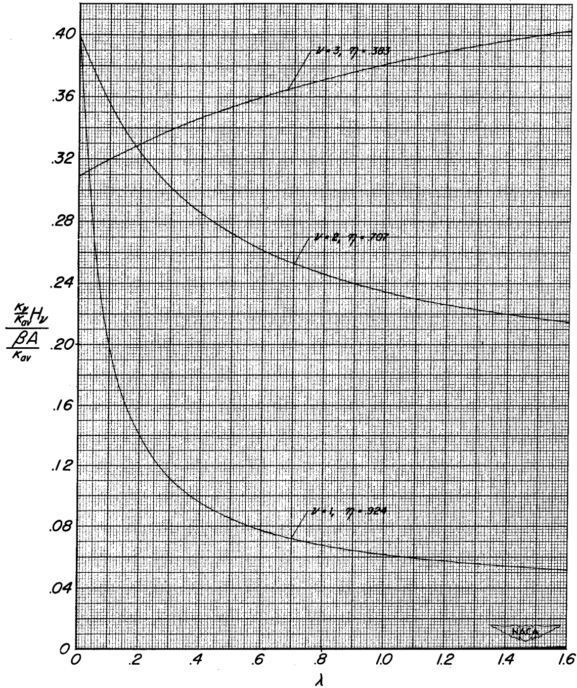
Figure 2.- Variation of the geometric parameter \frac{K_v H_v}{\frac{BA}{K_{av}}} with taper ratio \lambda for straight-tapered wings.
