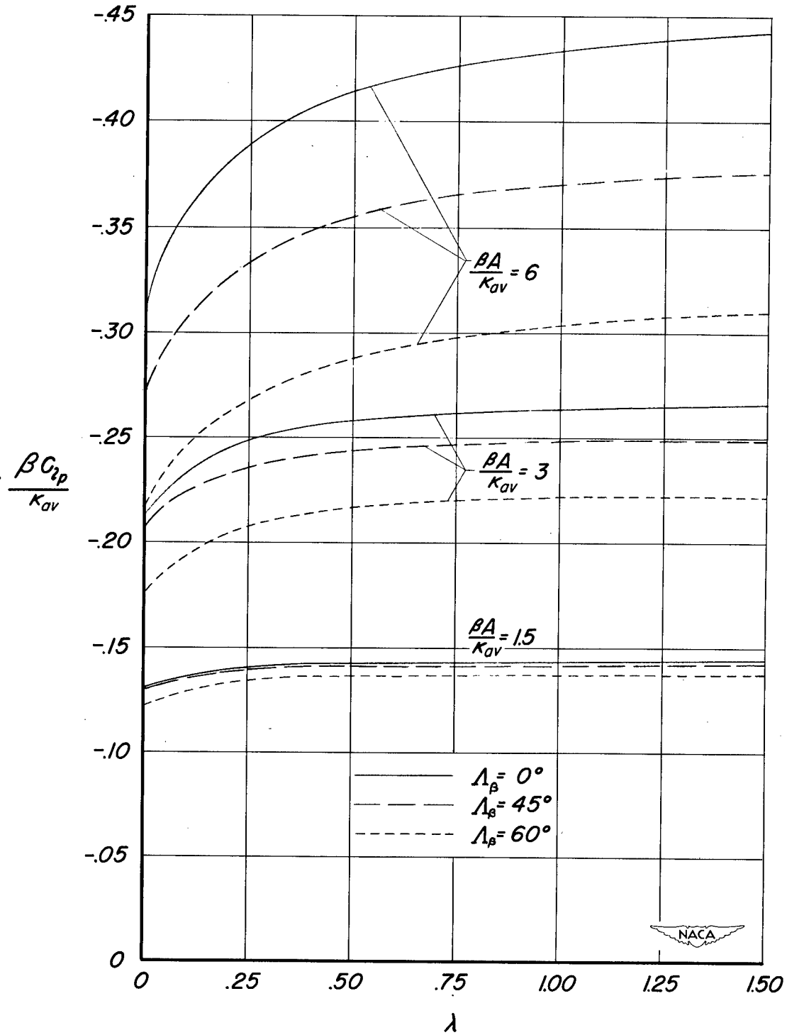
Figure 10.—Variation of the damping-in-roll parameter \frac{\beta C_{2p}}{K_{av}} with taper ratio for wings with various aspect ratio and sweep angle parameters.
