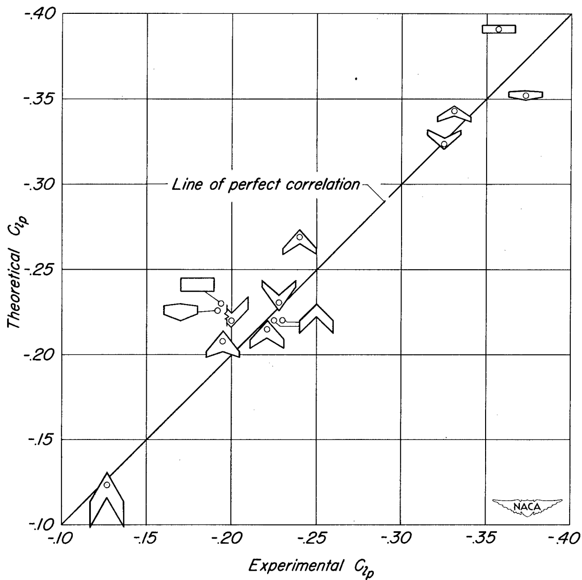
Figure 15.- Correlation of theoretical and low-speed experimental damping-in-roll coefficient C_{ip} for various plan forms.
