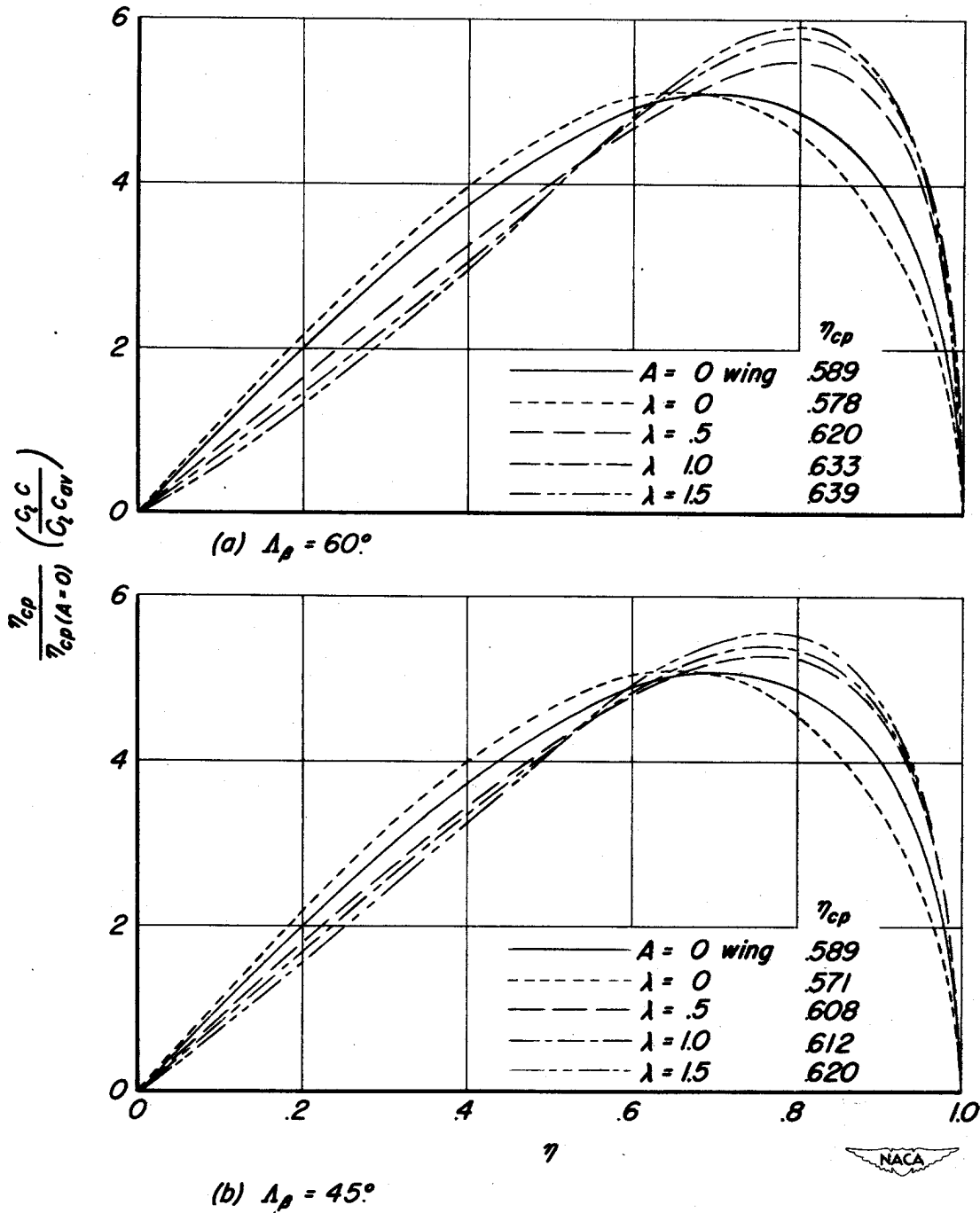
Figure 8.- Spanwise loading due to rolling of wings with various taper ratio and sweep angle parameters of aspect ratio parameter \frac{\beta A}{\kappa_{av}} = 4 . The curve for A=0 serves as a basis for comparison and the factor \frac{\eta_{cp}}{\eta_{cp}(A=0)} gives the curves constant area equal to 3.454.
