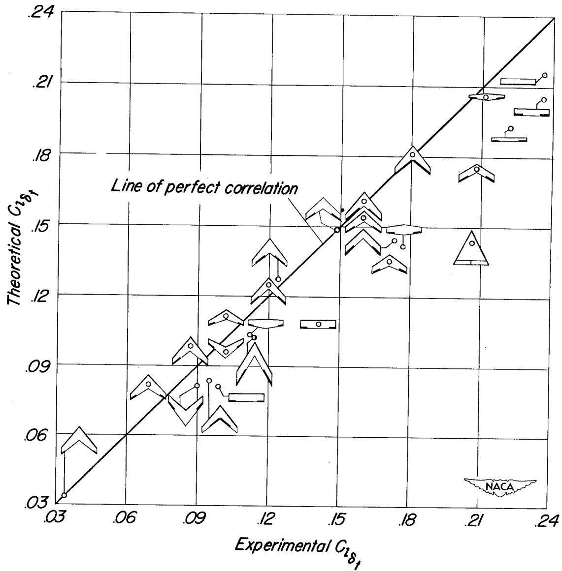
Figure 17.-Correlation of theoretical and low-speed experimental aileron-effectiveness C_{l\delta_1} , per radian, due to two antisymmetrically deflected ailerons, for various plan forms.
