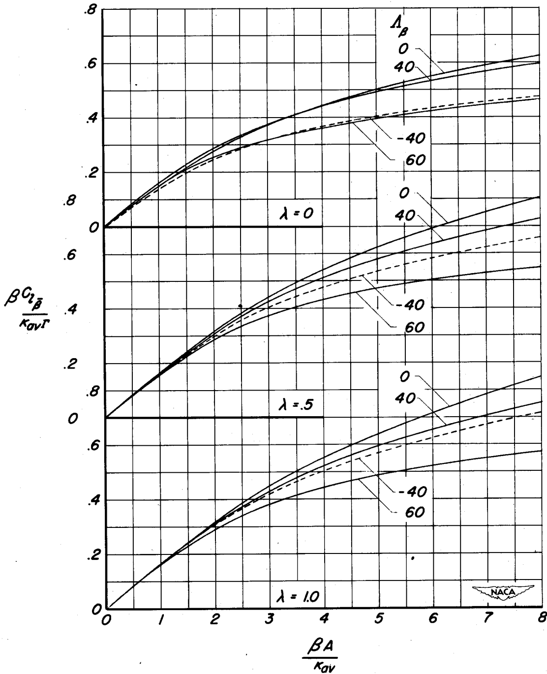
Figure 7.- Rolling moment due to sideslip of wing with dihedral \frac{\beta C_{l\beta}}{\kappa_{av}\Gamma} , per radian squared, for unit constant spanwise dihedral angle for straight-tapered wings.
