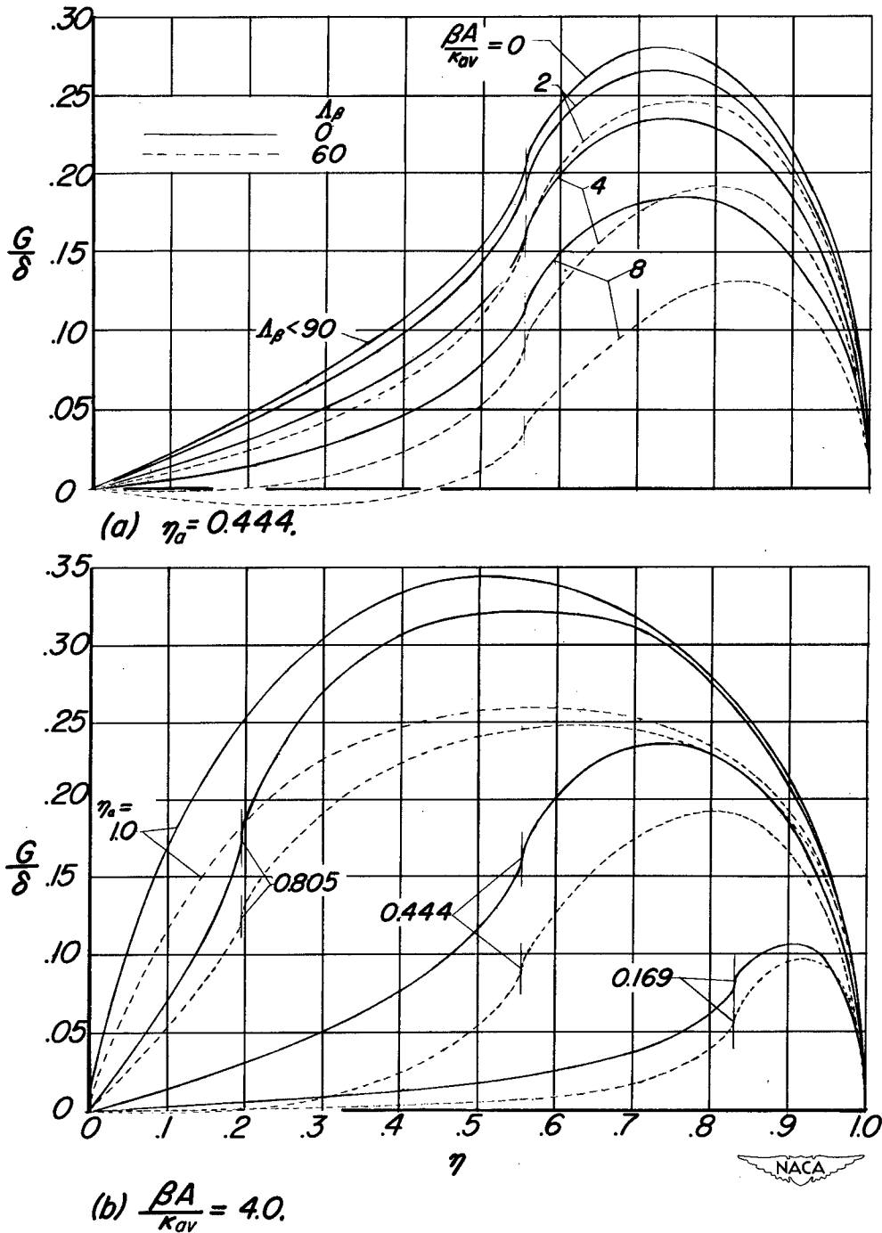
Figure II.-Antisymmetric spanwise loading distribution due to deflection of outboard ailerons, for c_a=c , on wings having a taper ratio of 0.5.
