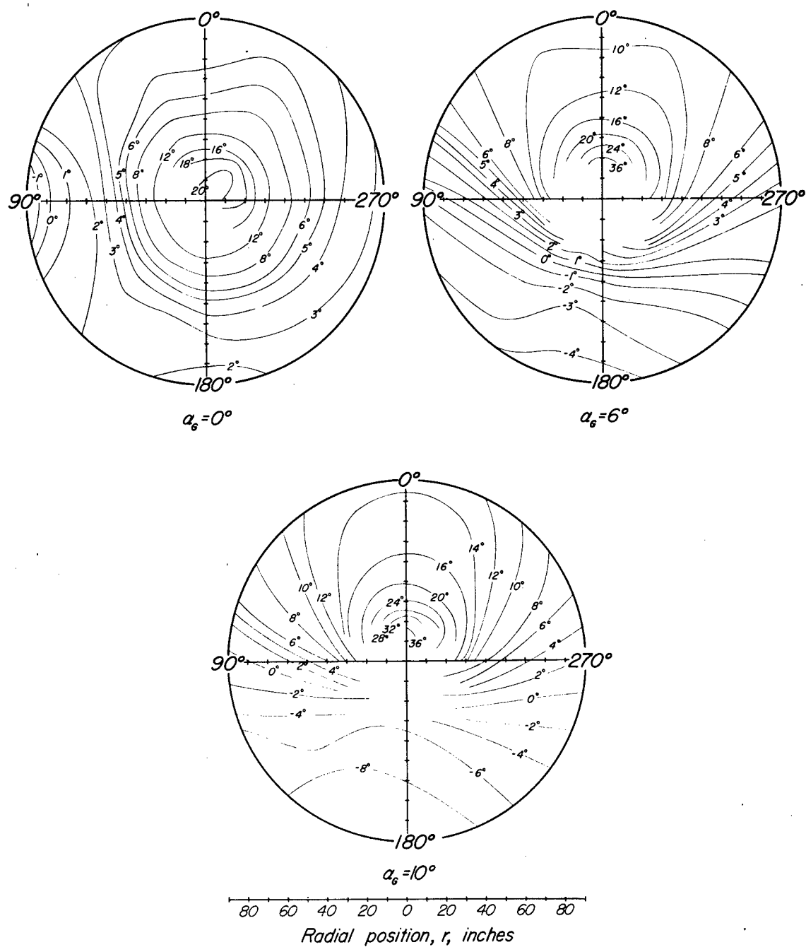
Figure 19.—Contours of the angle of outflow, \theta , at the survey disk for several angles of attack. m_1/m_0 , 0.29; \delta_r , 0^\circ .
