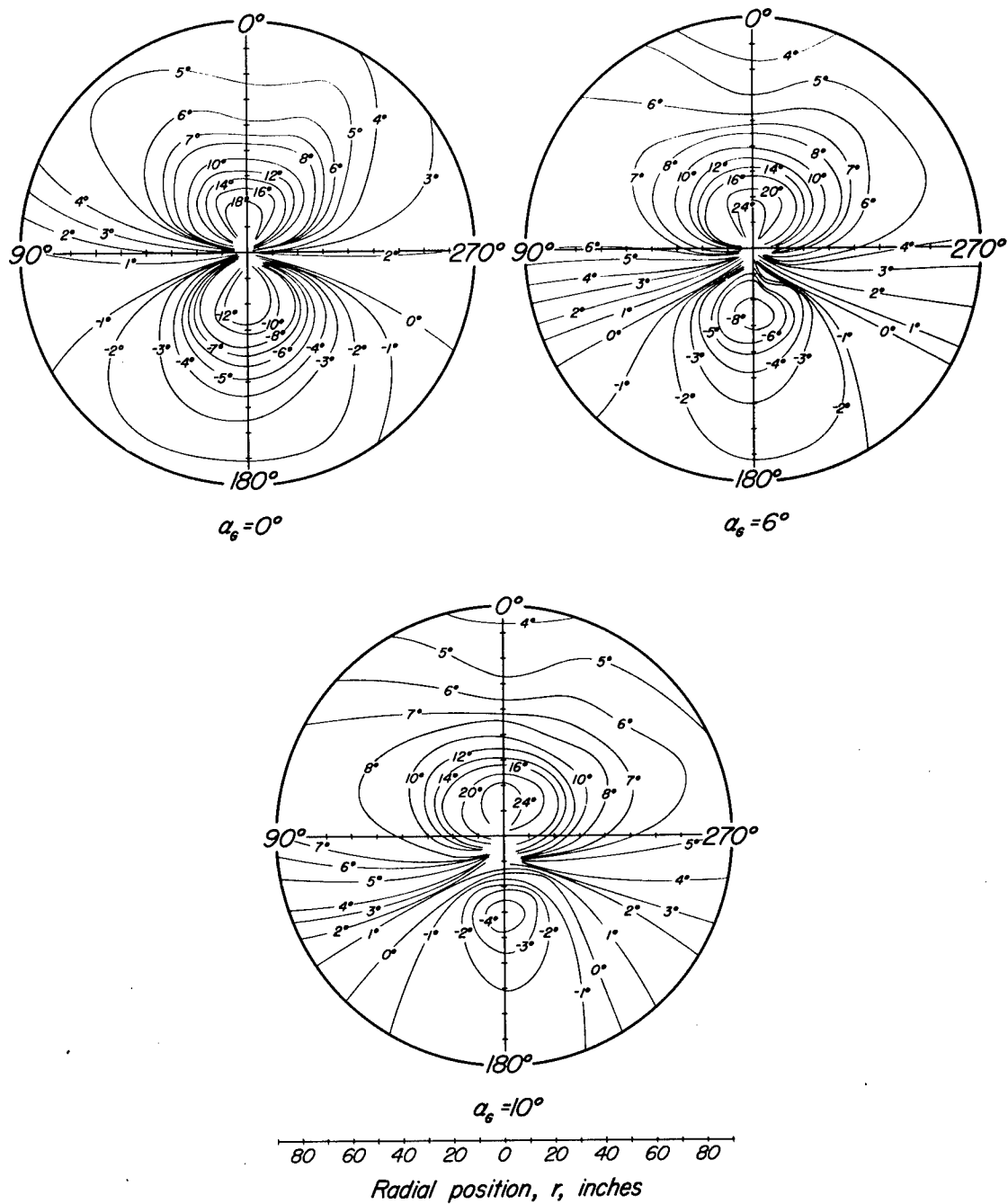
Figure 21.- Contours of the angle of upwash, \epsilon , at the survey disk for several angles of attack. m_t/m_o , 0.29; \delta_t , 0^\circ .
