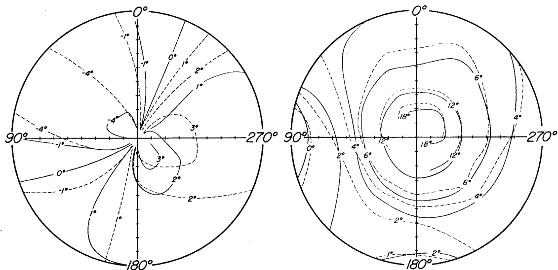
(b) Angle of outflow, \theta , deg.
