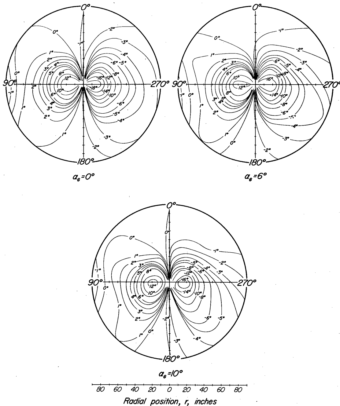
Figure 22.- Contours of the angle of sidewash, \sigma , at the survey disk for several angles of attack. m_1/m_0 , 0.29; \delta_f , 0^\circ .
