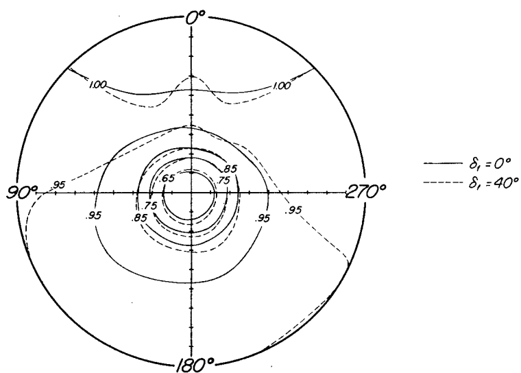
(c) Velocity ratio, V_1/V_0 .
