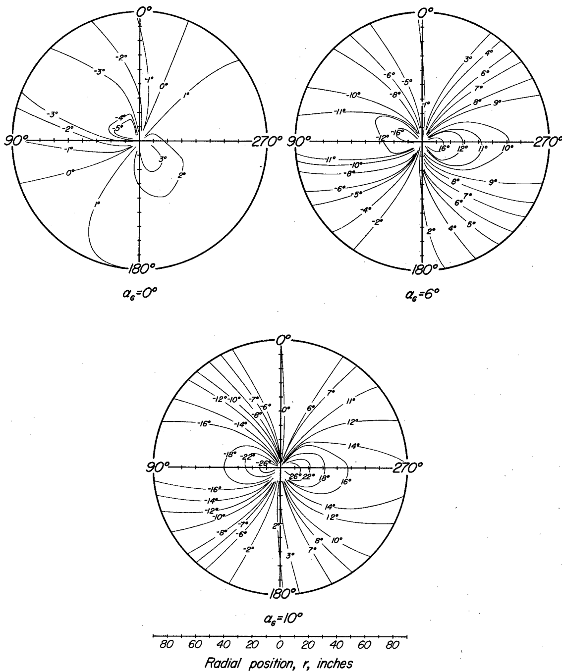
Figure 18.—Contours of the angle of rotational flow, \psi , at the survey disk for several angles of attack. m_1/m_0 , 0.29; \delta_f , 0^\circ .
