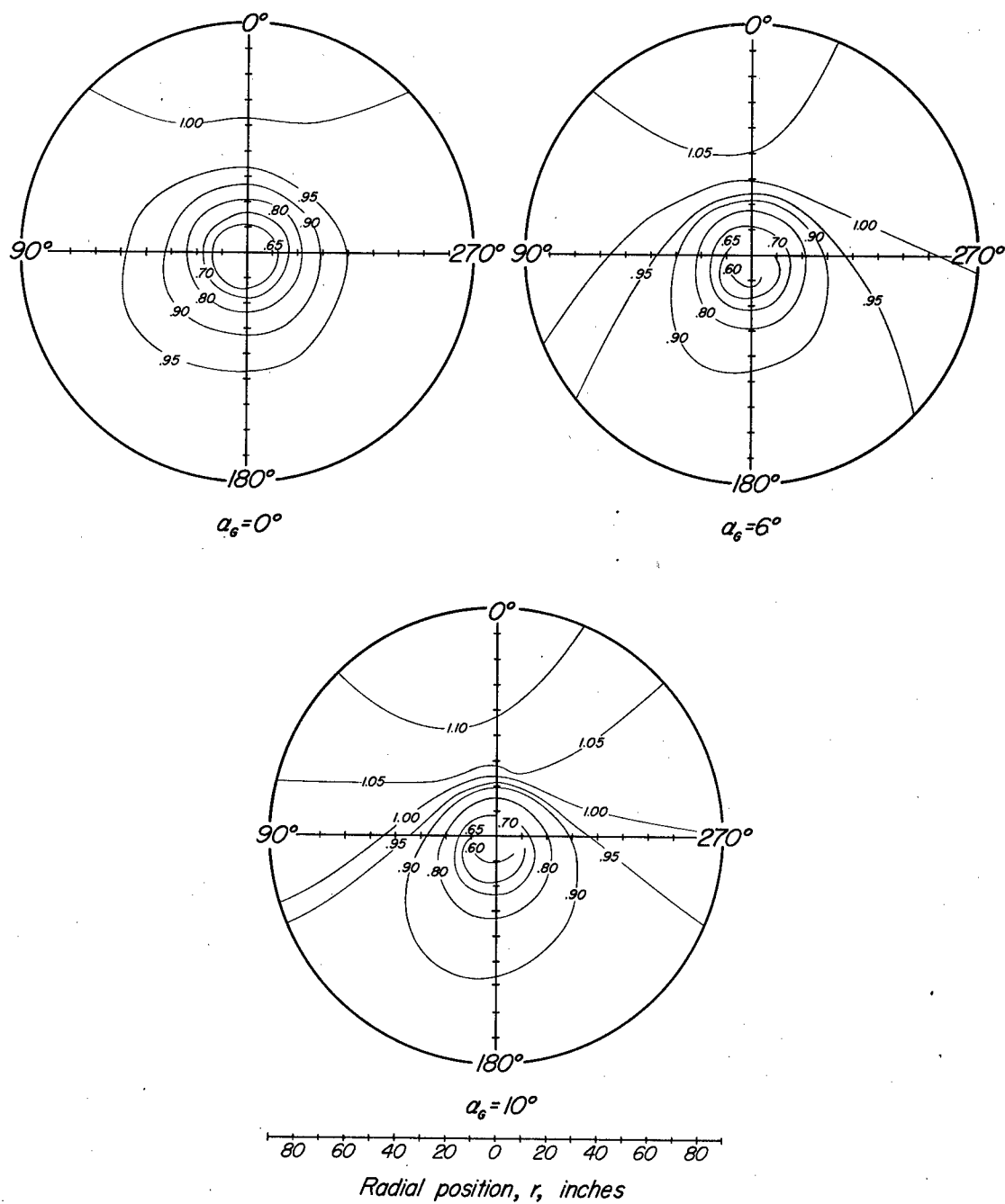
Figure 2Q.- Contours of the velocity ratio, V_t/V_o , at the survey disk for several angles of attack. m_t/m_o , 0.29; \delta_t , 0^\circ .
