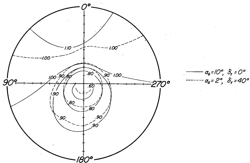
(c) Velocity ratio, V_1/V_0
