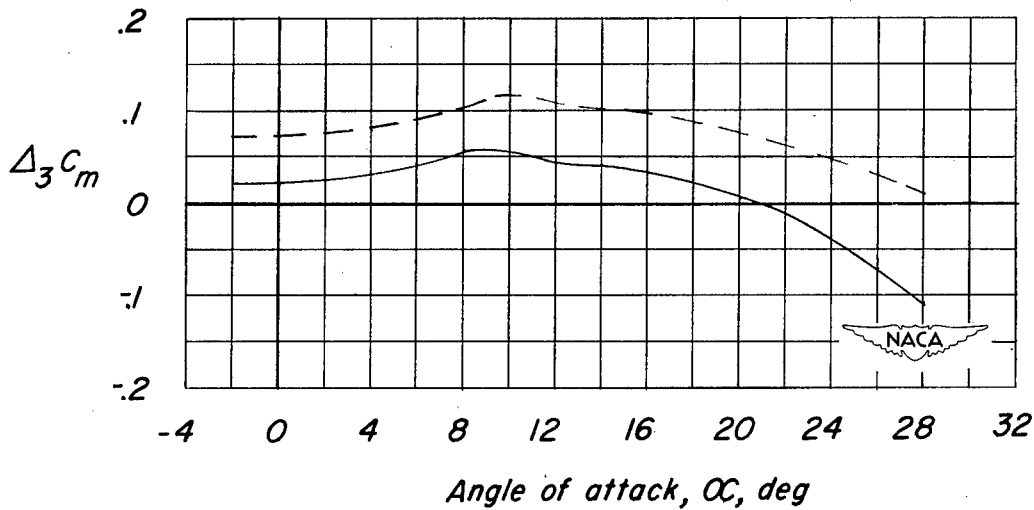
Figure 10.- Variation with angle of attack of the fuselage interference increment \Delta_3 C_m for the unswept and 45° sweptback fuselage-tail configurations.
