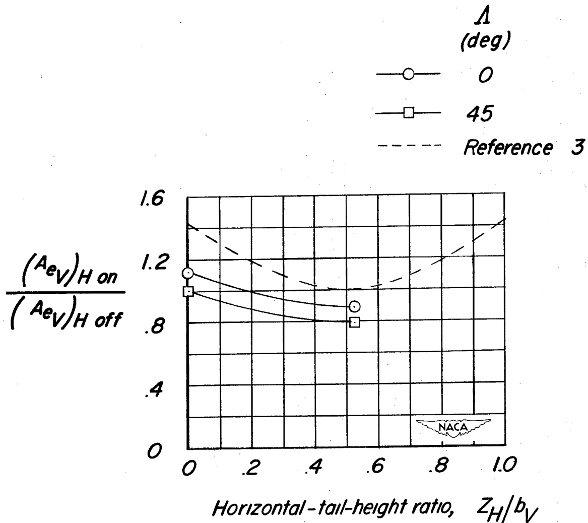
Figure 21.- Variation of the ratio \frac{(Ae_V)_{H \text{ on}}}{(Ae_V)_{H \text{ off}}} with horizontal-tail-height ratio Z_H/b_V for the unswept and 45^\circ sweptback tails. \alpha_H = 0^\circ ; wing off.
