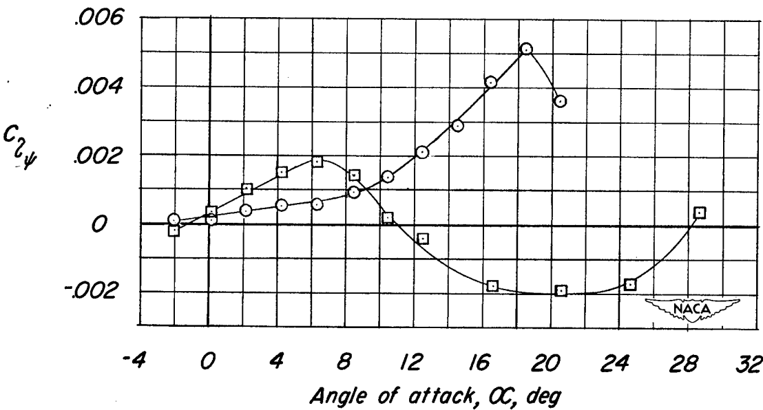
Figure 14.- Static lateral stability characteristics of the unswept and 45° sweptback wings.
