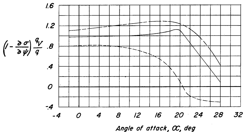
Figure 28.- Effects of wing position on the variation of the average efficiency factor (fig. 27) with angle of attack for the unswept and 45° sweptback configurations.
