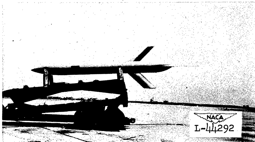
(b) Sweptback plan form.
