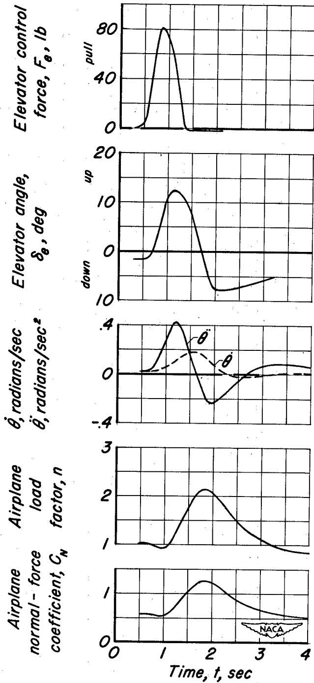
Figure 15.- Time history of pertinent quantities during pull-up maneuver; airspeed, 164 miles per hour; altitude, 20,400 feet.
