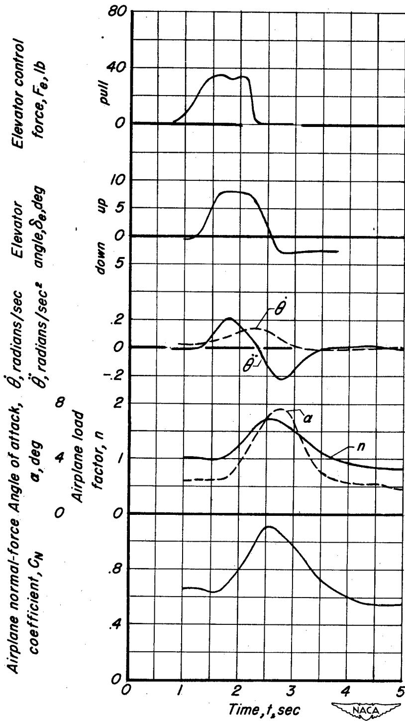
Figure 8.—Time history of pertinent quantities measured during pull-up maneuver; airspeed, 155 miles per hour; altitude, 5300 feet.
