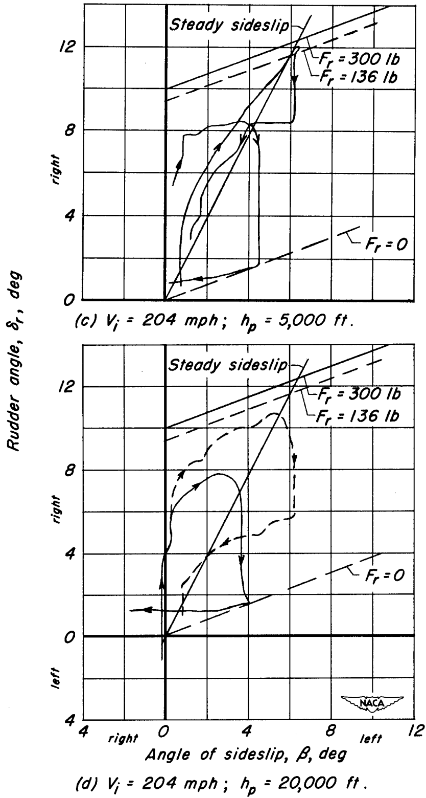
Figure 49.- Concluded.
