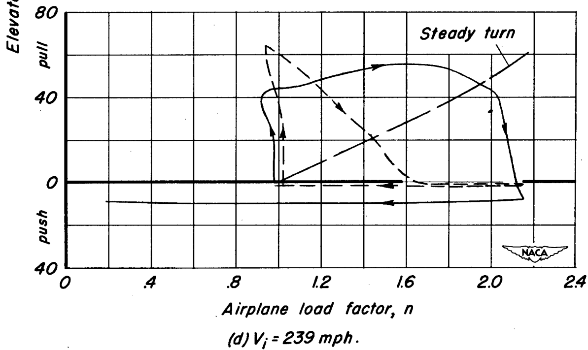
Figure 19.- Continued.
