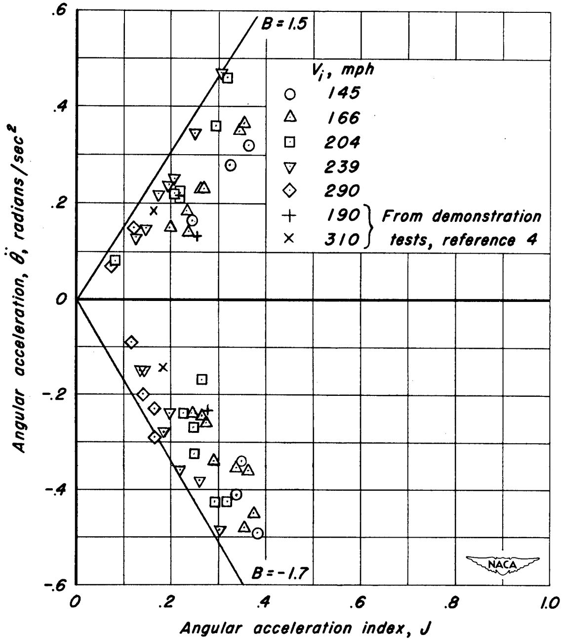
Figure 27.— Evaluation of method of reference 5 for estimating maximum angular accelerations.
