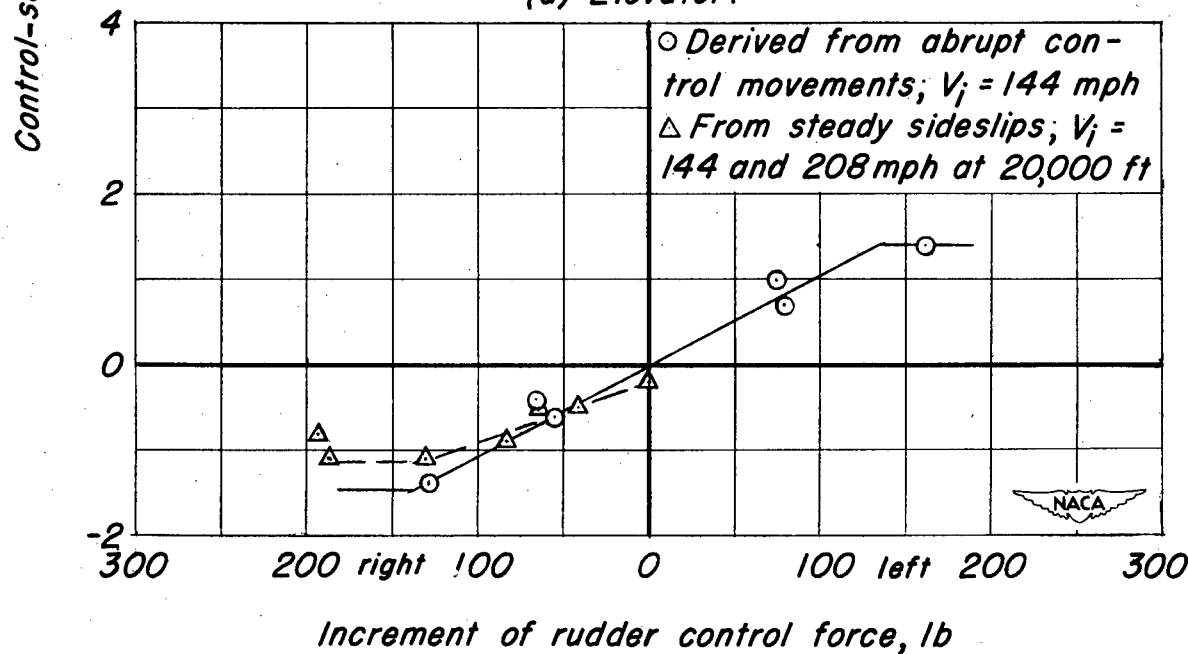
(b) Rudder.
