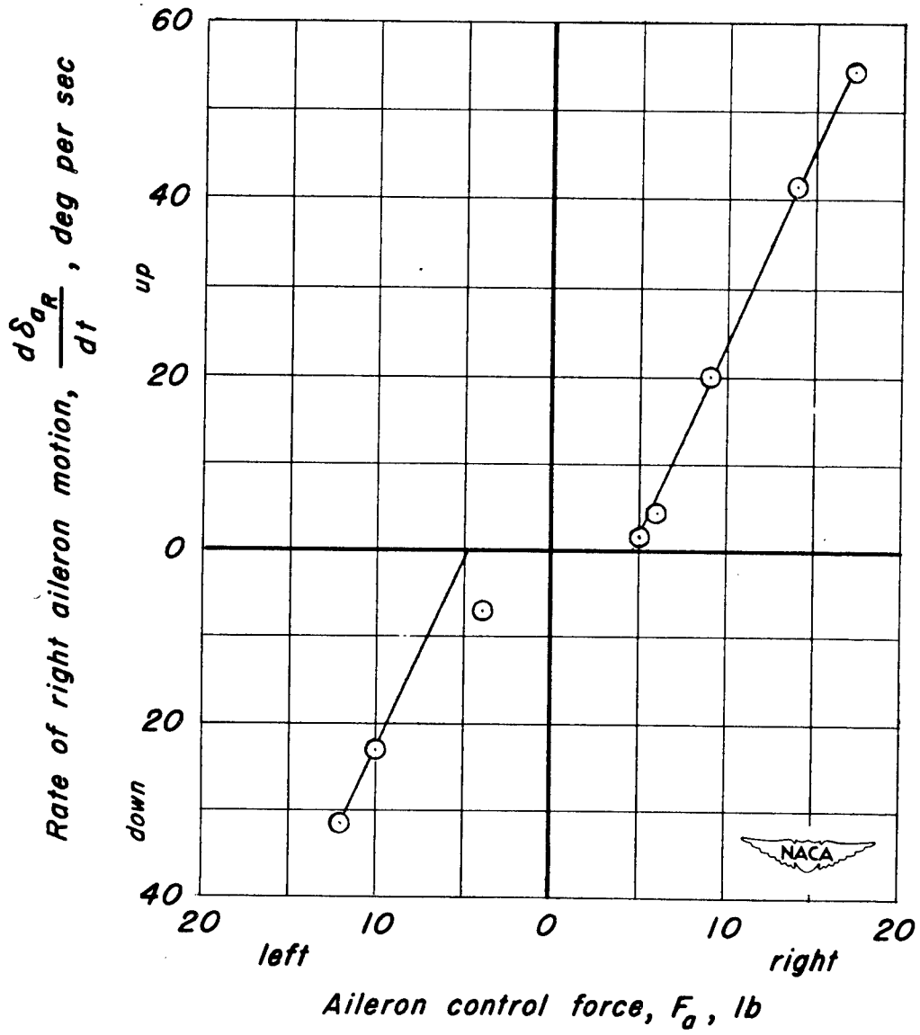
(c) Ailerons.
