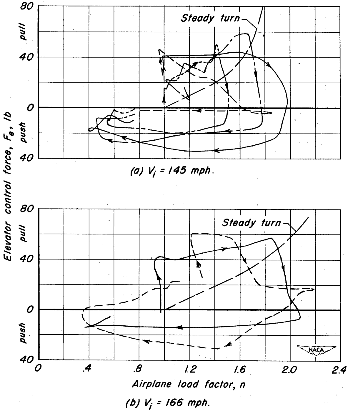
Figure 19.— Concurrent variation of elevator control force and airplane load factor during pitching maneuvers, 5,000 feet altitude.
