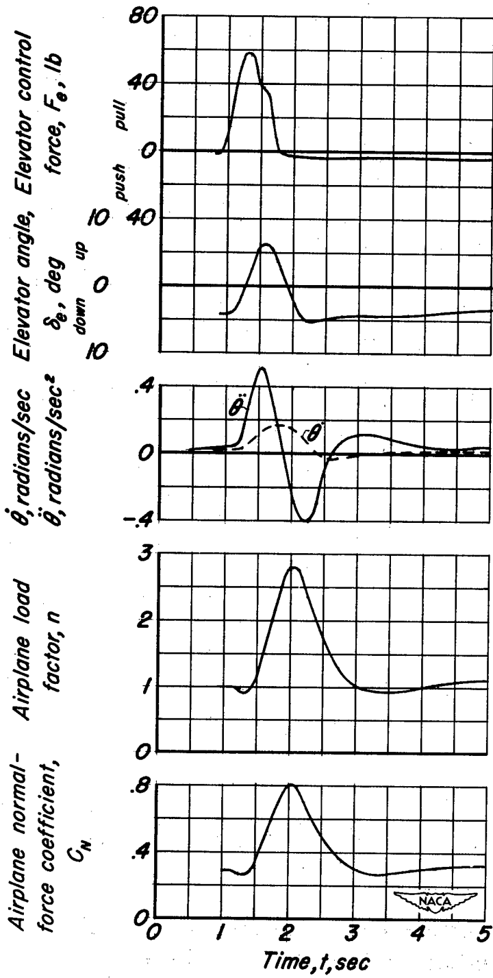
Figure 17.-Time history of pertinent quantities during pull-up maneuver; airspeed, 240 miles per hour; altitude, 19,800 feet.
