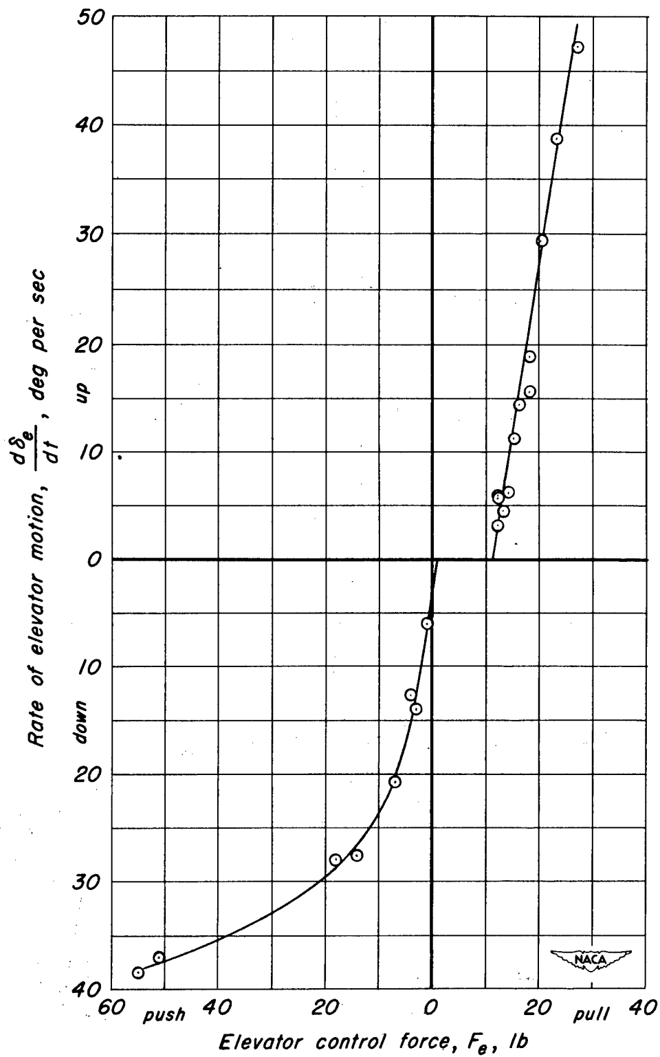
(a) Elevator.
