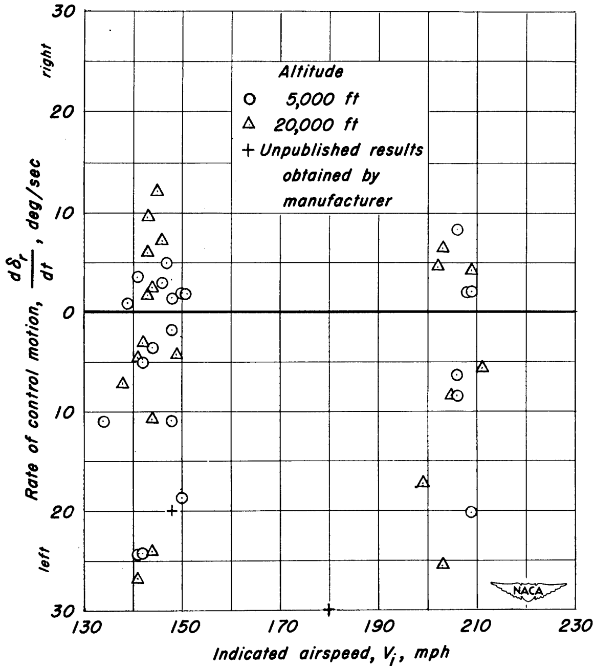
Figure 51.—Variation with airspeed of maximum rates of rudder motion attained during flight tests.
