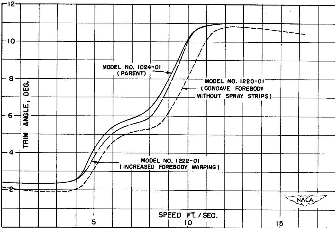
Figure 71.- Effect of increased forebody warping and concave forebody sections on resistance and trim in displacement range. Free-to-trim tests at zero trimming moment with a constant load of 5.45 pounds.
