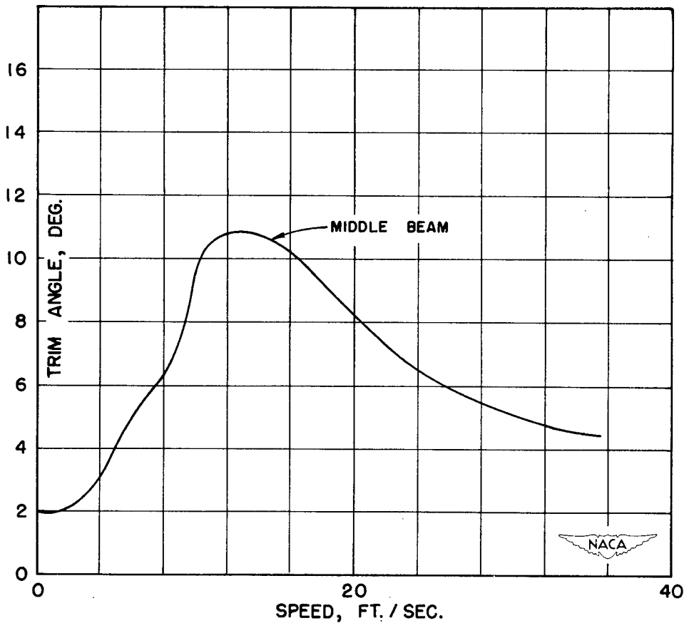
Figure 51.- Variation of resistance and trim with speed for model with a medium afterbody and sternpost angle of 8^\circ . Constant-load comparison; initial load, 5.86 pounds; take-off speed, 35.6 feet per second.
