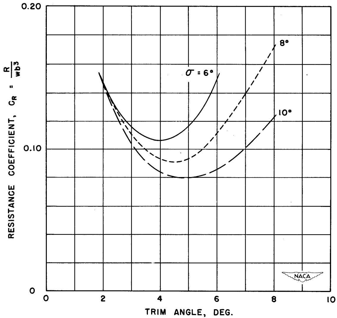
Figure 61.- Variation of resistance coefficient with trim angle at 90 percent of take-off speed of 68.7 miles per hour. Long-afterbody model no. 1057; C_V = 7.99 ; C_\Delta = 0.143 .
