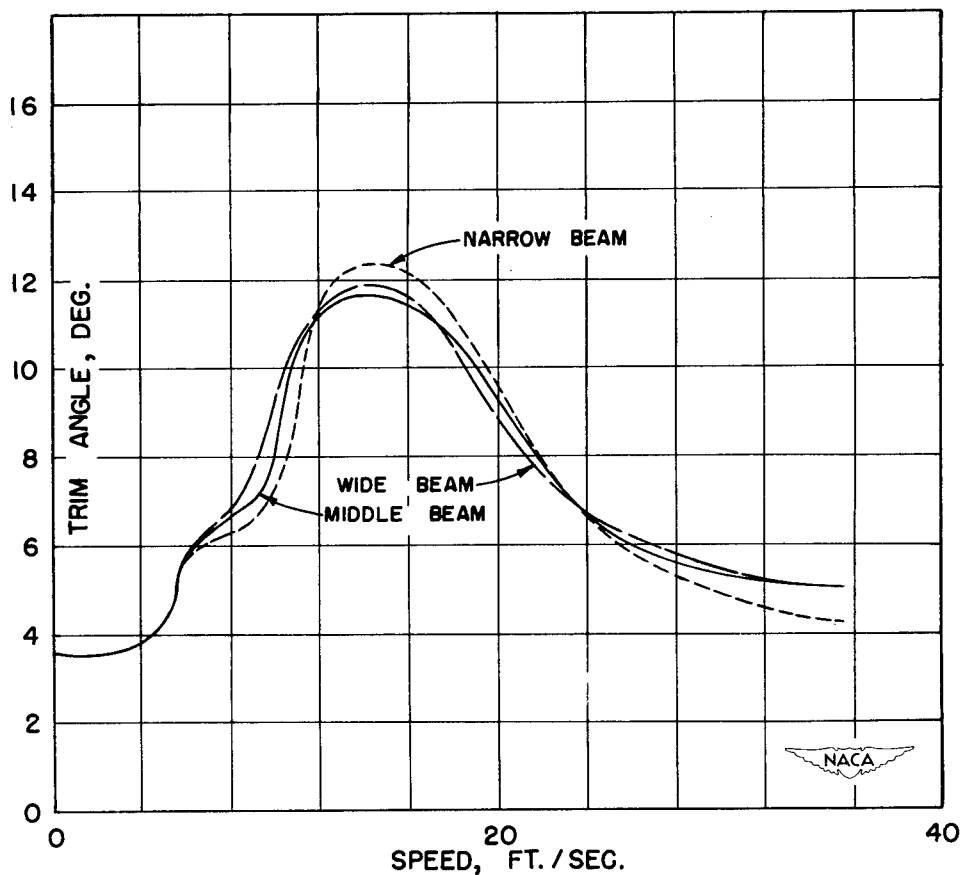
Figure 54.- Variation of resistance and trim with speed for models with a long afterbody and sternpost angle of 10^{\circ} . Constant-load comparison; initial load, 5.86 pounds; take-off speed, 35.6 feet per second.
