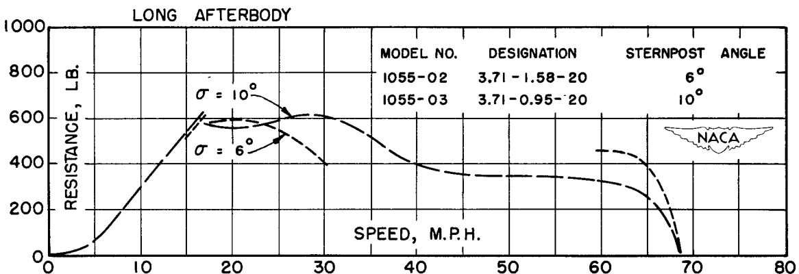
Figure 56.- Variation of resistance with speed for narrow-beam hulls. Comparison with constant forebody plan-form area; gross weight, 3000 pounds; take-off speed, 68.7 miles per hour.
