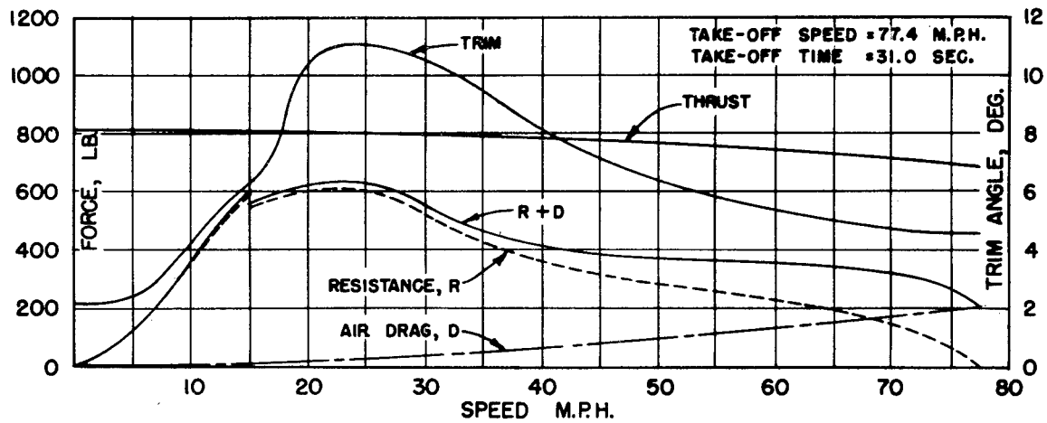
Figure 64.- Curves for determining take-off times of medium-afterbody hull. Model no. 1024-01; gross weight, 3000 pounds.
