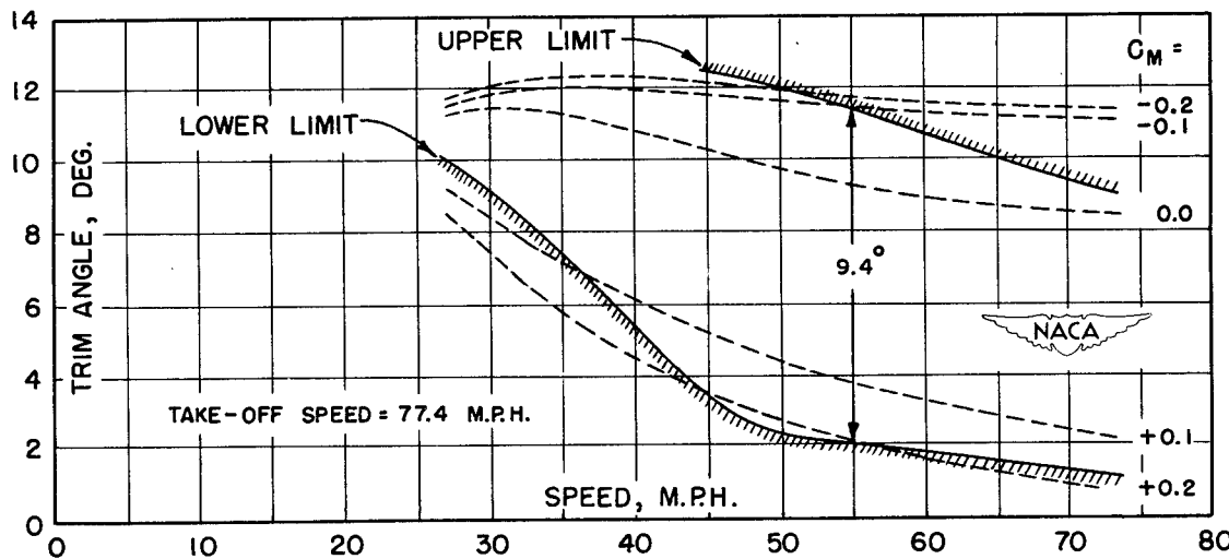
Figure 68.- Longitudinal stability characteristics of long-afterbody hull. Model no. 1057-03; gross weight, 3000 pounds.
