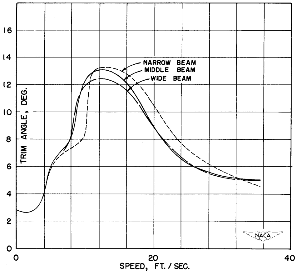
Figure 52.- Variation of resistance and trim with speed for models with a medium afterbody and sternpost angle of 10^\circ . Constant-load comparison; initial load, 5.86 pounds; take-off speed, 35.6 feet per second.
