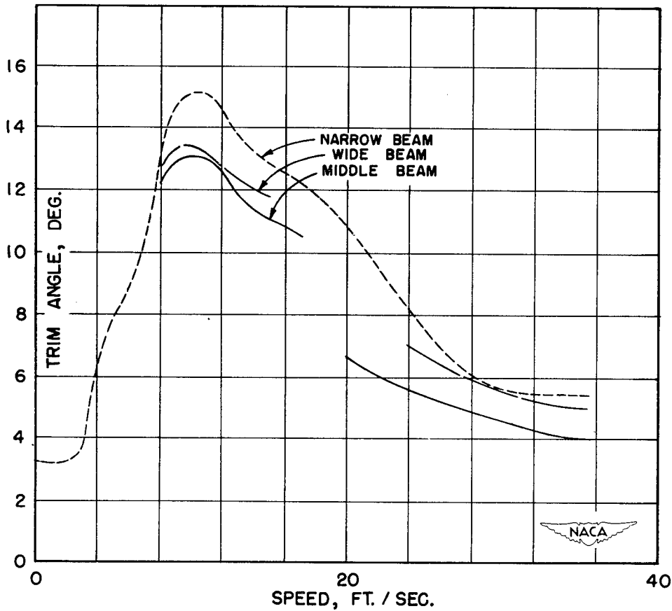
Figure 49.- Variation of resistance and trim with speed for models with a short afterbody and sternpost angle of 8^{\circ} . Constant-load comparison; initial load, 5.86 pounds; take-off speed, 35.6 feet per second.
