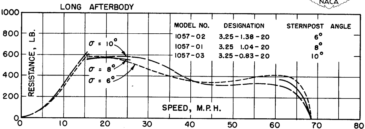
Figure 57.- Variation of resistance with speed for middle-beam hulls. Comparison with constant forebody plan-form area; gross weight, 3000 pounds; take-off speed, 68.7 miles per hour.
