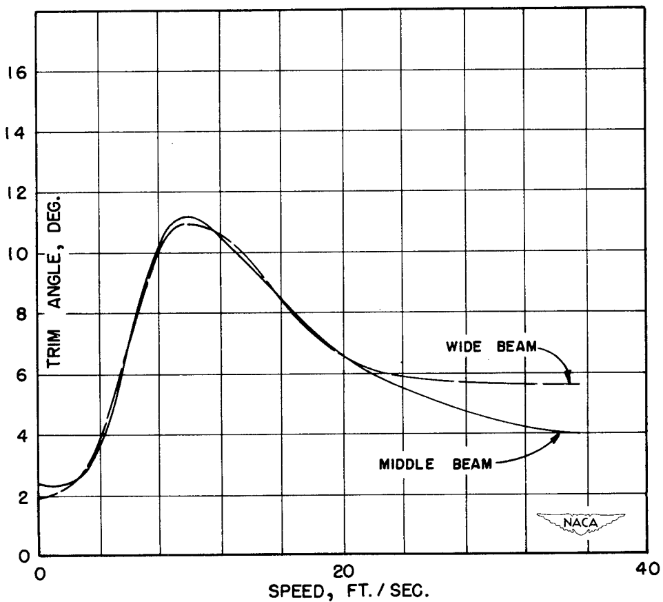
Figure 48.- Variation of resistance and trim with speed for models with a short afterbody and sternpost angle of 6^{\circ} . Constant-load comparison; initial load, 5.86 pounds; take-off speed, 35.6 feet per second.
