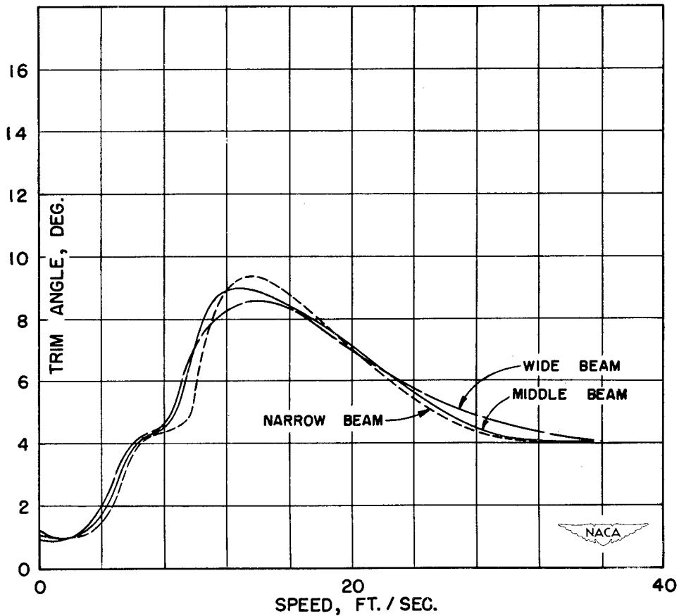
Figure 50.- Variation of resistance and trim with speed for models with a medium afterbody and sternpost angle of 6°. Constant-load comparison; initial load, 5.86 pounds; take-off speed, 35.6 feet per second.
