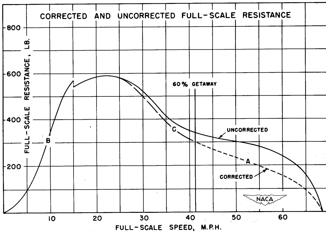
Figure 79.- Model and full-scale resistance.
