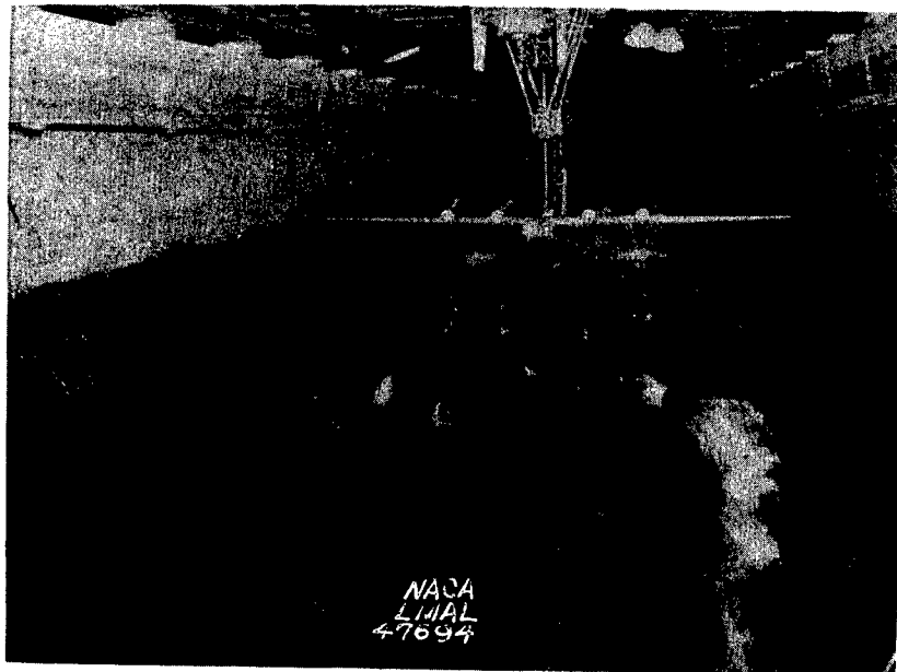
(b) Model landing in waves.
