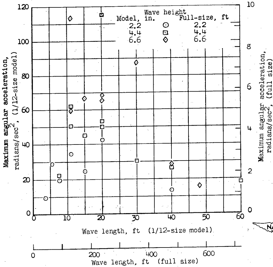
(b) Model 164J.
