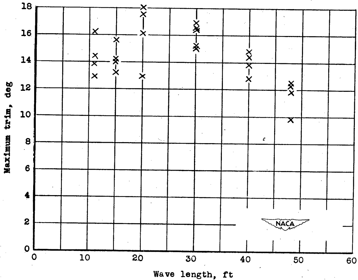
(b) Wave height, 6.6 inches (6.6 feet, full size).
