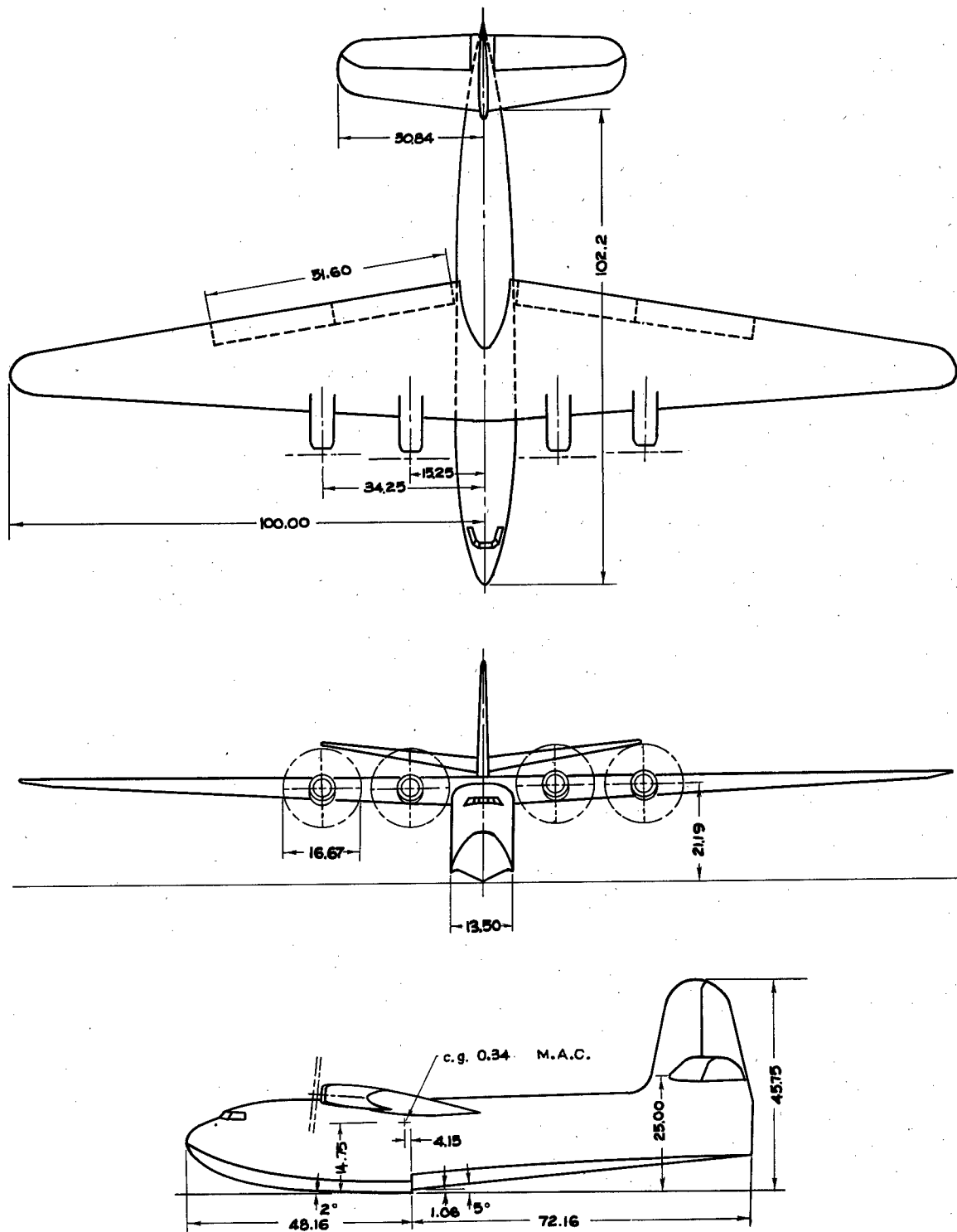
Figure 3.- General arrangement of Langley tank model 164L. (All dimensions are in inches.)
