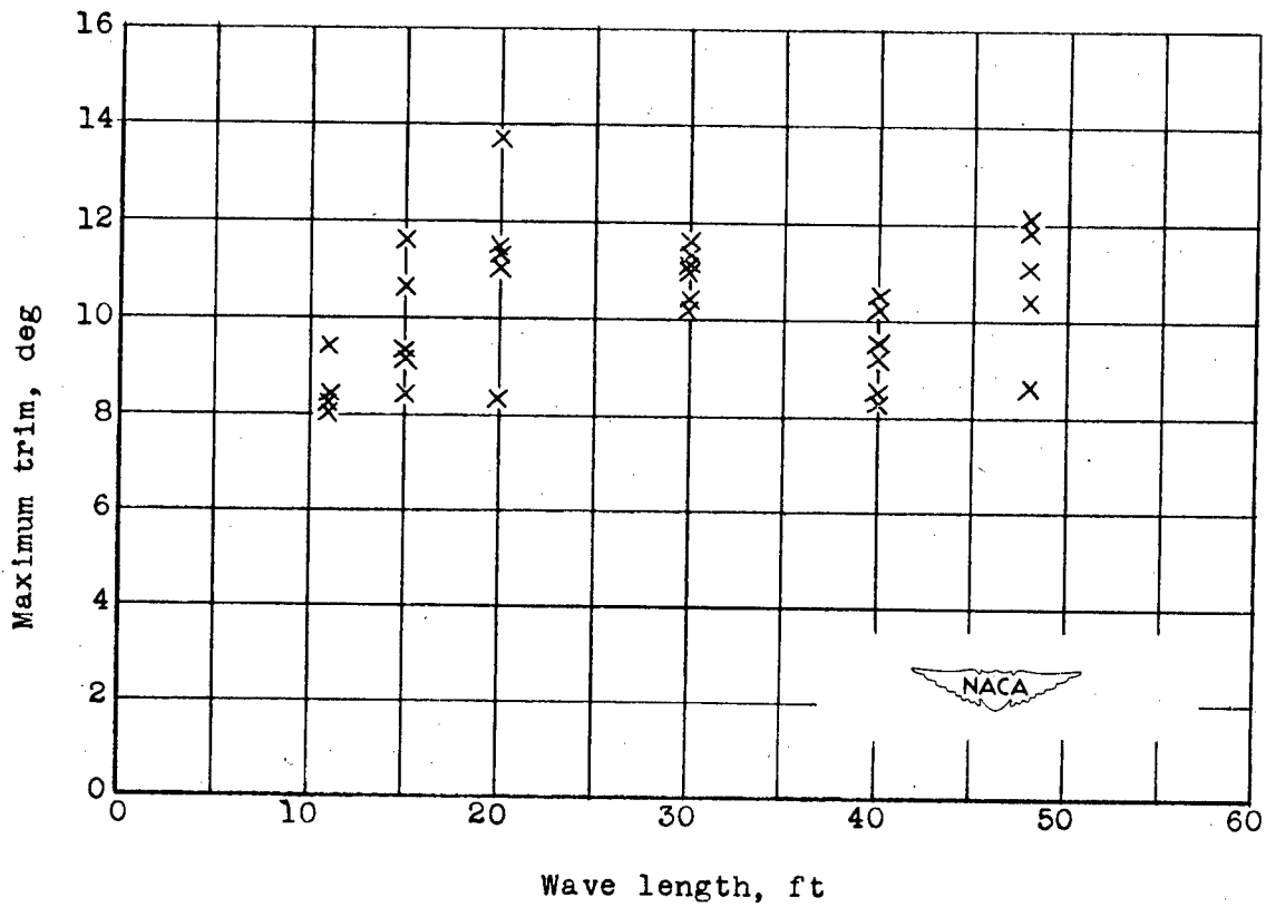
(b) Wave height, 6.6 inches (6.6 feet, full size).
