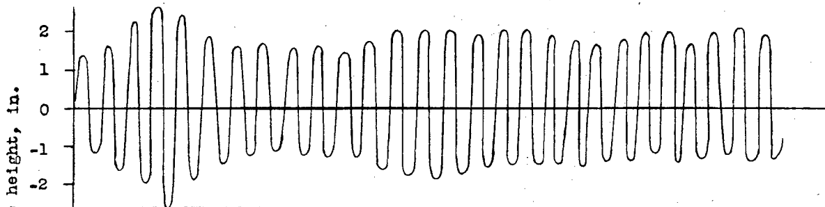
(b) Wave length, 9.4 feet; designated wave height, 3.5 inches.
