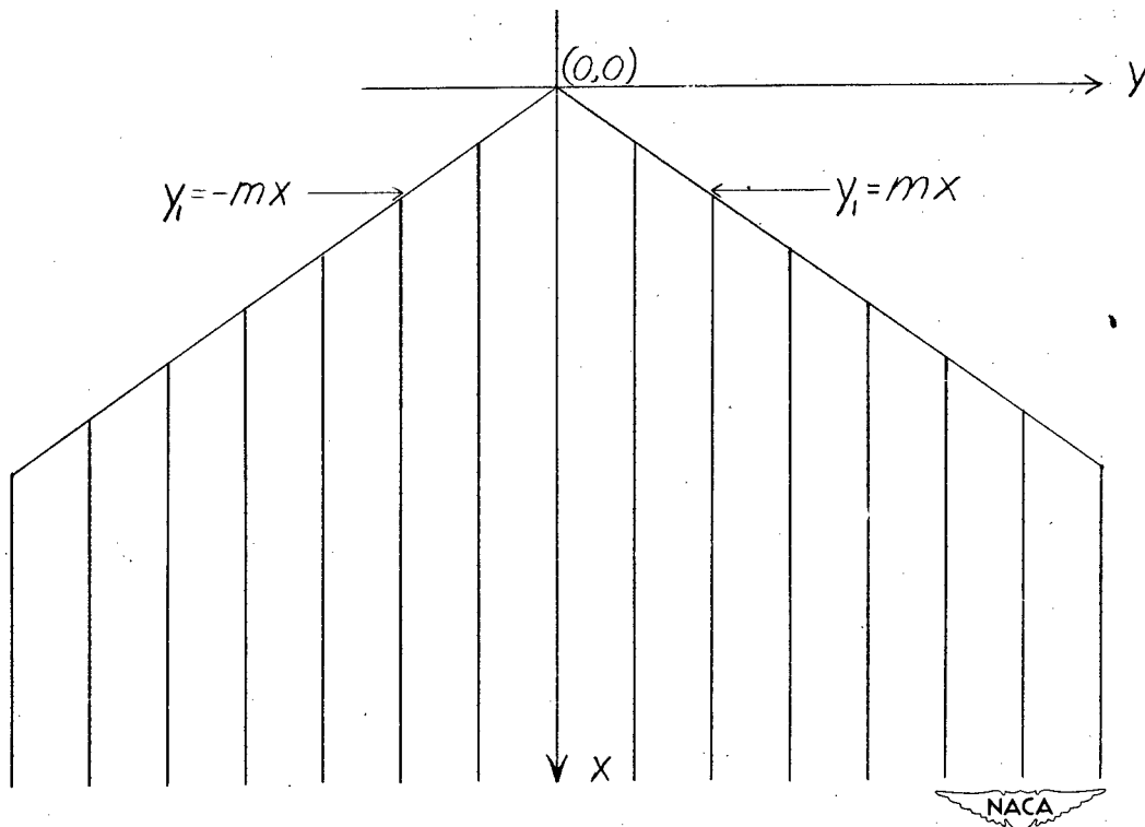
Figure 8.- Bent lifting line approximated by a series of finite vortices.
