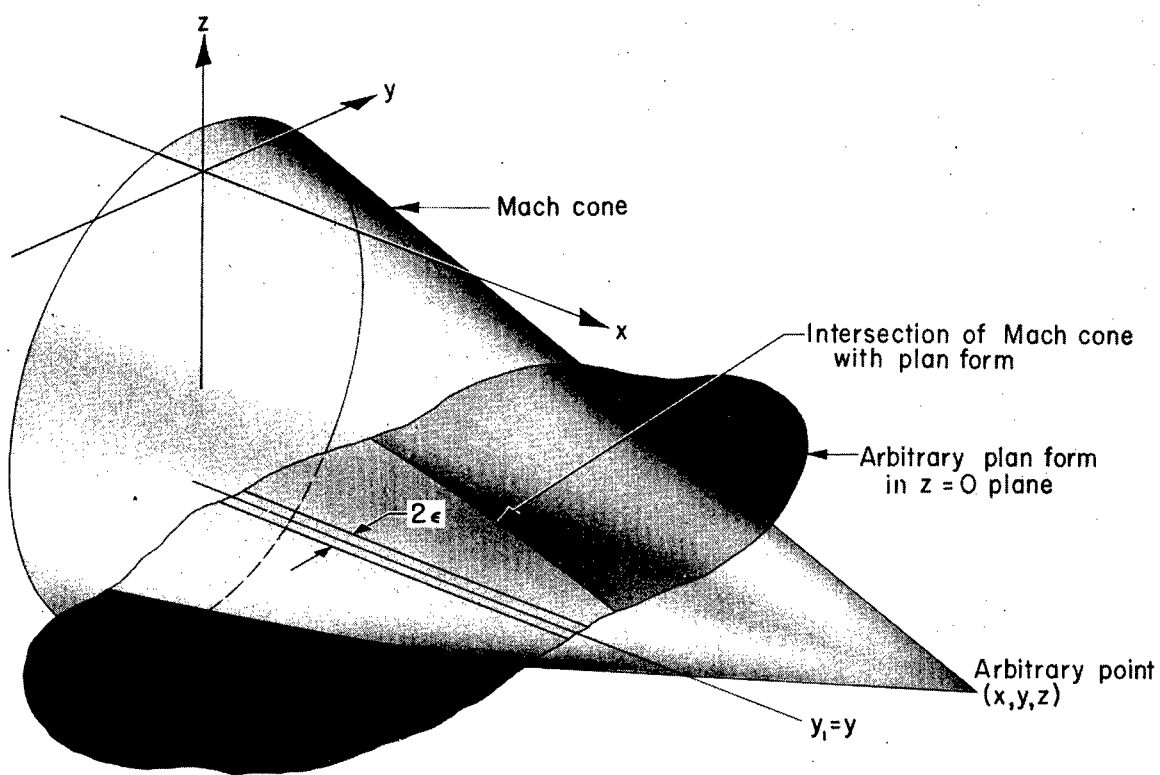
(b) Arbitrary point above wake.
