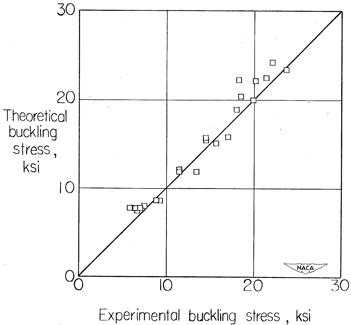
Figure 5.- Comparison of theoretical and experimental buckling stresses for sandwich plates with Alclad 24S-T aluminum-alloy faces and cellular-cellulose-acetate cores.
