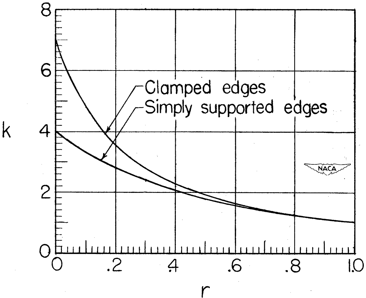
Figure 3.- Comparison of elastic-compressive-buckling coefficients for infinitely long Metalite type sandwich plates with clamped edges ( \mu_F = \frac{1}{3} ) and with simply supported edges.
