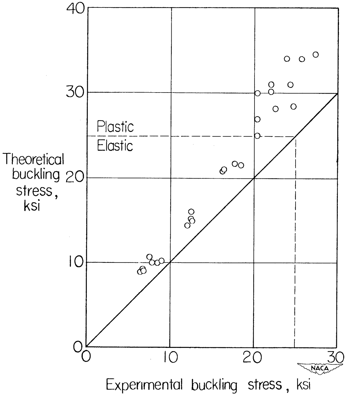
Figure 4.— Comparison of theoretical and experimental buckling stresses for sandwich plates with Alclad 24S-T aluminum faces and balsa-wood cores.
