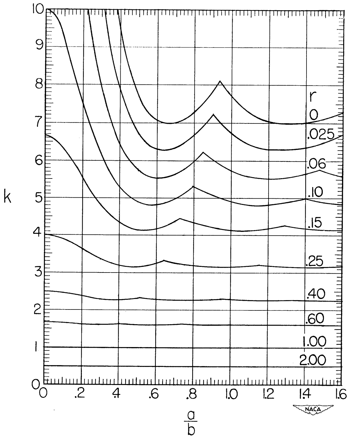
Figure 2.— Elastic-compressive-buckling curves for Metalite type sandwich plates with simply supported loaded edges and clamped unloaded edges ( \mu_F = \frac{1}{3} ).
