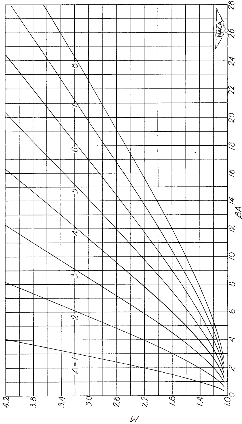
Figure 4.— Variation of M with \beta_A . (4 blocks = 1 inch).
