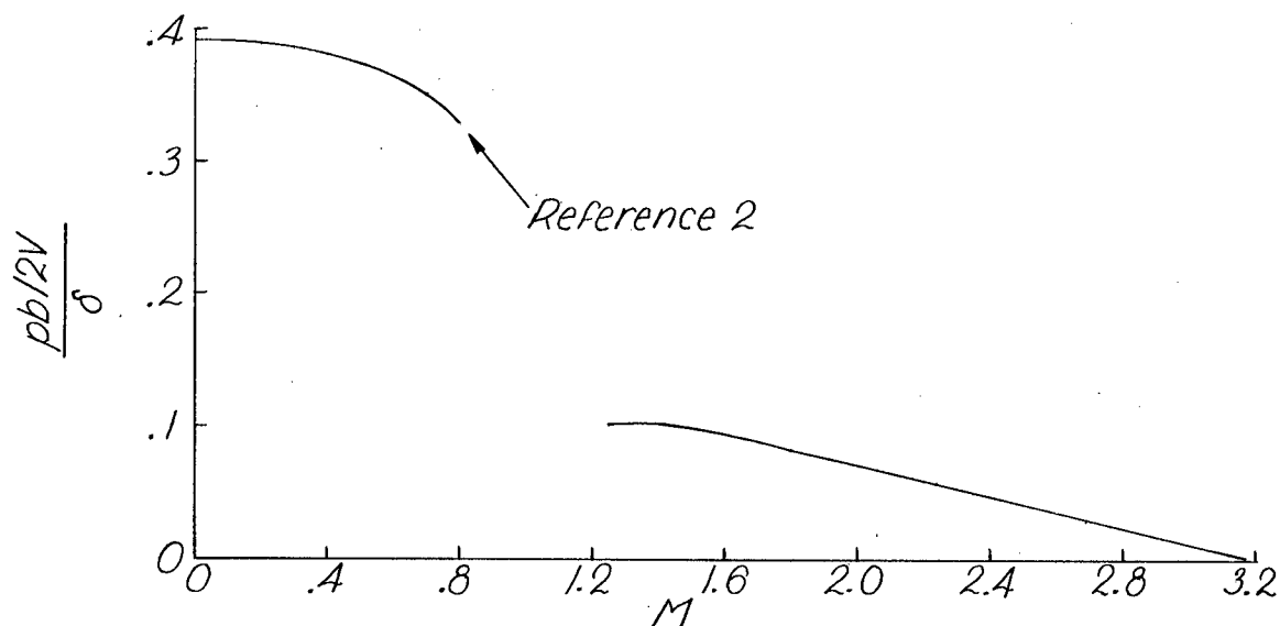
Figure 16.- Results of computations for a hypothetical configuration at sea level. A = 4 ; \lambda = 0.4 ; \frac{b_a}{b} = 0.4 ; \frac{c_a}{c} = 0.2 ; b = 30 feet; m\theta_r = 2,000,000 foot-pounds per radian; \phi_N = 8^\circ .
