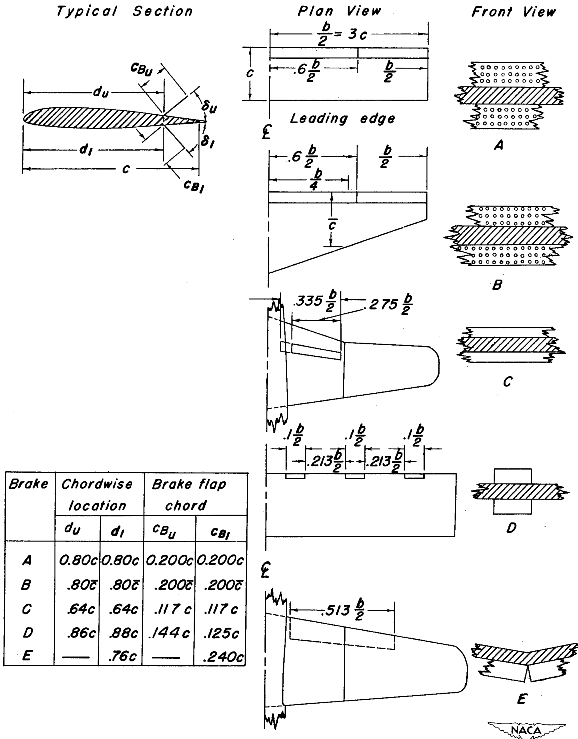
(a) Split-flap-type air brakes.
