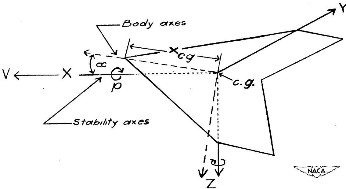
(a) Notation and body axes used in analysis. Origin is located at projection of leading edge of tip on center section.
