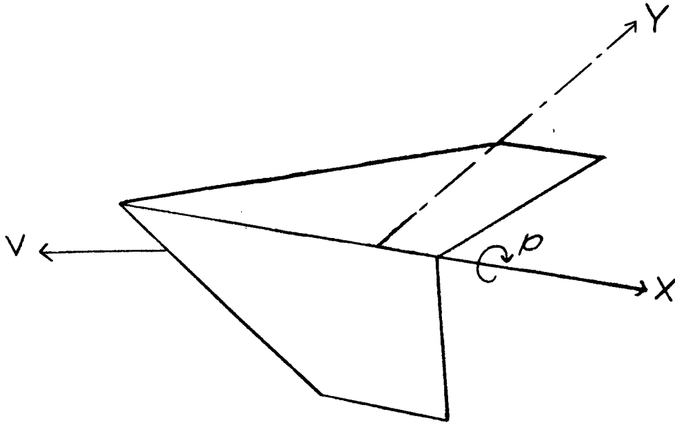
(a) Notation and body axes used in analysis. Origin is located at projection of leading edge of tip on center section.
