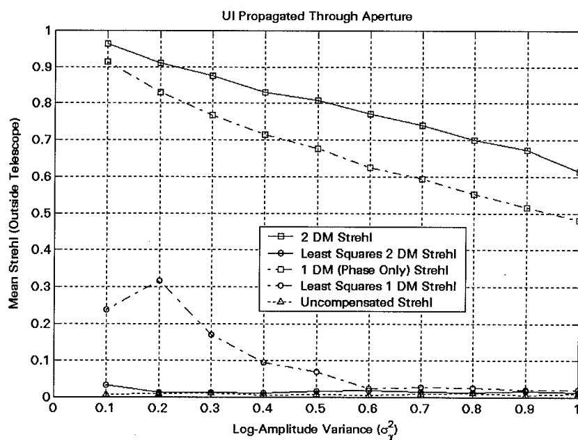
Figure 5.16. Mean Strehl Ratio Outside Telescope vs. Log-Amplitude Variance
