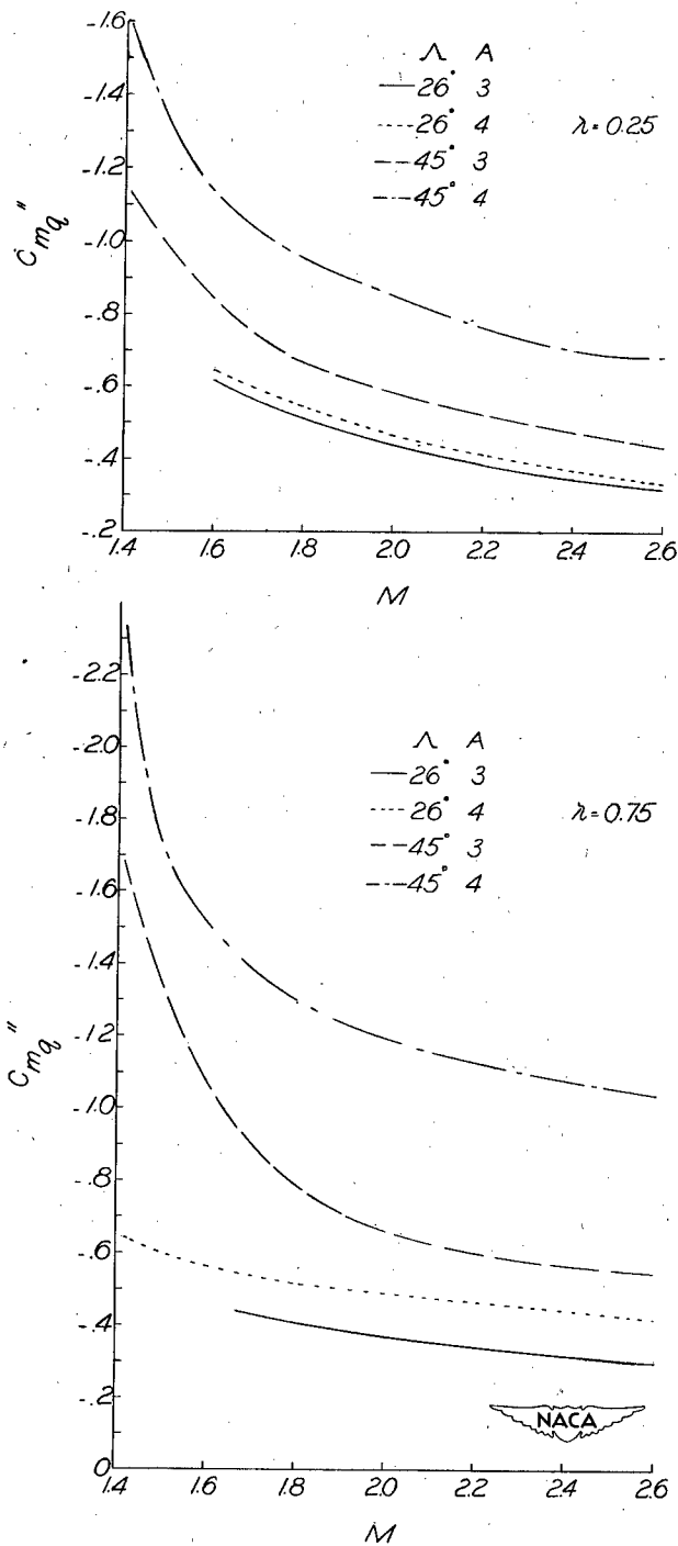
(a) Variation with Mach number.
