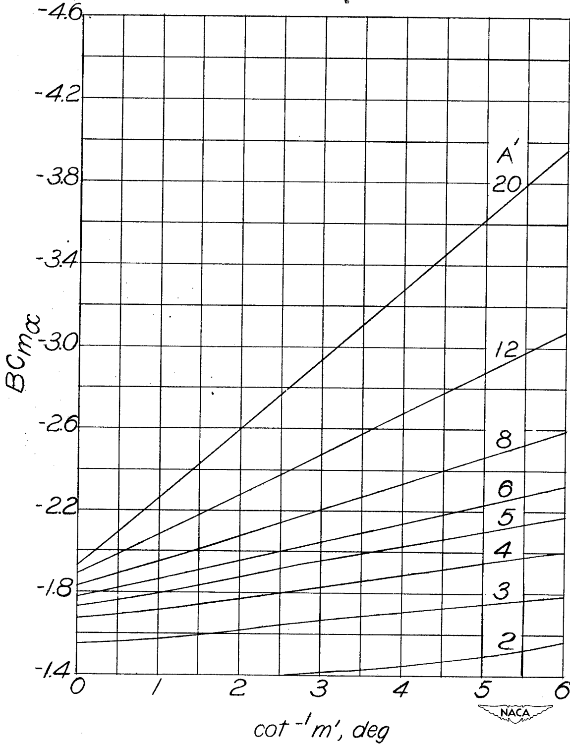
(c) \lambda = 1.0 ; A' = 2 to 20; m' = \infty to 9.4.
