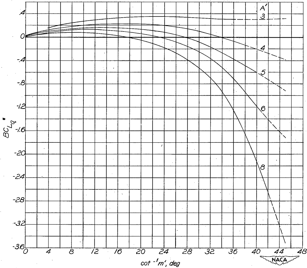
(a) \lambda = 0.25 ; A' = 3 to 8 ; m' = \infty to 1 .
