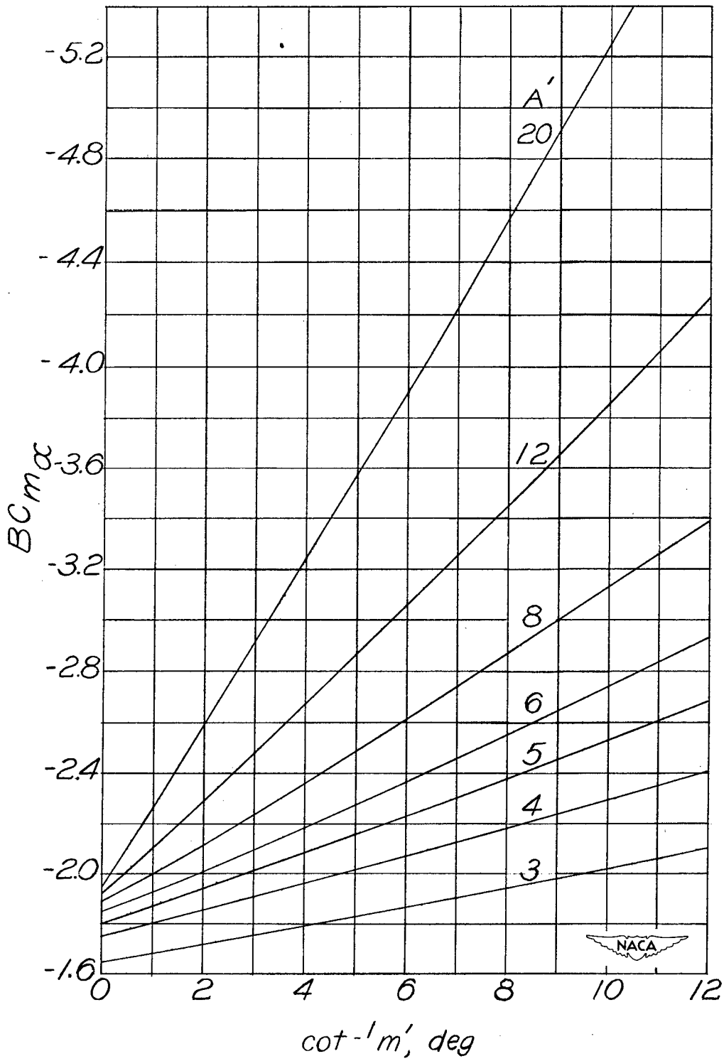
(c) \lambda = 0.75 ; A' = 3 to 20; m' = \infty to 4.7.
