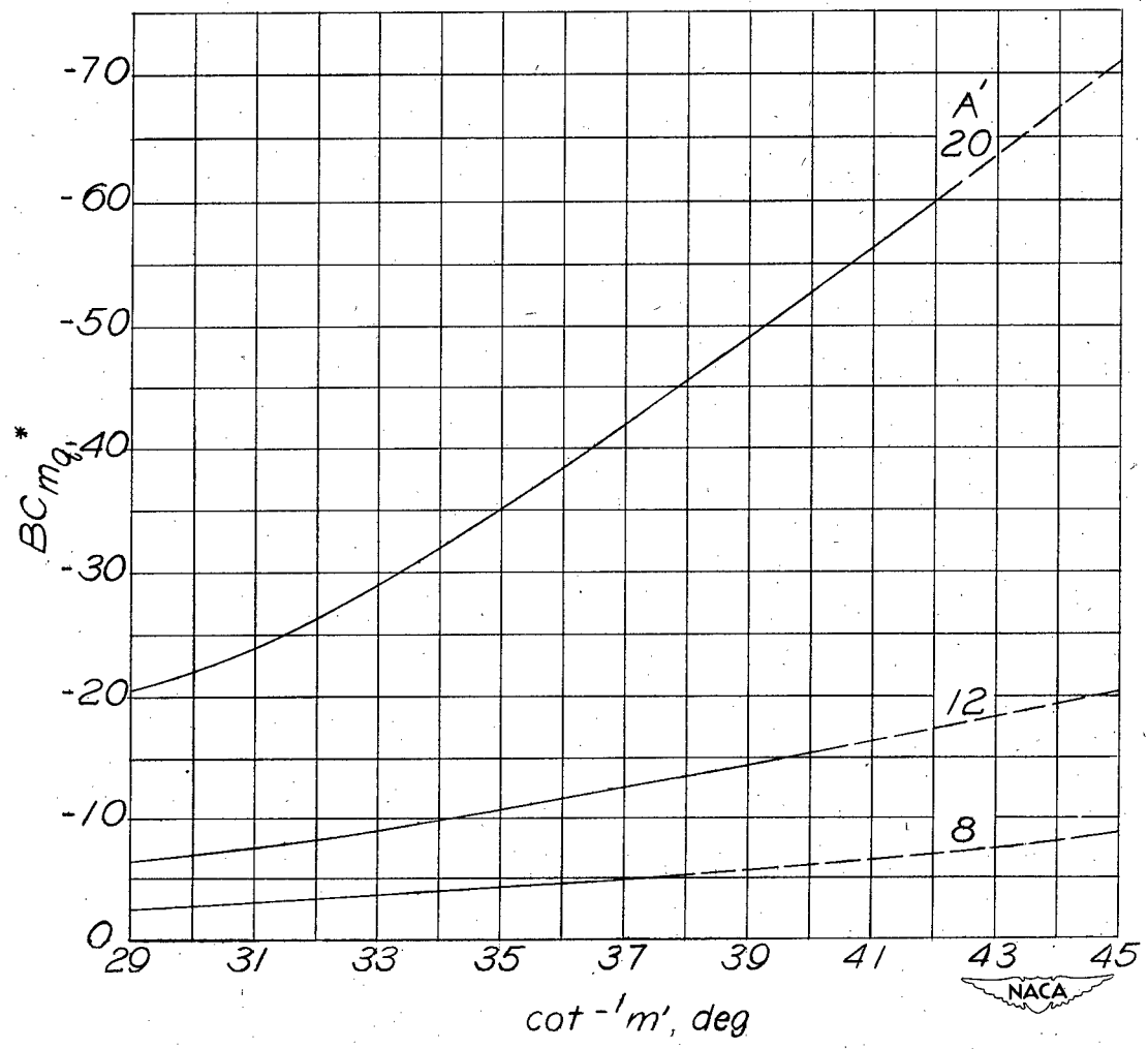
(c) \lambda = 0.75 ; A' = 8 to 20; m' = 1.8 to 1.
