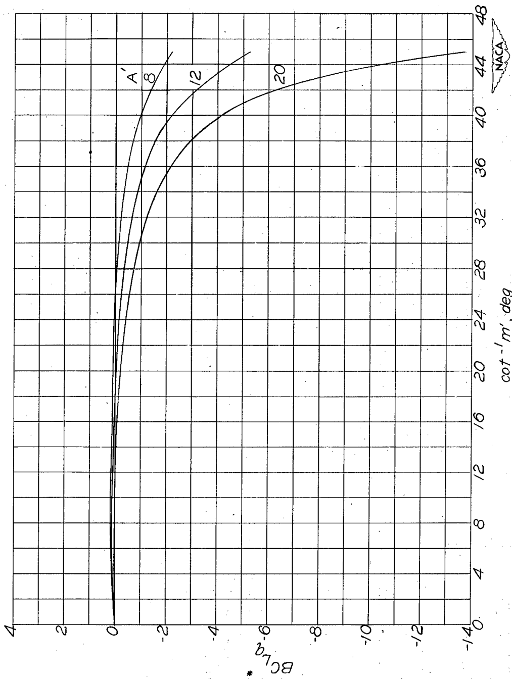
(b) \lambda = 0 ; A' = 8 to 20; m' = \infty to 1.
