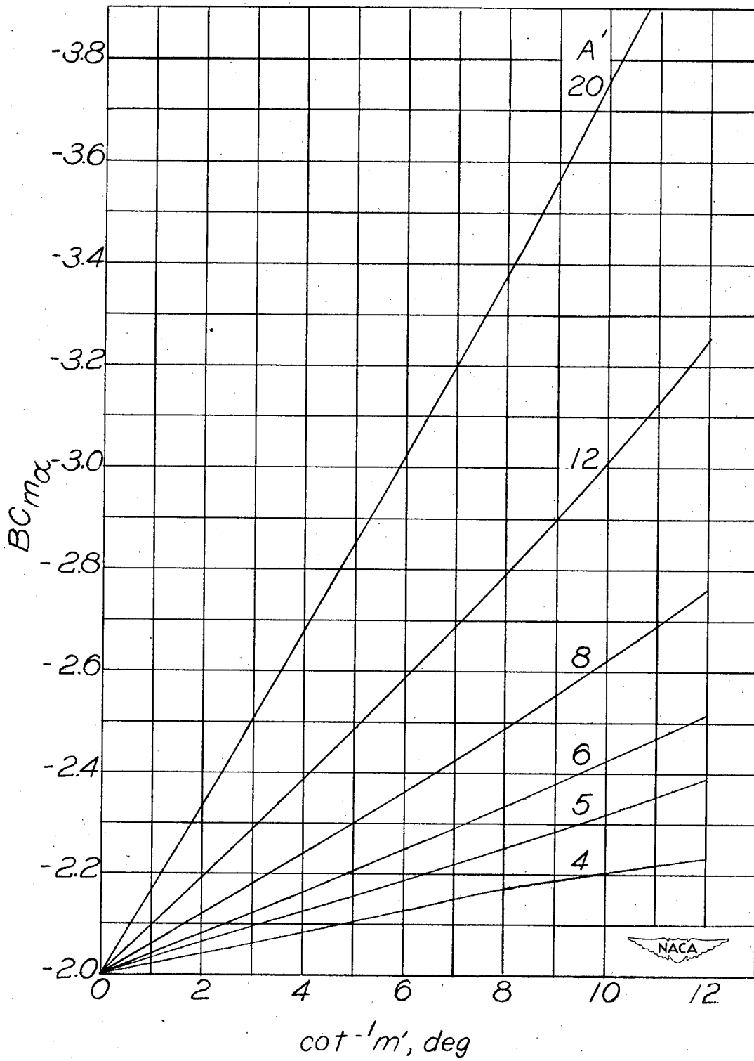
(c) \lambda = 1 ; A' = 4 to 20; m' = \infty to 4.7.
