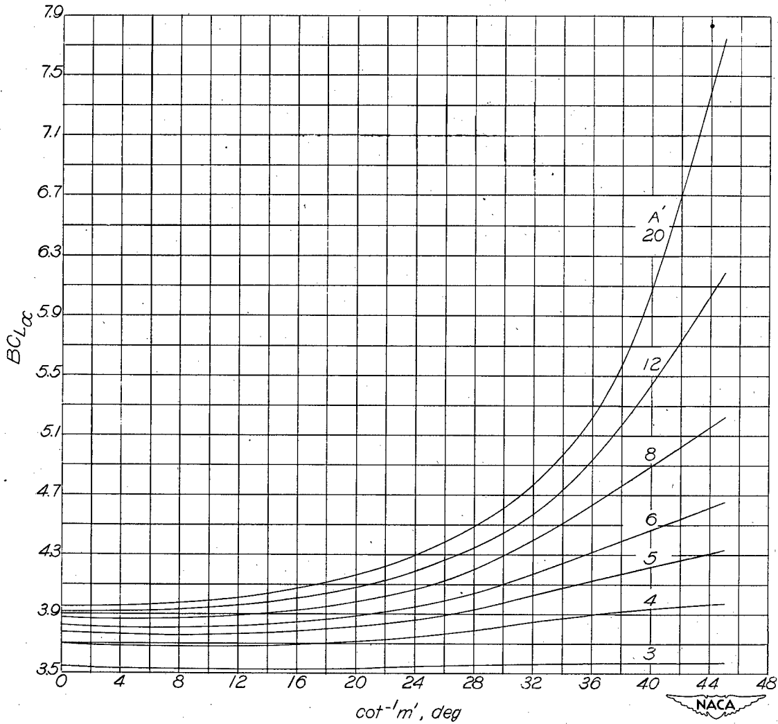
Figure 28.- Variation of BC_{L\alpha} with \cot^{-1}m' for various values of A' . System of body axes; \lambda = 0.50 .
