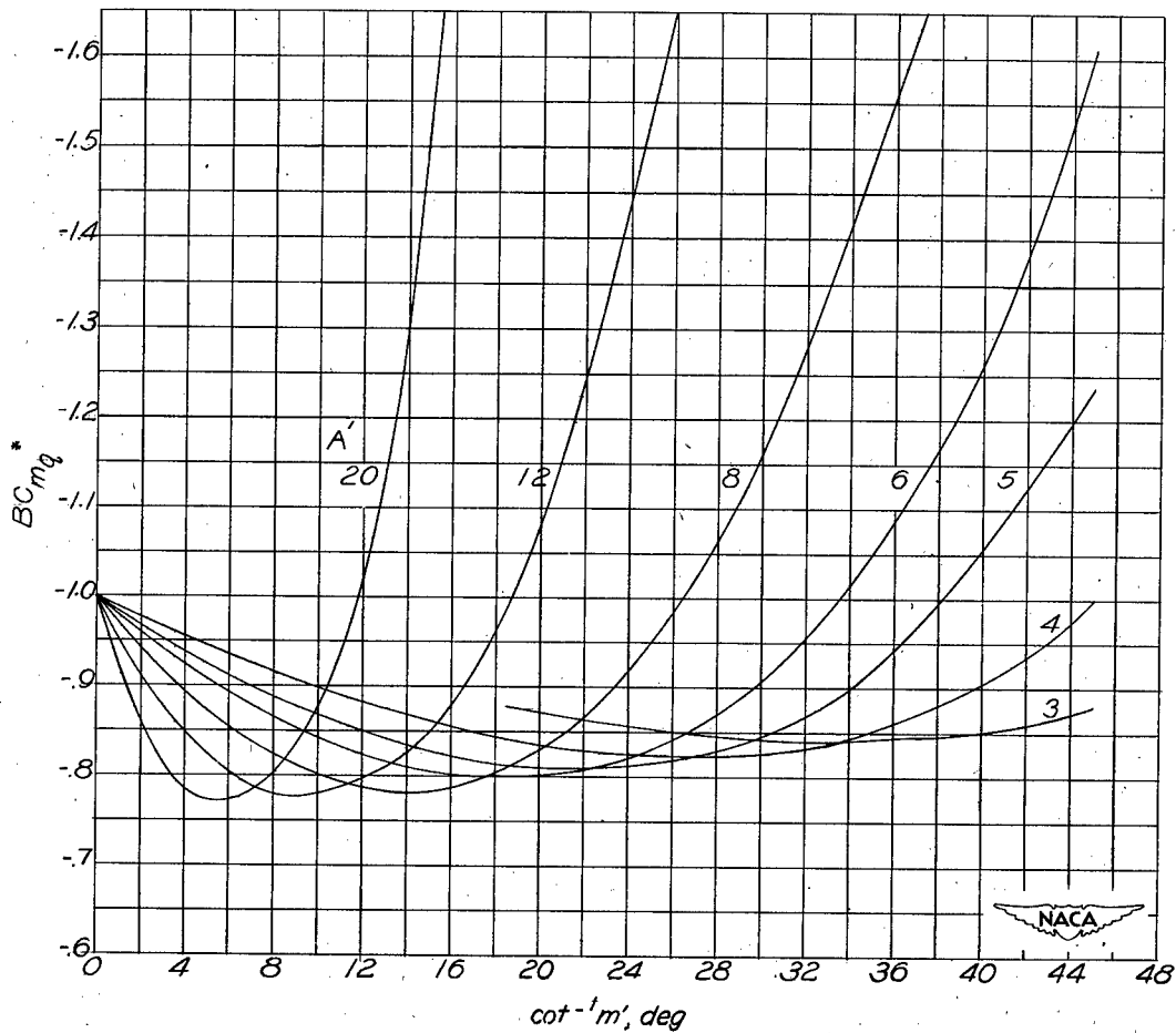
(a) \lambda = 0 ; A' = 3 to 20 ; m' = \infty to 1 .
