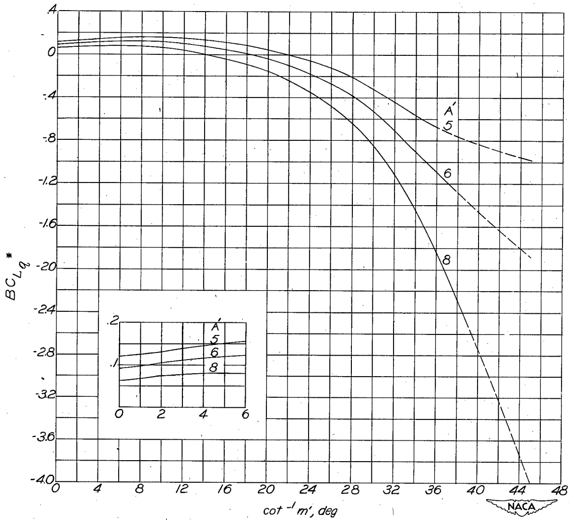
(b) \lambda = 0.50 ; A' = 5 to 8 ; m' = \infty to 1 .
