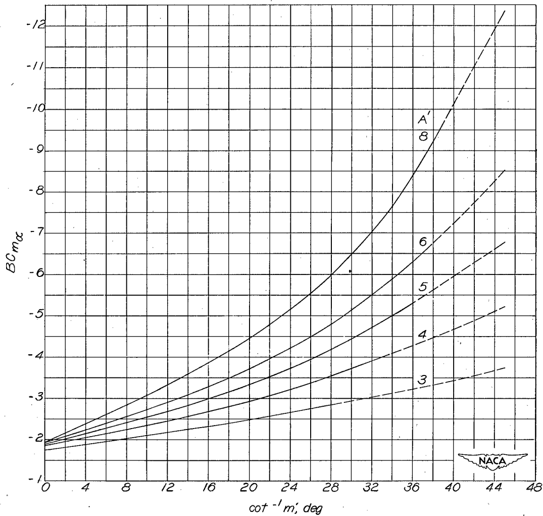
(a) \lambda = 0.50 ; A' = 3 to 8 ; m' = \infty to 1 .
