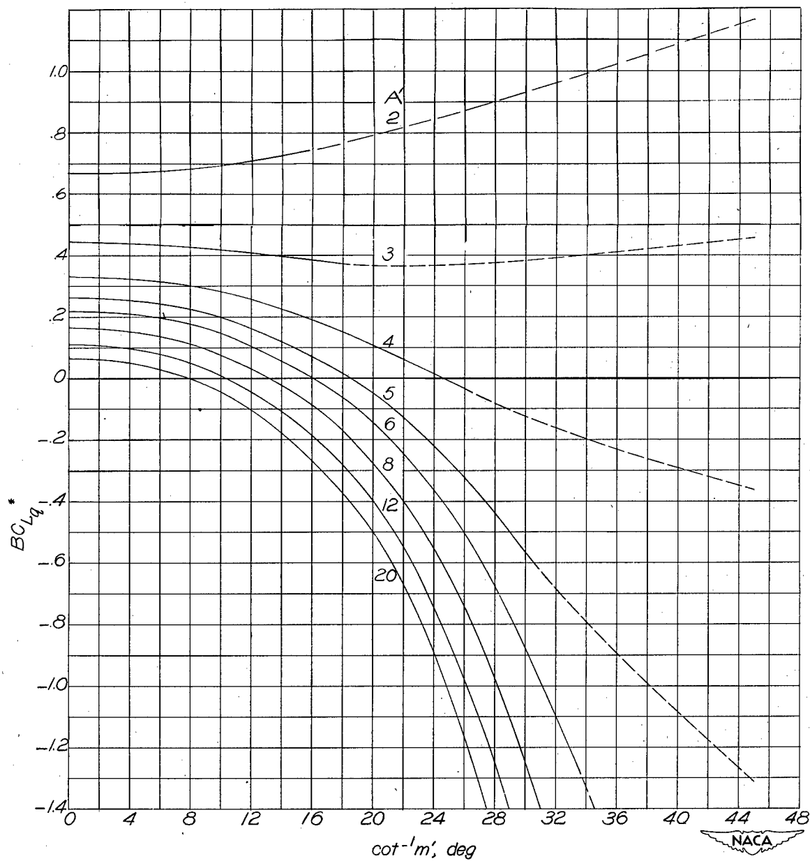
(a) \lambda = 1.0 ; A' = 2 to 20 ; m' = \infty to 1 .
