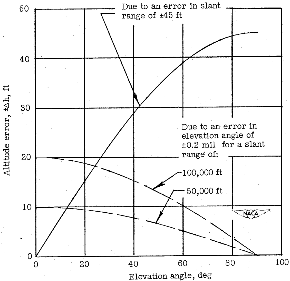
Figure 4.- Error in altitude due to error in range, \Delta r = \pm 45 feet, and to error in elevation angle, \Delta \theta = \pm 0.2 mil.
