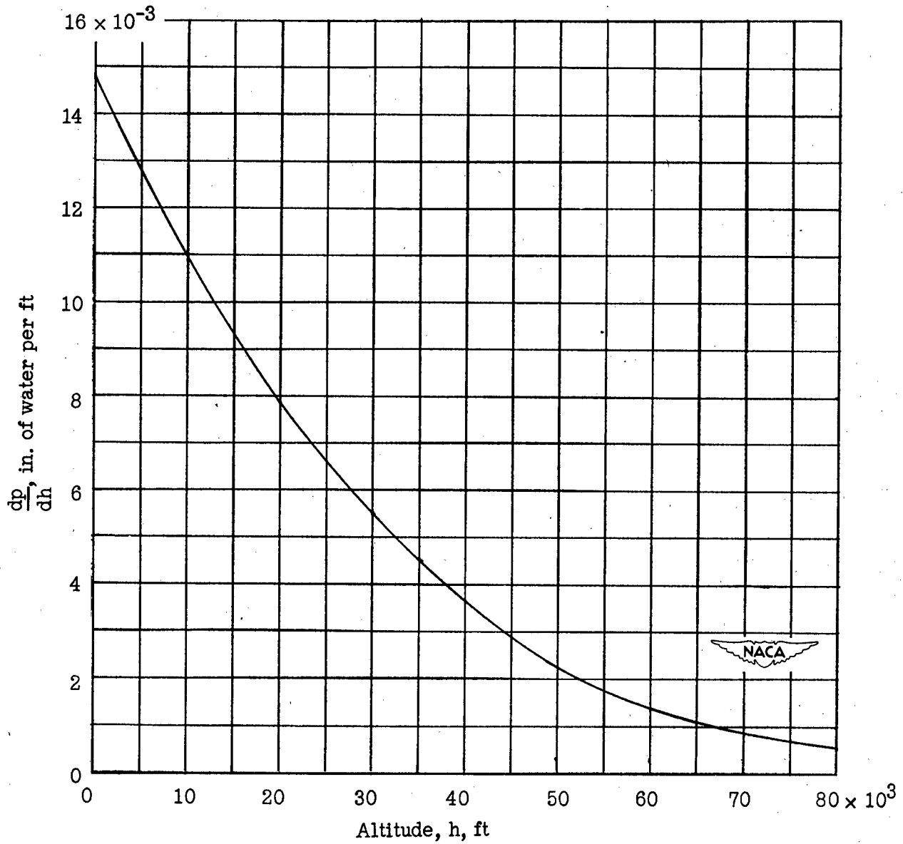
Figure 7.- Rate of change of atmospheric pressure with altitude. NACA standard atmosphere.
