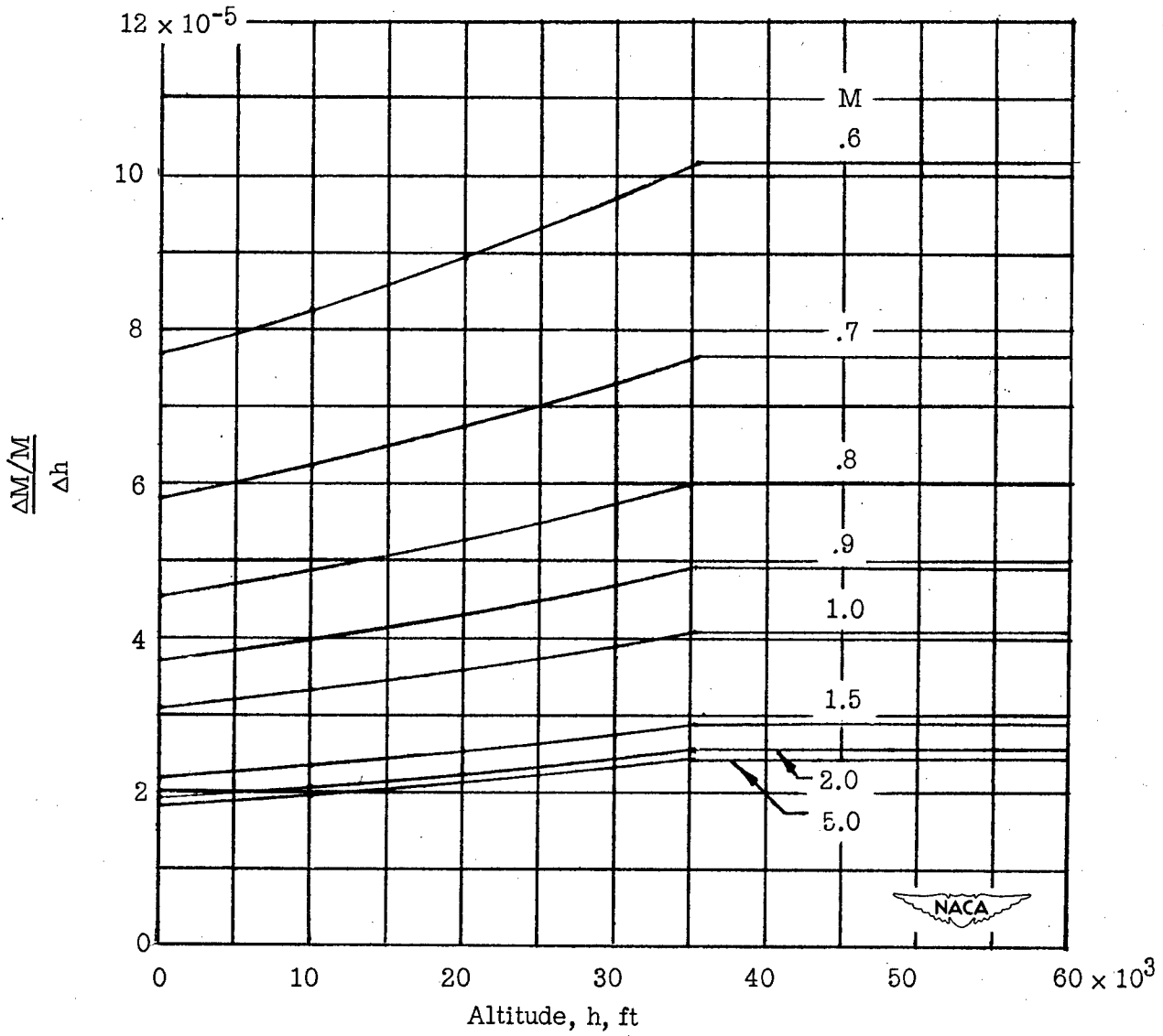
Figure 5.- Error in Mach number due to an error in altitude.
