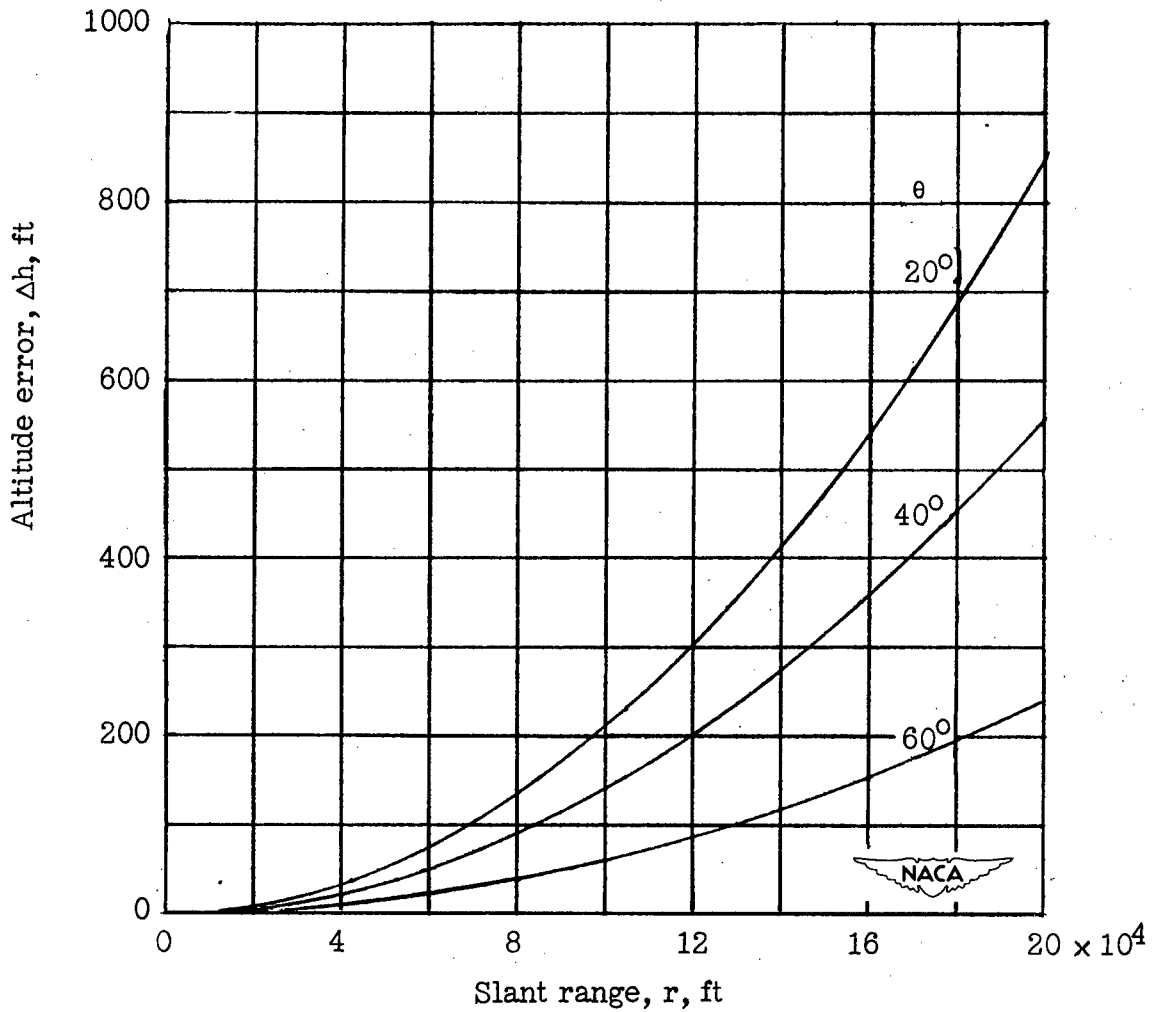
Figure 3.- Error in altitude due to curvature of the earth.
