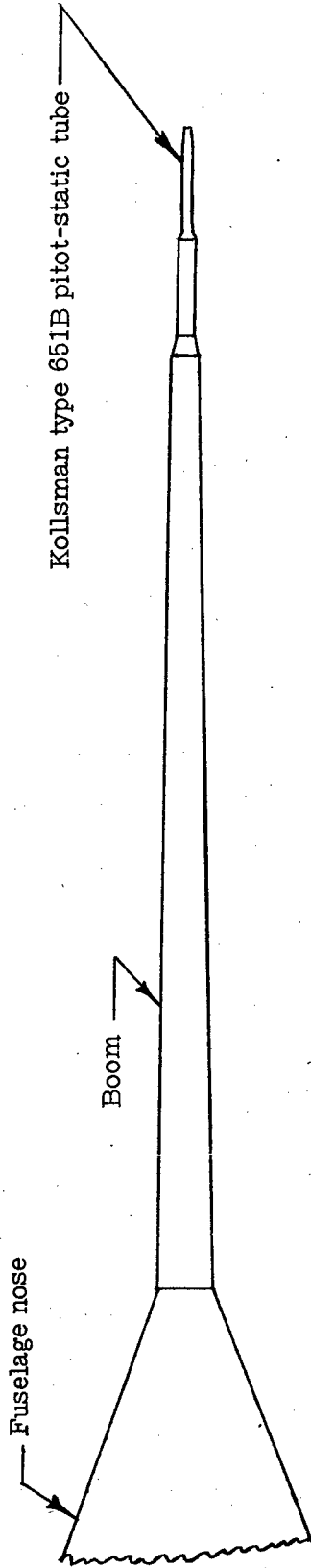
(a) Fuselage-nose airspeed installation.
