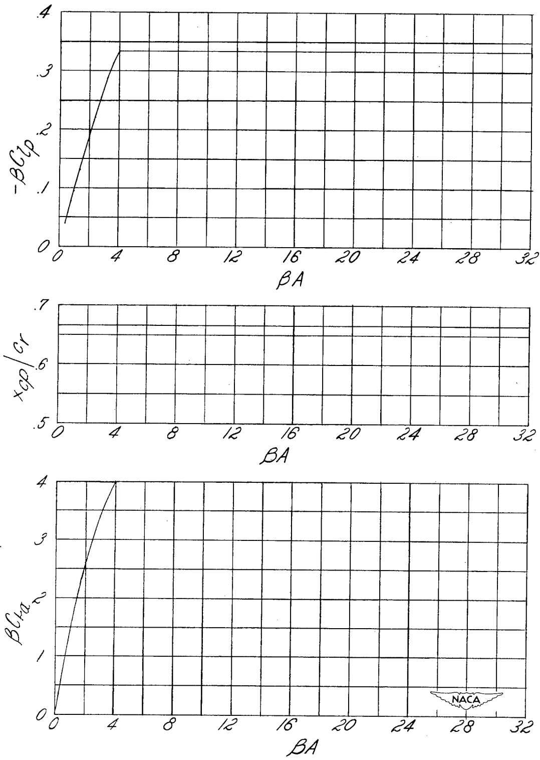
Figure 7.- Variation of BC_{L_{\alpha}} , x_{cp}/c_r , and -BC_{lp} with BA for triangular wings.
