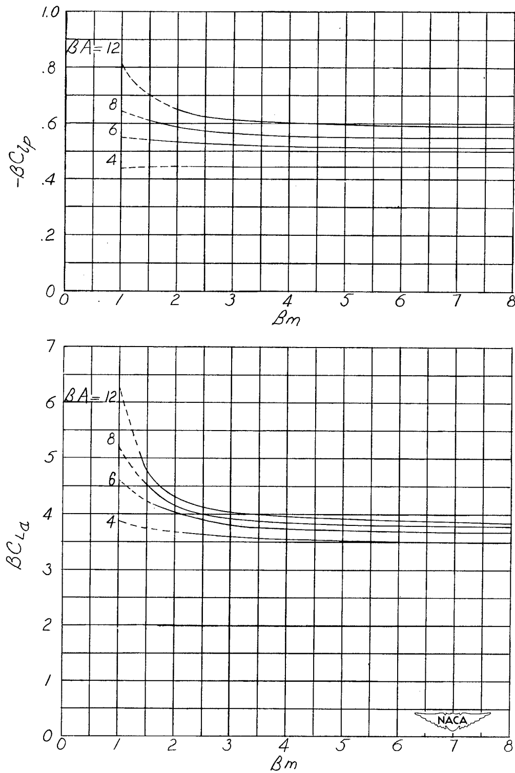
Figure 9.- Variation of BC_{L_{\alpha}} and -BC_{l_p} with \beta m for swept untapered wings with supersonic leading edges.
