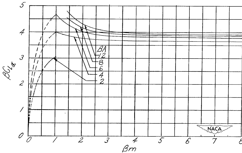
Figure 10.— Variation of BC_{L\alpha} and -BC_{lp} with \beta m for swept tapered wings. Taper ratio, 0.5.
