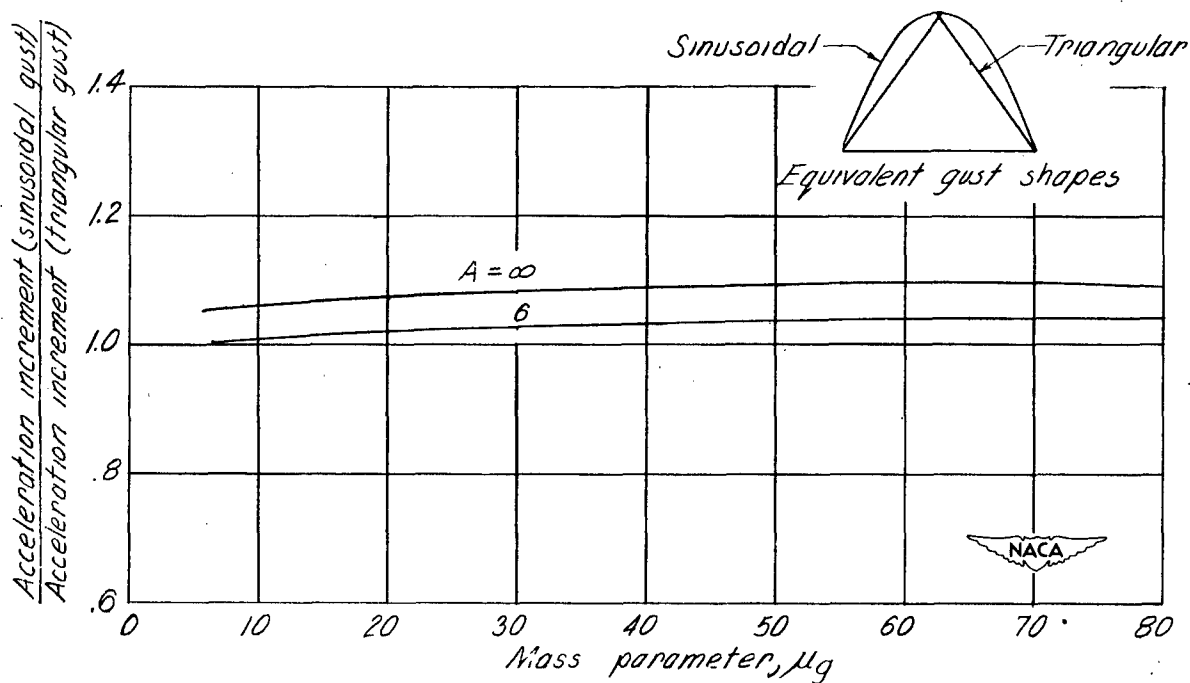
Figure 40.— Relative response of an airplane encountering sinusoidal and triangular gusts as a function of mass parameter.
