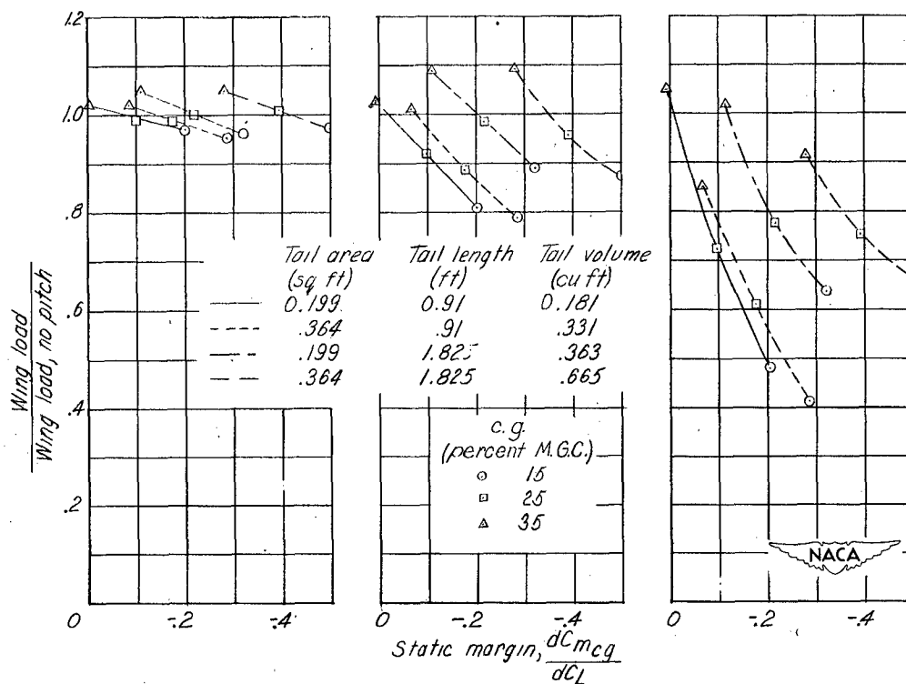
Figure 34.— The ratio of total wing load to the wing load with no pitch as a function of static margin for a conventional airplane.
