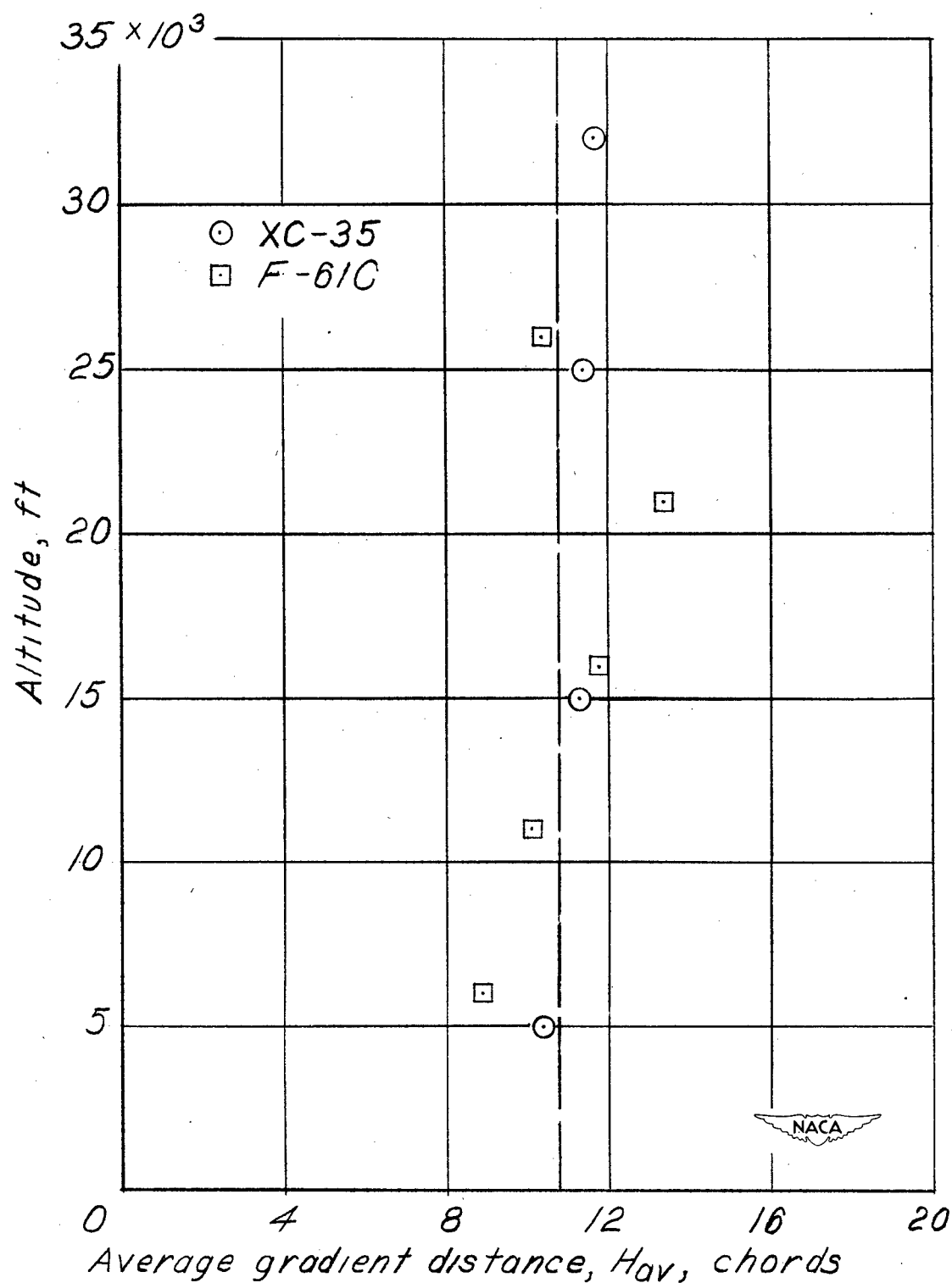
Figure 14.— Variation of average gradient distance with altitude.
