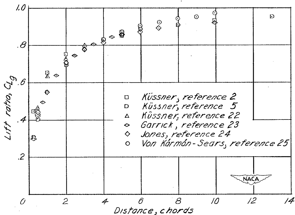
Figure 25.— Unsteady-lift function for an airfoil traversing a sharp gust.
