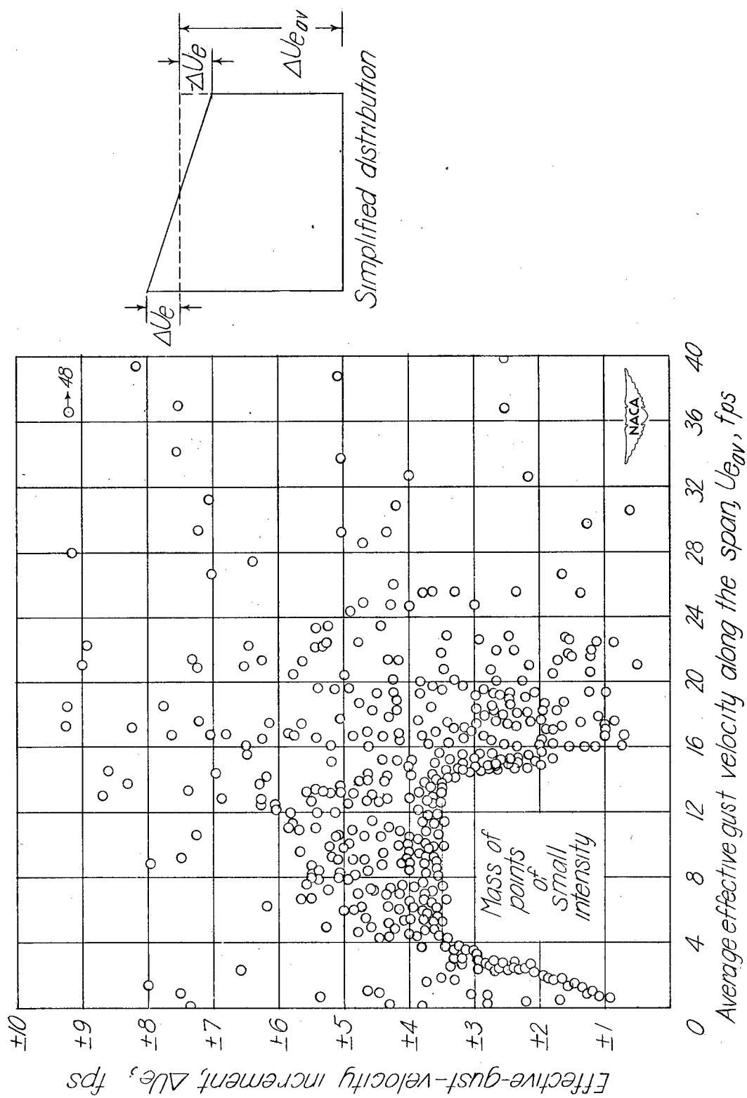
Figure 18.— Effective-gust-velocity increment \pm \Delta U_e as a function of the average effective gust velocity U_{eav} .
