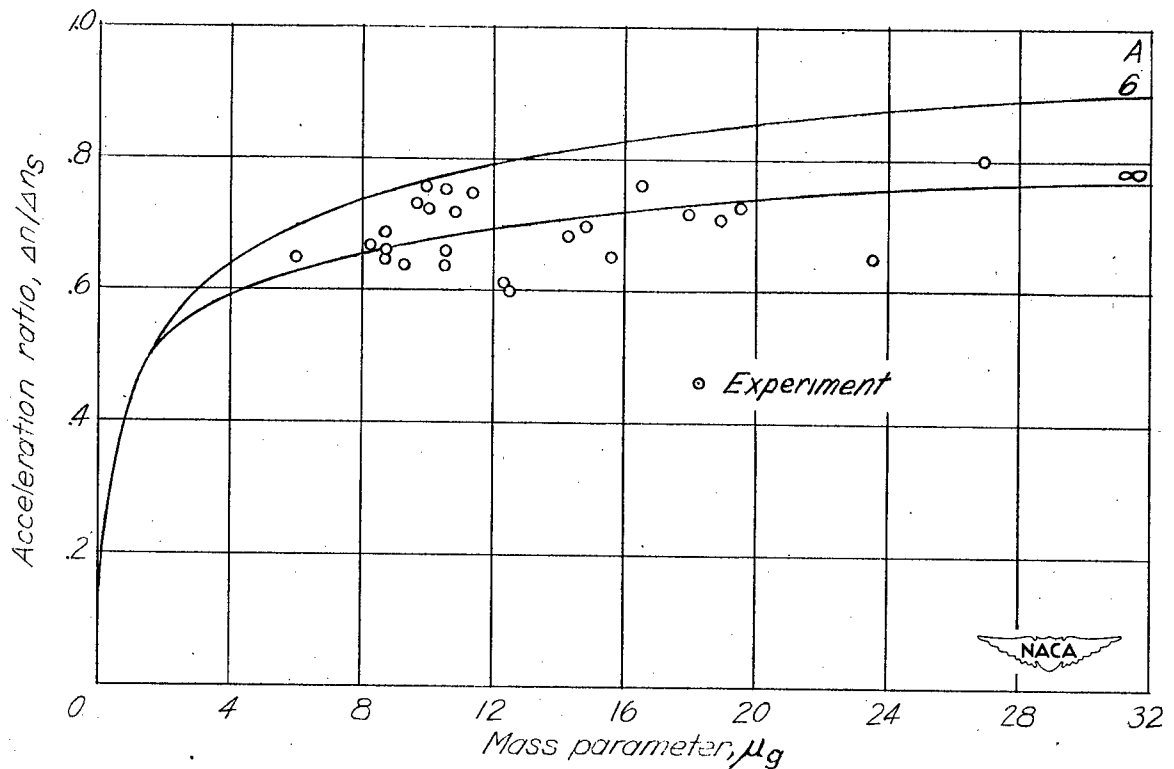
Figure 28.— Comparison of calculated and experimental acceleration ratios for a sharp-edge gust. Pitch assumed zero.
