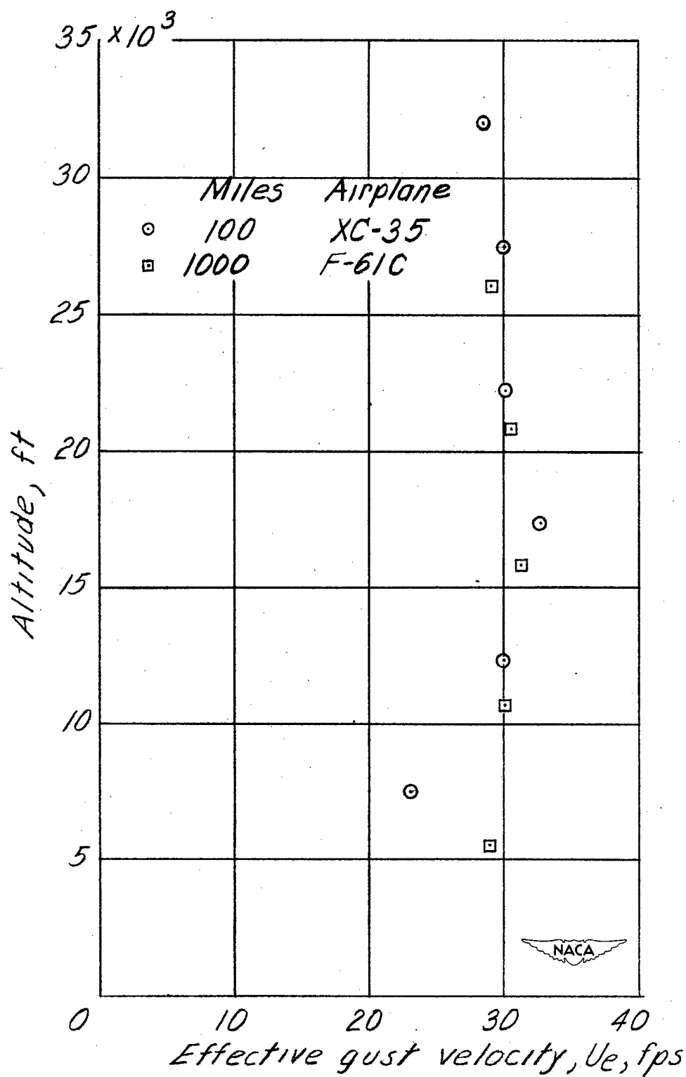
Figure 10.— Expected effective gust velocity at various altitudes within convective clouds for 100 and 1000 miles of flight from data for XC-35 and F-61C airplanes, respectively.
