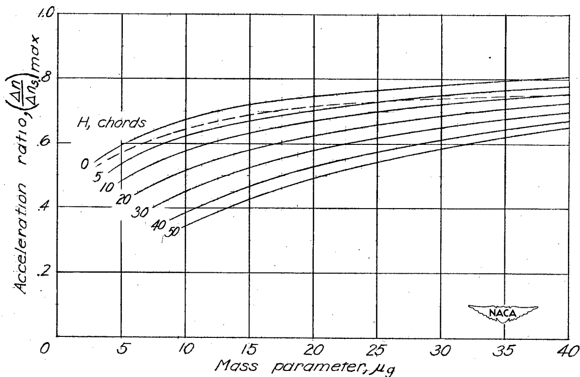
Figure 4.— Acceleration ratio as function of the mass parameter. Above dash line, finite gradient solution is not valid.
