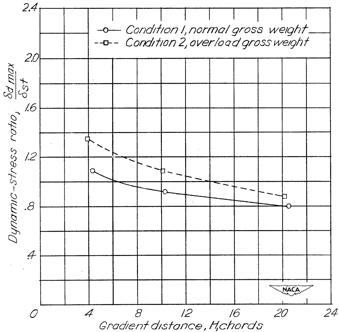
Figure 47.- Effect of change of wing frequency due to addition of mass Model D, conditions 1 and 2.
