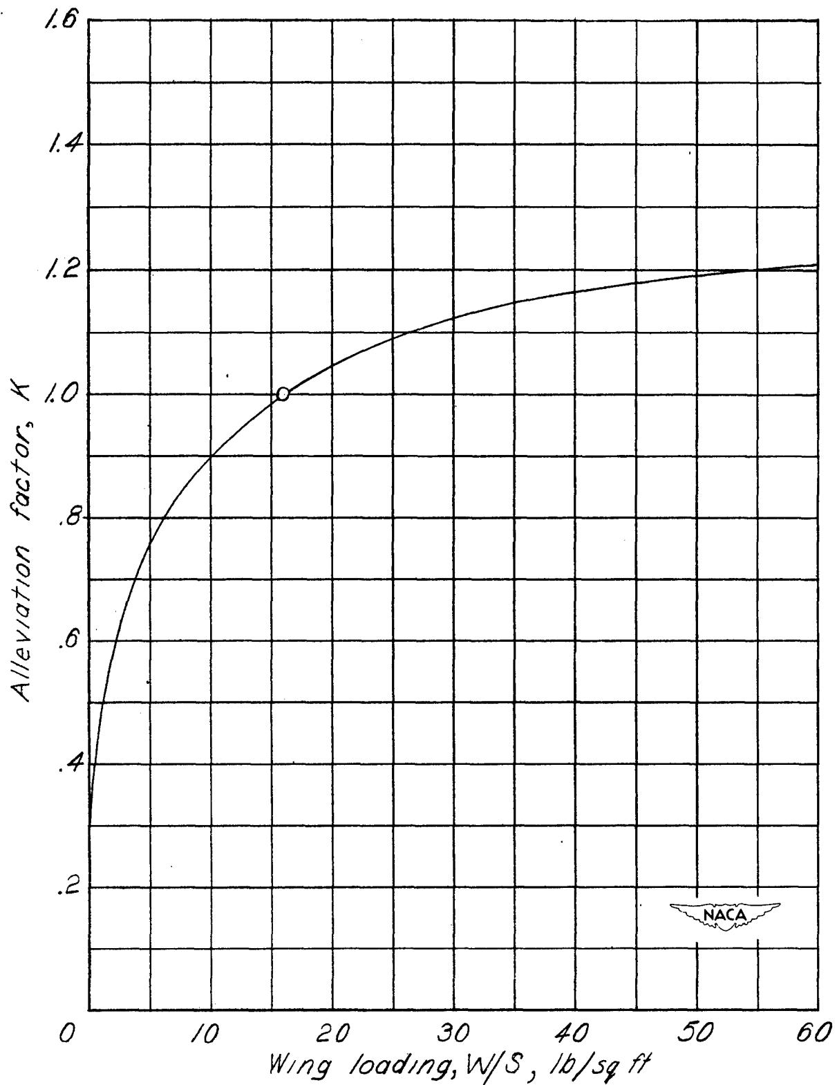
Figure 5.— Variation of alleviation factor with wing loading. From reference 1.
