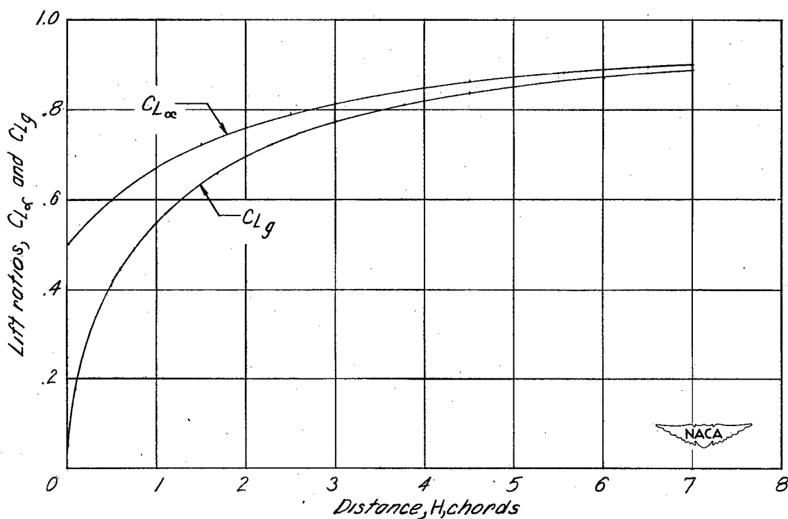
Figure 3.— Unsteady-lift functions for infinite aspect ratio. From reference 5.
