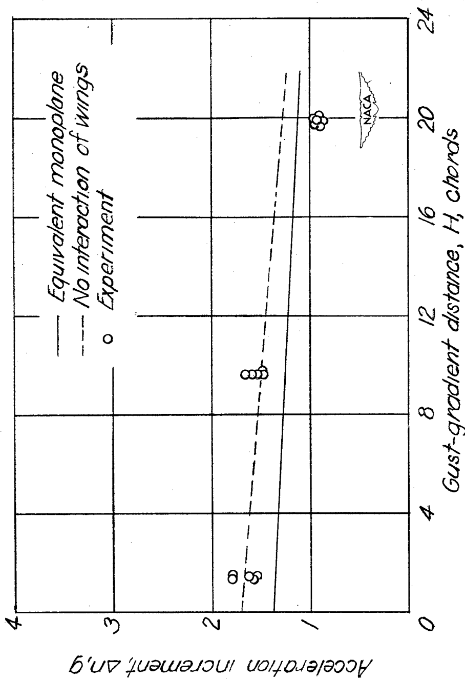
Figure 30.— Variation of acceleration with gust-gradient distance for a biplane. From reference 8.
