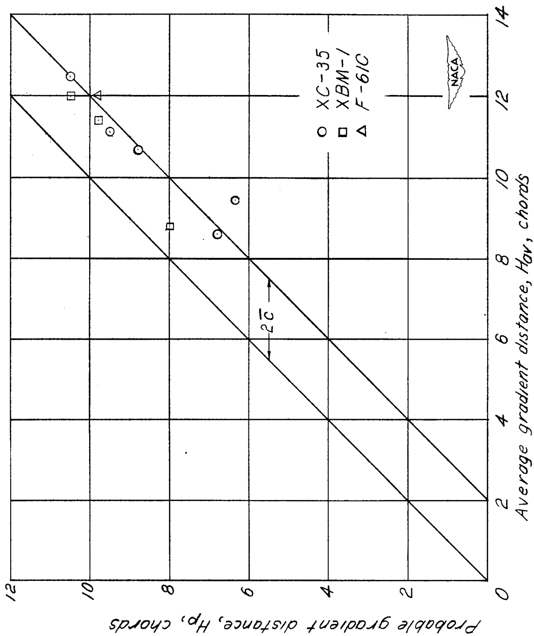
Figure 13.— Relation between the probable and average gust-gradient distance.
