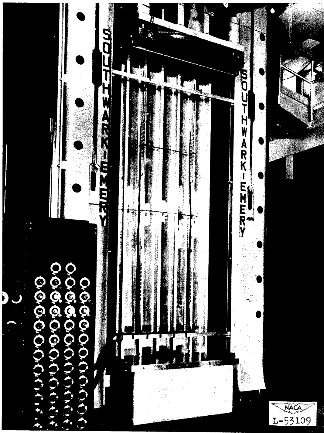
Figure 3.- End-fixity test.
