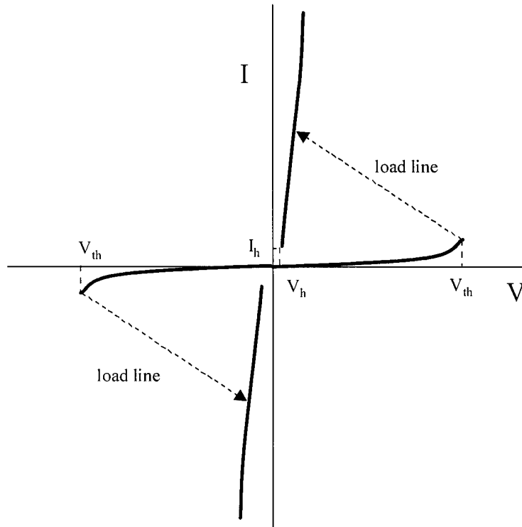
Figure 6. I-V Characteristic of a Threshold Switch [15]
