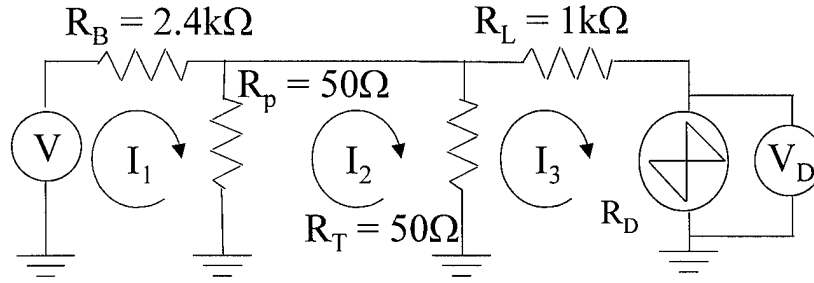
Figure 14. Equivalent characterization circuit
