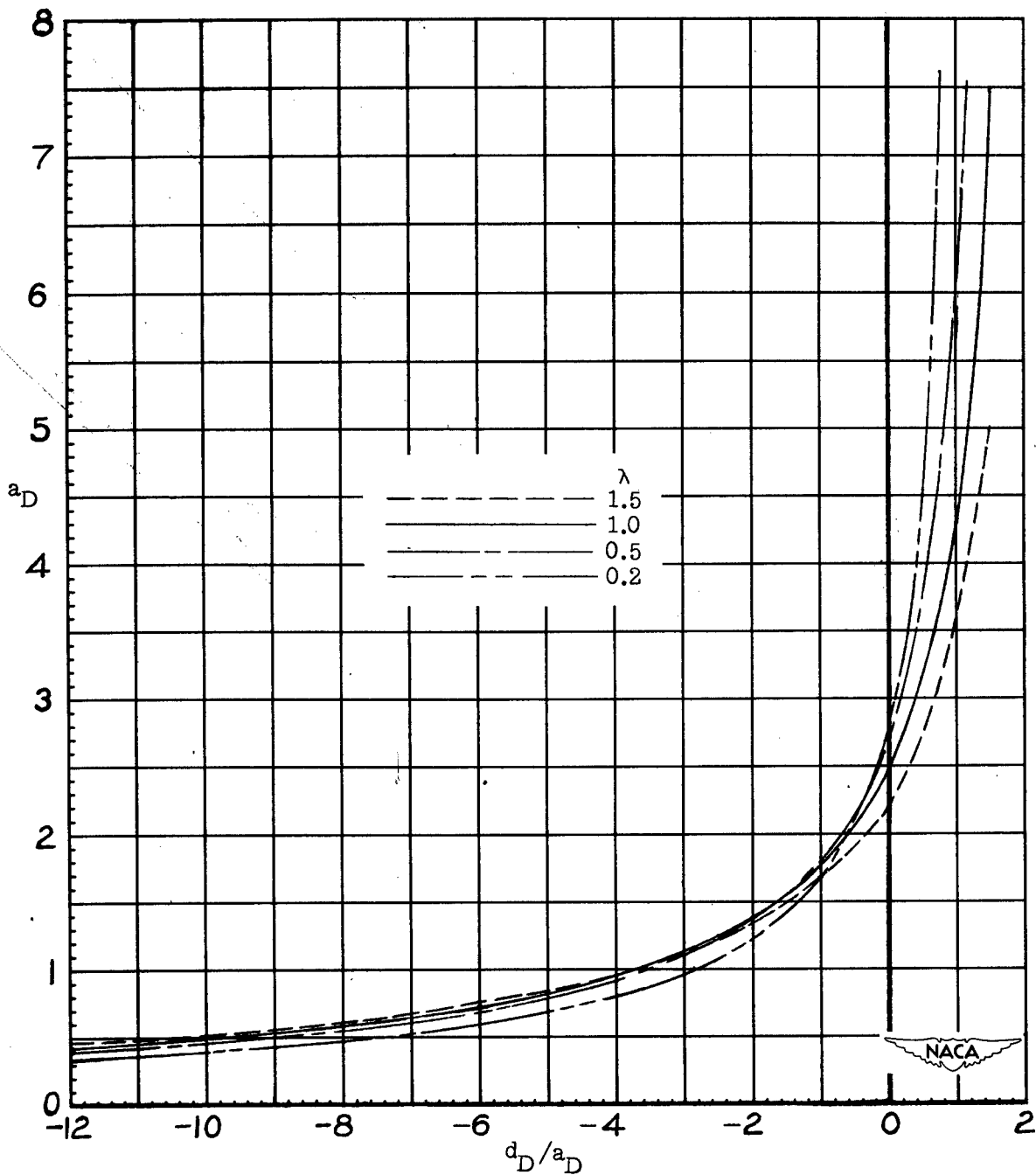
Figure 4.- Divergence of swept wings.
