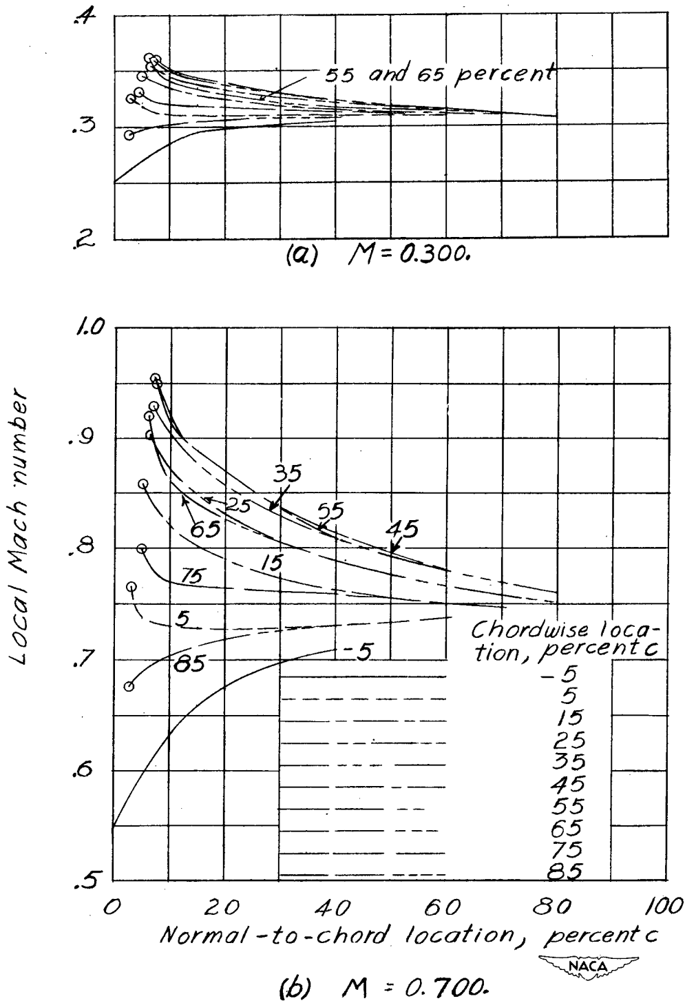
Figure 6.- Variation of local Mach number along lines perpendicular to chord and at various distances from leading edge. NACA 66,2-015; \alpha = 0^\circ
